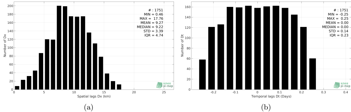
Figure 5: Histograms of the spatial (a) and temporal (b) lags between the time of the TSG-GOSUD-Research-vessel measurements and the date of the corresponding SMAP-L2-JPL-V4 SSS product.
