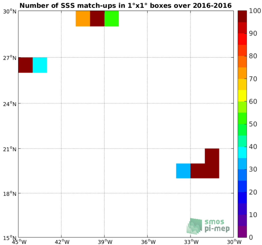
Figure 4: Number of SSS match-ups between TSG-GOSUD-Research-vessel SSS and the SMAP-L2-JPL-V4 SSS product for the SPURS 1 Pi-MEP region over 1°x1° boxes and for the full satellite product period.
