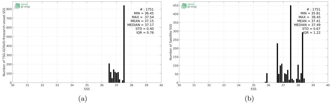
Figure 2: Histograms of SSS from TSG-GOSUD-Research-vessel (a) and SMAP-L2-JPL-V4 (b) considering all match-up pairs per bins of 0.1 over the SPURS 1 Pi-MEP region and for the full satellite product period.
