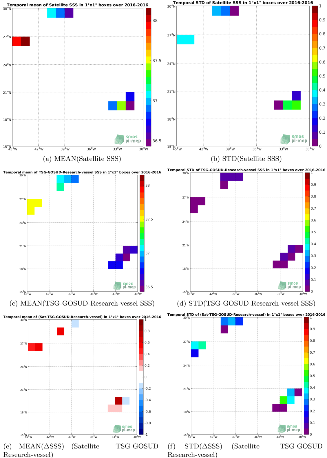
Figure 6: Temporal mean (left) and STD (right) of SSS from SMAP-L2-JPL-V4 (top), TSG-GOSUD-Research-vessel (middle), and of \Delta SSS 18 (Satellite - TSG-GOSUD-Research-vessel). Only match-up pairs are used to generate these maps.
