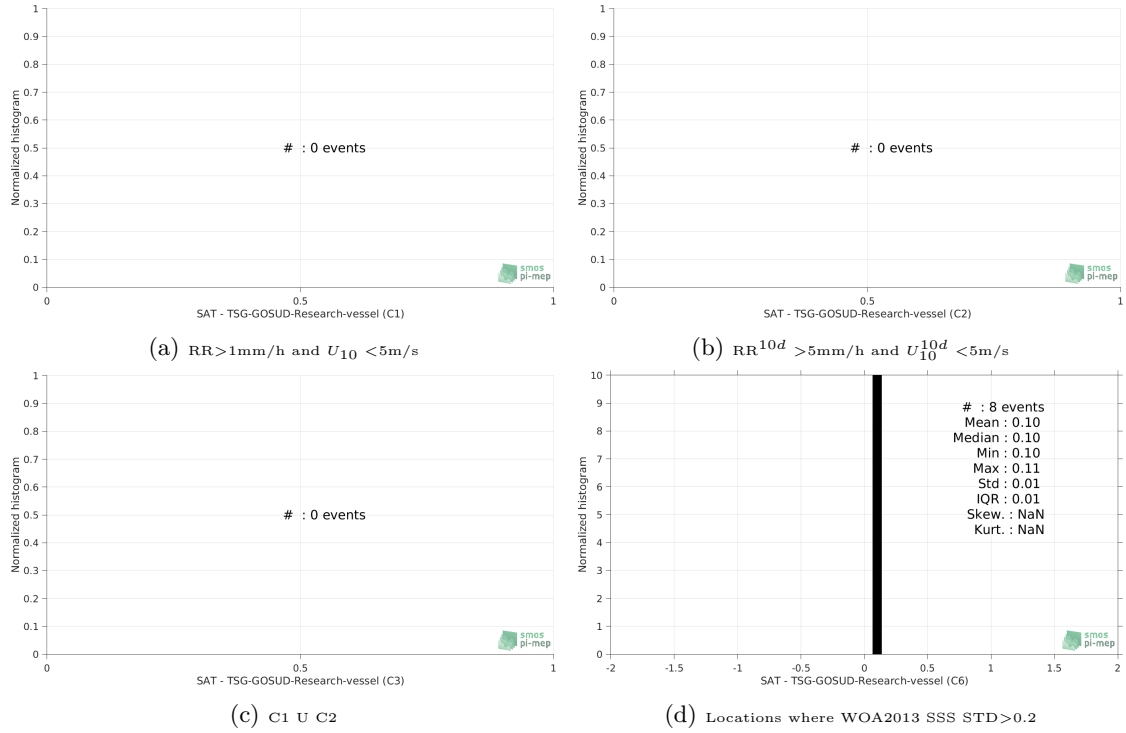
Figure 13: Normalized histogram of \Delta\text{SSS} (SMAP-L2-JPL-V4 - TSG-GOSUD-Research-vessel) for 6 different subdatasets corresponding to: RR > 1\text{mm/h} and U_{10} < 5\text{m/s} (a), RR^{10d} > 5\text{mm/h} and U_{10}^{10d} < 5\text{m/s} (b), C1 \cup C2 (c), Locations where WOA2013 SSS STD > 0.2 (d).
