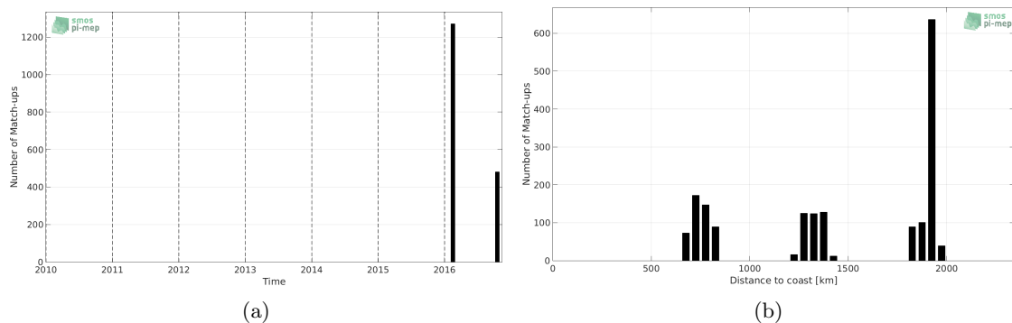
Figure 1: Number of match-ups between TSG-GOSUD-Research-vessel and SMAP-L2-JPL-V4 SSS as a function of time (a) and as function of the distance to coast (b) over the SPURS 1 Pi-MEP region and for the full satellite product period.
