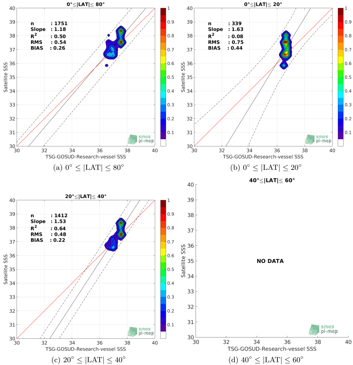
Figure 9: Contour maps of the concentration of SMAP-L2-JPL-V4 SSS (y-axis) versus TSG-GOSUD-Research-vessel SSS (x-axis) at match-up pairs for different latitude bands. For each plot, the red line shows x=y . The black thin and dashed lines indicate a linear fit through the data cloud and the \pm 95\% confidence levels, respectively. The number match-up pairs n , the slope and R^2 coefficient of the linear fit, the root mean square (RMS) and the mean bias between satellite and in situ data are indicated for each latitude band in each plots.
