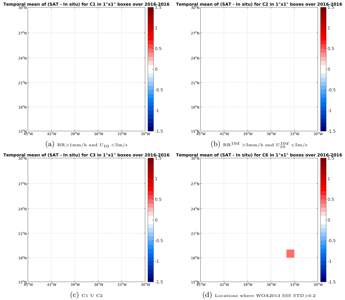
Figure 12: Temporal mean gridded over spatial boxes of size 1°x1° of \Delta SSS (SMAP-L2-JPL-V4 - TSG-GOSUD-Research-vessel) for 4 different subdatasets corresponding to: RR > 1mm/h and U 10 < 5m/s (a), RR 10d > 5mm/h and U 10 10d < 5m/s (b), C1 U C2 (c), Locations where WOA2013 SSS STD > 0.2 (d).
