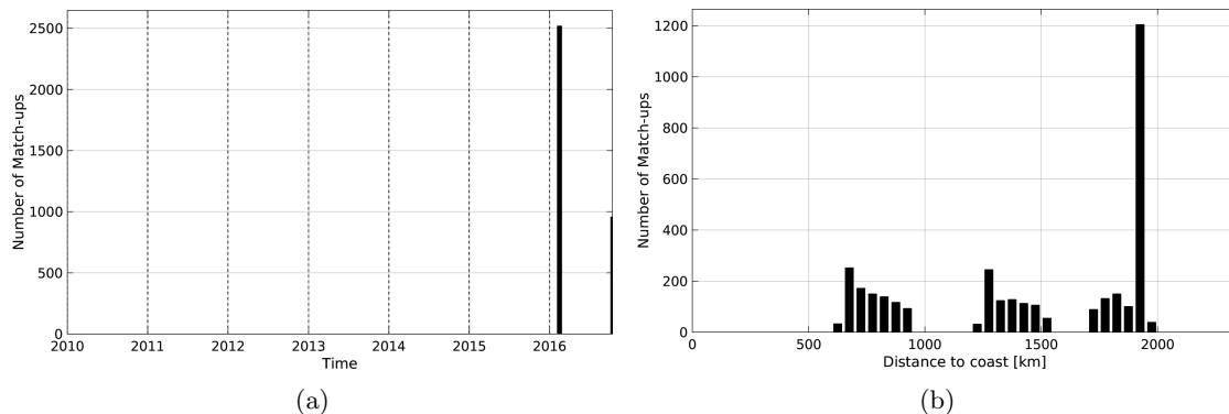
Figure 1: Number of match-ups between TSG-GOSUD-Research-vessel and SMAP-L2-JPL-V4 SSS as a function of time (a) and as function of the distance to coast (b) over the SPURS 1 Pi-MEP region and for the full satellite product period.
