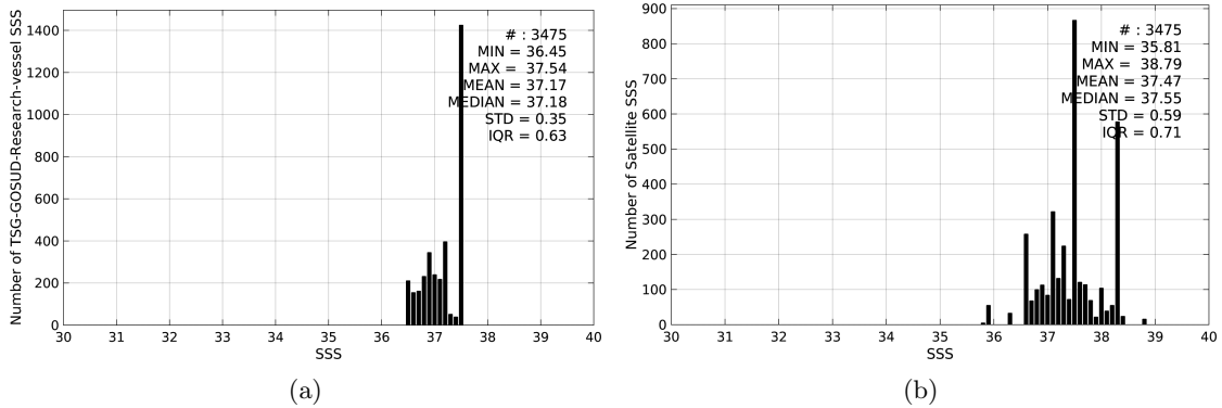
Figure 2: Histograms of SSS from TSG-GOSUD-Research-vessel (a) and SMAP-L2-JPL-V4 (b) considering all match-up pairs per bins of 0.1 over the SPURS 1 Pi-MEP region and for the full satellite product period.
