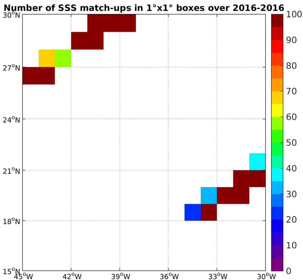
Figure 4: Number of SSS match-ups between TSG-GOSUD-Research-vessel SSS and the SMAP-L2-JPL-V4 SSS product for the SPURS 1 Pi-MEP region over 1°x1° boxes and for the full satellite product period.
