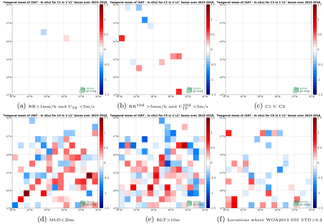
Figure 12: Temporal mean gridded over spatial boxes of size 1^\circ \times 1^\circ of \Delta\text{SSS} (SMAP-L2-JPL-V4 - Argo) for 6 different subdatasets corresponding to: \text{RR} > 1\text{mm/h} and U_{10} < 5\text{m/s} (a), \text{RR}^{10d} > 5\text{mm/h} and U_{10}^{10d} < 5\text{m/s} (b), C1 U C2 (c), \text{MLD} < 20\text{m} (d), \text{BLT} > 10\text{m} (e), Locations where WOA2013 SSS STD > 0.2 (f).
