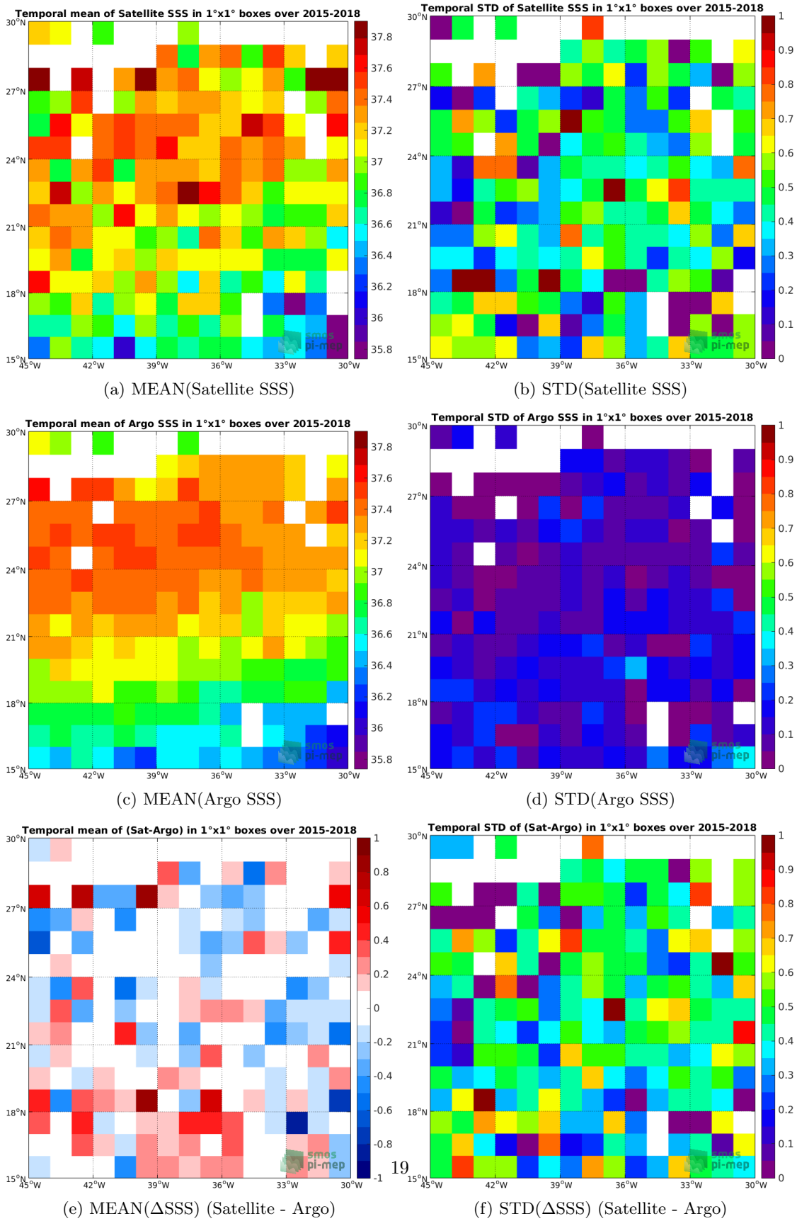
Figure 6: Temporal mean (left) and STD (right) of SSS from SMAP-L2-JPL-V4 (top), Argo (middle), and of \Delta SSS (Satellite - Argo). Only match-up pairs are used to generate these maps.
