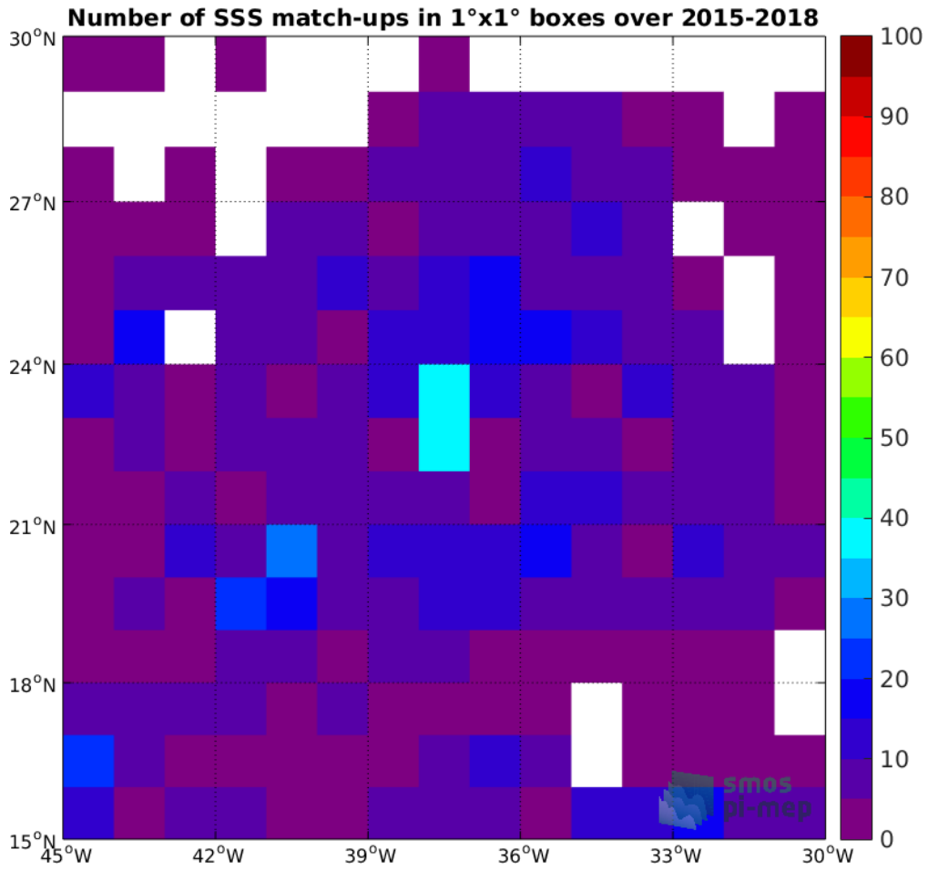
Figure 4: Number of SSS match-ups between Argo SSS and the SMAP-L2-JPL-V4 SSS product for the SPURS 1 Pi-MEP region over 1°x1° boxes and for the full satellite product period.
