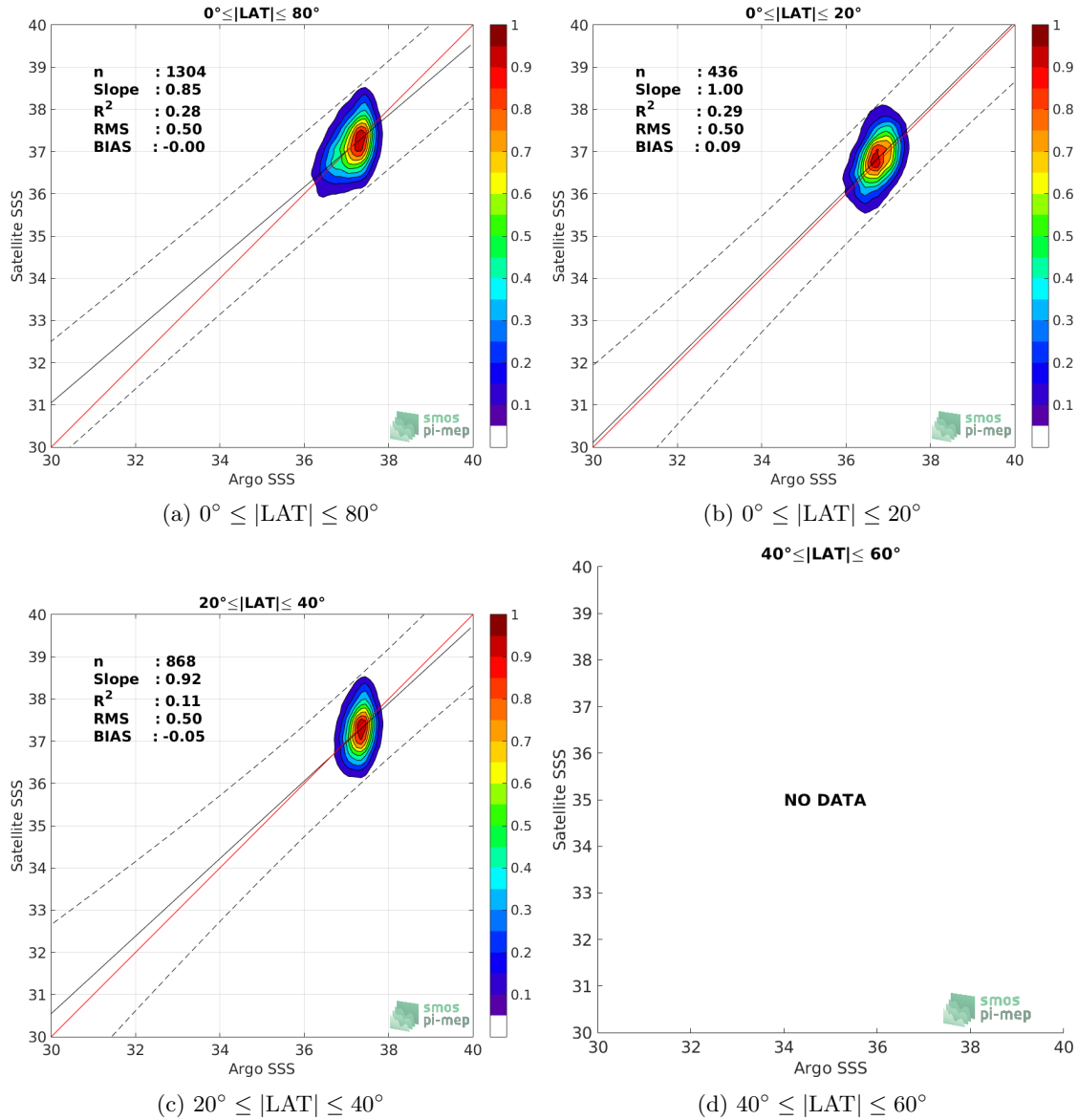
Figure 9: Contour maps of the concentration of SMAP-L2-JPL-V4 SSS (y-axis) versus Argo SSS (x-axis) at match-up pairs for different latitude bands. For each plot, the red line shows x=y . The black thin and dashed lines indicate a linear fit through the data cloud and the \pm 95\% confidence levels, respectively. The number match-up pairs n , the slope and R^2 coefficient of the linear fit, the root mean square (RMS) and the mean bias between satellite and in situ data are indicated for each latitude band in each plots.
