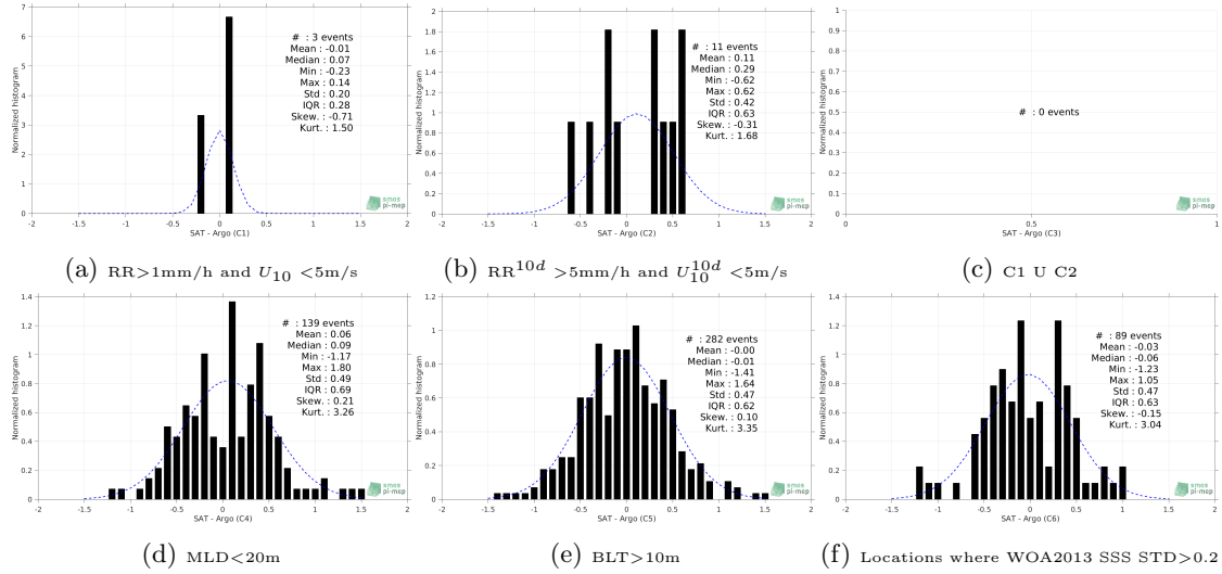
Figure 13: Normalized histogram of \Delta SSS (SMAP-L2-JPL-V4 - Argo) for 6 different subdatasets corresponding to: RR>1mm/h and U_{10} < 5\text{m/s} (a), RR^{10d} > 5\text{mm/h} and U_{10}^{10d} < 5\text{m/s} (b), C1 U C2 (c),MLD<20m (d),BLT>10m (e),Locations where WOA2013 SSS STD>0.2 (f).
