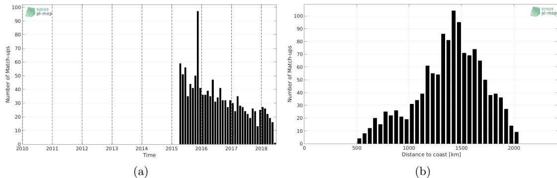
Figure 1: Number of match-ups between Argo and SMAP-L2-JPL-V4 SSS as a function of time (a) and as function of the distance to coast (b) over the SPURS 1 Pi-MEP region and for the full satellite product period.
