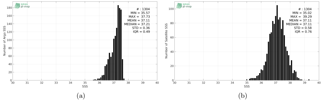
Figure 2: Histograms of SSS from Argo (a) and SMAP-L2-JPL-V4 (b) considering all match-up pairs per bins of 0.1 over the SPURS 1 Pi-MEP region and for the full satellite product period.
