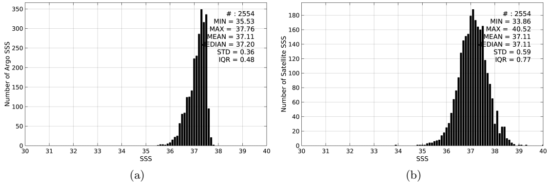
Figure 2: Histograms of SSS from Argo (a) and SMAP-L2-JPL-V4 (b) considering all match-up pairs per bins of 0.1 over the SPURS 1 Pi-MEP region and for the full satellite product period.
