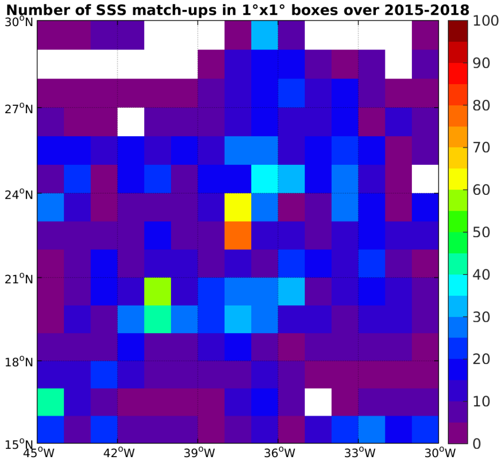
Figure 4: Number of SSS match-ups between Argo SSS and the SMAP-L2-JPL-V4 SSS product for the SPURS 1 Pi-MEP region over 1°x1° boxes and for the full satellite product period.
