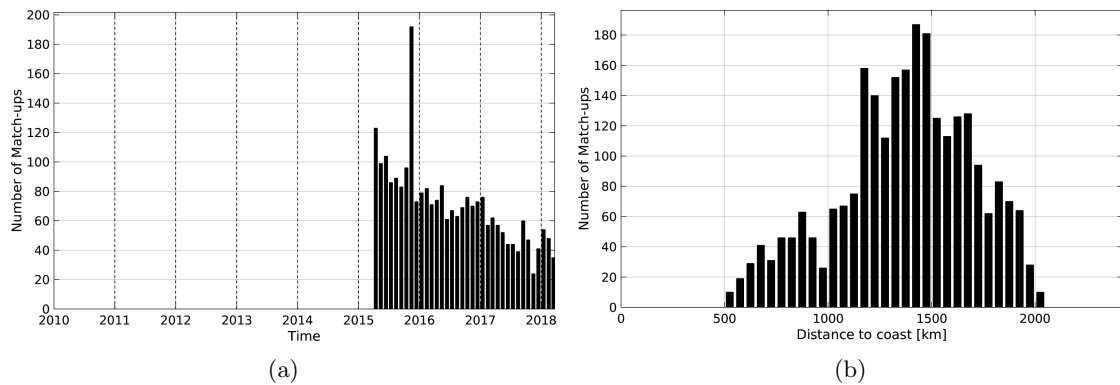
Figure 1: Number of match-ups between Argo and SMAP-L2-JPL-V4 SSS as a function of time (a) and as function of the distance to coast (b) over the SPURS 1 Pi-MEP region and for the full satellite product period.
