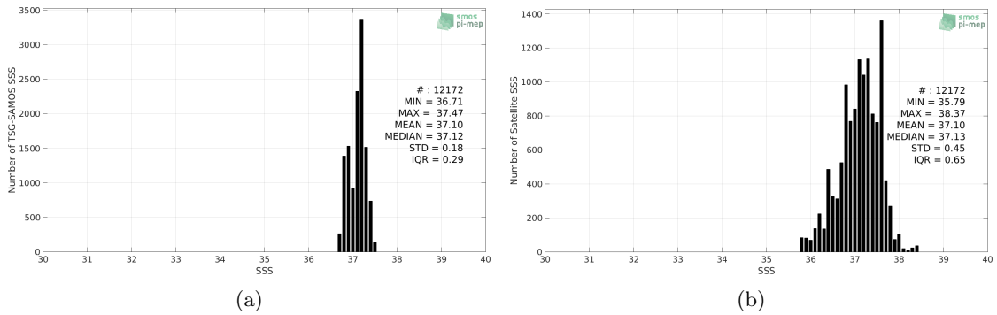
Figure 2: Histograms of SSS from TSG-SAMOS (a) and SMAP-L2-JPL-V4.3 (b) considering all match-up pairs per bins of 0.1 over the SPURS 1 Pi-MEP region and for the full satellite product period.
