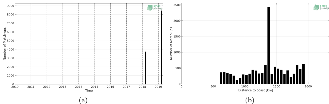
Figure 1: Number of match-ups between TSG-SAMOS and SMAP-L2-JPL-V4.3 SSS as a function of time (a) and as function of the distance to coast (b) over the SPURS 1 Pi-MEP region and for the full satellite product period.
