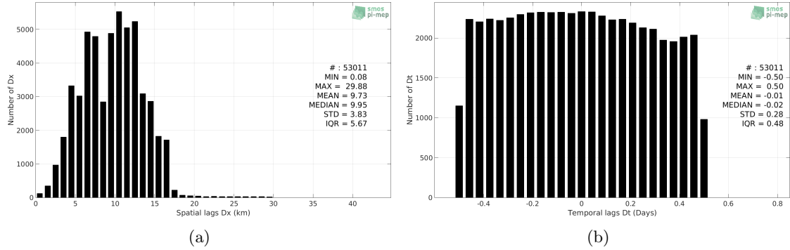
Figure 5: Histograms of the spatial (a) and temporal (b) lags between the time of the TSG-GOSUD-Research-vessel measurements and the date of the corresponding SMAP-L2-JPL-V4.3 SSS product.
