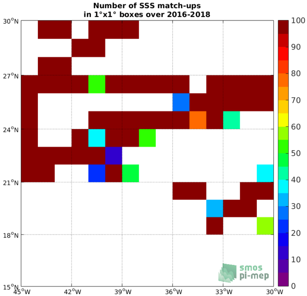
Figure 4: Number of SSS match-ups between TSG-GOSUD-Research-vessel SSS and the SMAP-L2-JPL-V4.3 SSS product for the SPURS 1 Pi-MEP region over 1°x1° boxes and for the full satellite product period.
