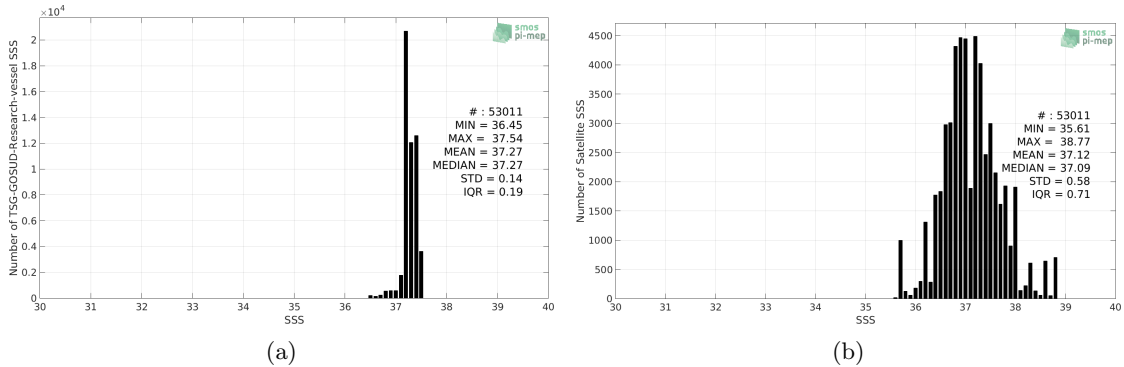
Figure 2: Histograms of SSS from TSG-GOSUD-Research-vessel (a) and SMAP-L2-JPL-V4.3 (b) considering all match-up pairs per bins of 0.1 over the SPURS 1 Pi-MEP region and for the full satellite product period.
