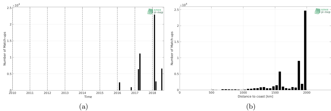
Figure 1: Number of match-ups between TSG-GOSUD-Research-vessel and SMAP-L2-JPL-V4.3 SSS as a function of time (a) and as function of the distance to coast (b) over the SPURS 1 Pi-MEP region and for the full satellite product period.
