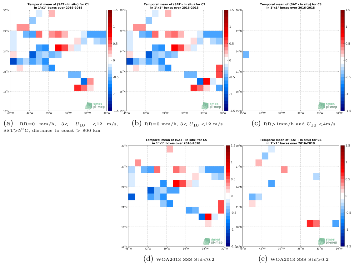
Figure 12: Temporal mean gridded over spatial boxes of size 1^\circ \times 1^\circ of \Delta SSS (SMAP-L2-JPL-V4.3 - TSG-GOSUD-Research-vessel) for 5 different subdatasets corresponding to: RR=0 mm/h, 3 < U_{10} < 12 m/s, SST > 5^\circ C , distance to coast > 800 km (a), RR=0 mm/h, 3 < U_{10} < 12 m/s (b), RR > 1 mm/h and U_{10} < 4 m/s (c), WOA2013 SSS Std < 0.2 (d), WOA2013 SSS Std > 0.2 (e).
