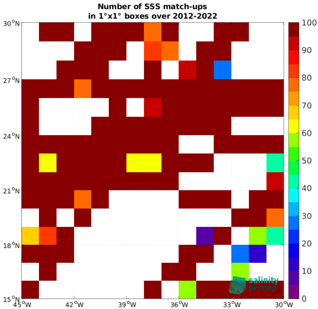
Figure 5: Number of SSS match-ups between TSG (GOSUD-Research-vessel) SSS and the ISAS v7 - Monthly (Ifremer-LOPS-CMEMS) SSS product for the SPURS 1 Pi-MEP region over 1°x1° boxes and for the full satellite product period.
