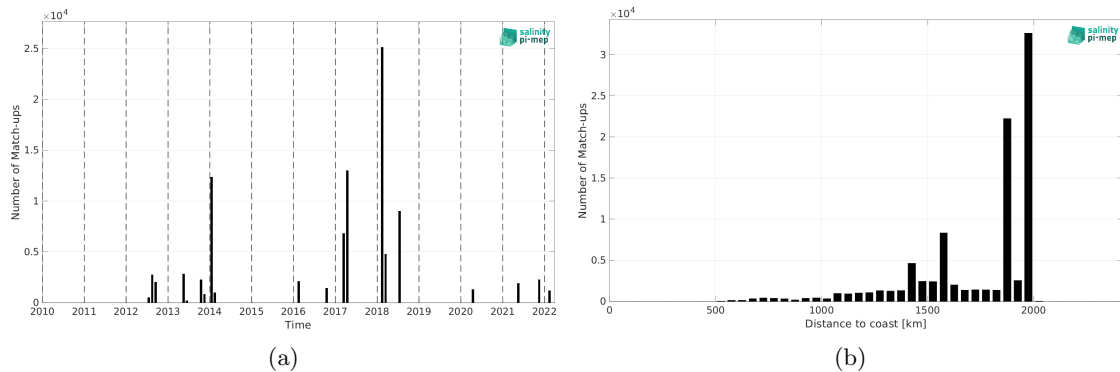
Figure 2: Number of match-ups between TSG (GOSUD-Research-vessel) and ISAS v7 - Monthly (Ifremer-LOPS-CMEMS) SSS as a function of time (a) and as function of the distance to coast (b) over the SPURS 1 Pi-MEP region and for the full satellite product period.
