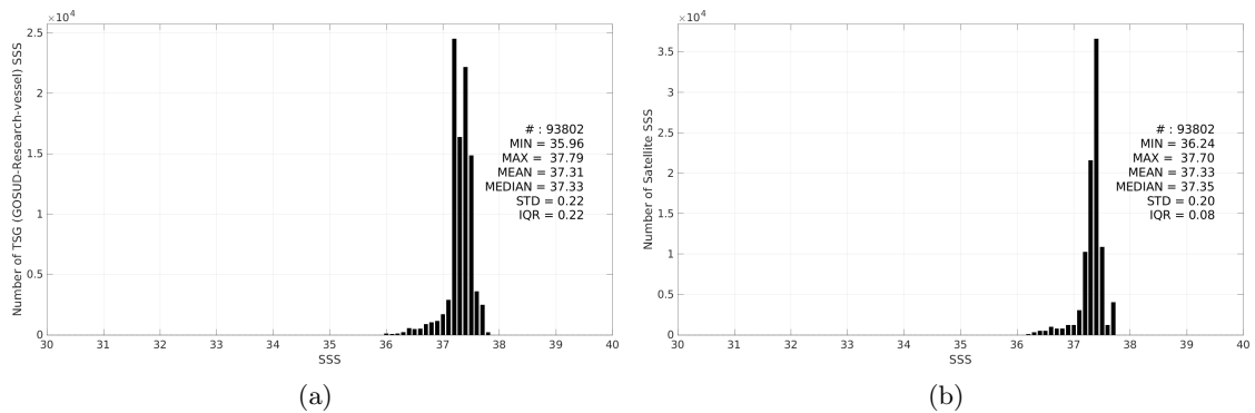
Figure 3: Histograms of SSS from TSG (GOSUD-Research-vessel) (a) and ISAS v7 - Monthly (Ifremer-LOPS-CMEMS) (b) considering all match-up pairs per bins of 0.1 over the SPURS 1 Pi-MEP region and for the full satellite product period.
