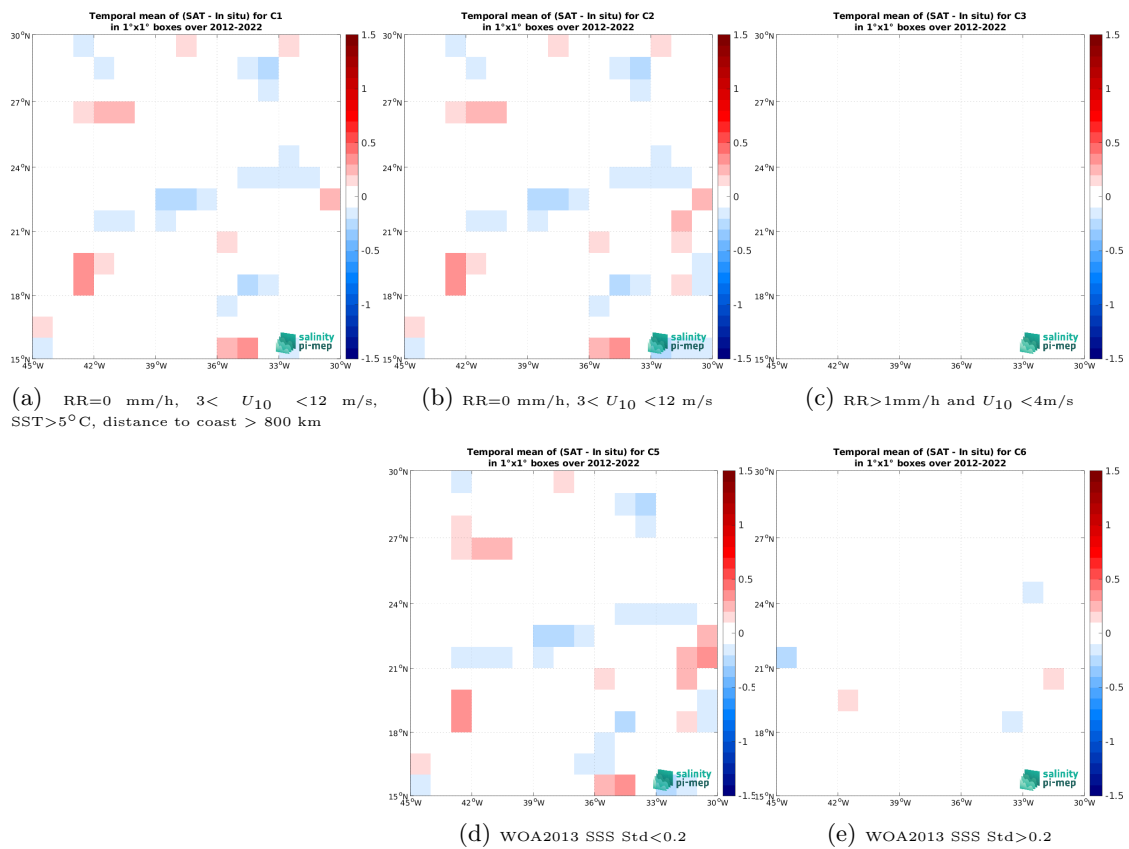
Figure 14: Temporal mean gridded over spatial boxes of size 1^\circ \times 1^\circ of \Delta SSS (ISAS v7 - Monthly (Ifremer-LOPS-CMEMS) - TSG (GOSUD-Research-vessel)) for 5 different subdatasets corresponding to: RR=0 mm/h, 3 < U_{10} < 12 m/s, SST > 5^\circ C , distance to coast > 800 km (a), RR=0 mm/h, 3 < U_{10} < 12 m/s (b), RR > 1 mm/h and U_{10} < 4 m/s (c), WOA2013 SSS Std < 0.2 (d), WOA2013 SSS Std > 0.2 (e).
