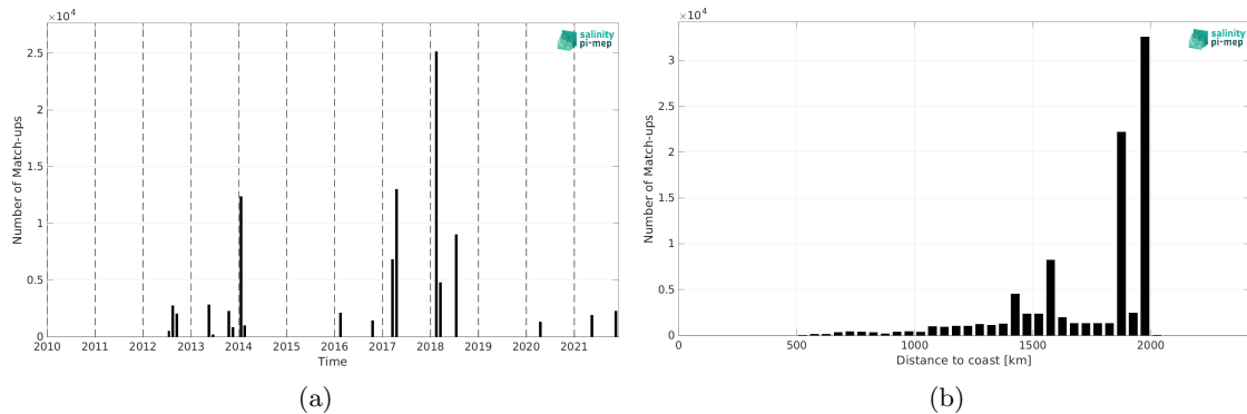
Figure 2: Number of match-ups between TSG (GOSUD-Research-vessel) and ISAS SSS as a function of time (a) and as function of the distance to coast (b) over the SPURS 1 Pi-MEP region and for the full satellite product period.
