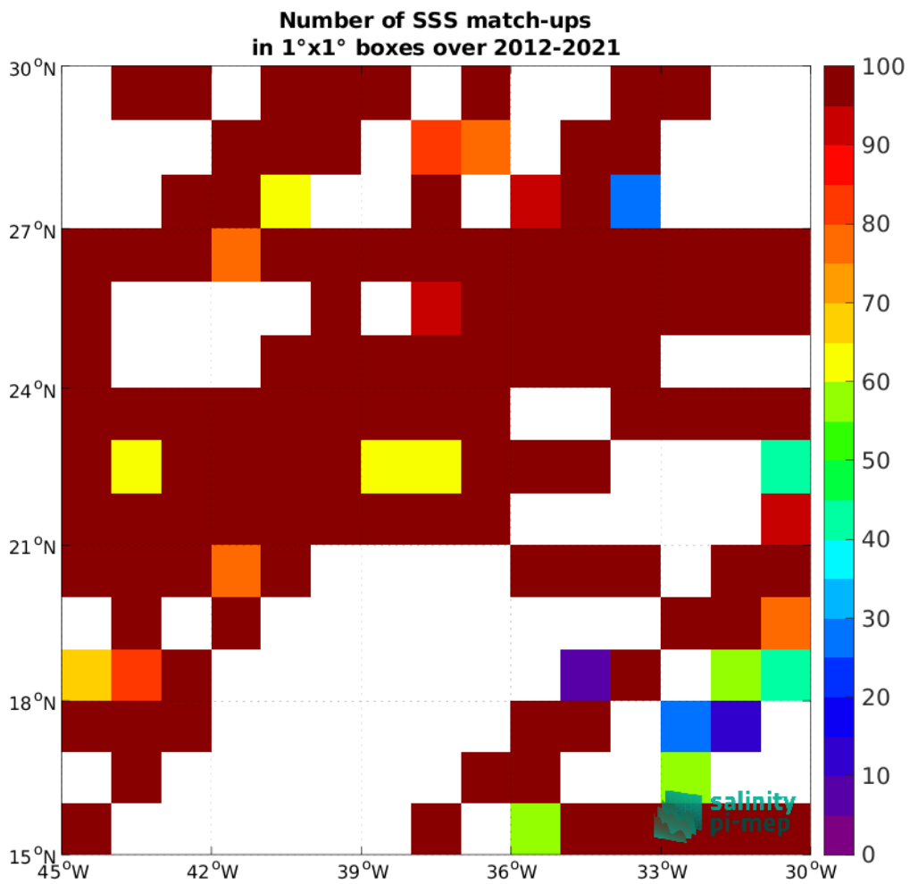
Figure 5: Number of SSS match-ups between TSG (GOSUD-Research-vessel) SSS and the ISAS SSS product for the SPURS 1 Pi-MEP region over 1°×1° boxes and for the full satellite product period.
