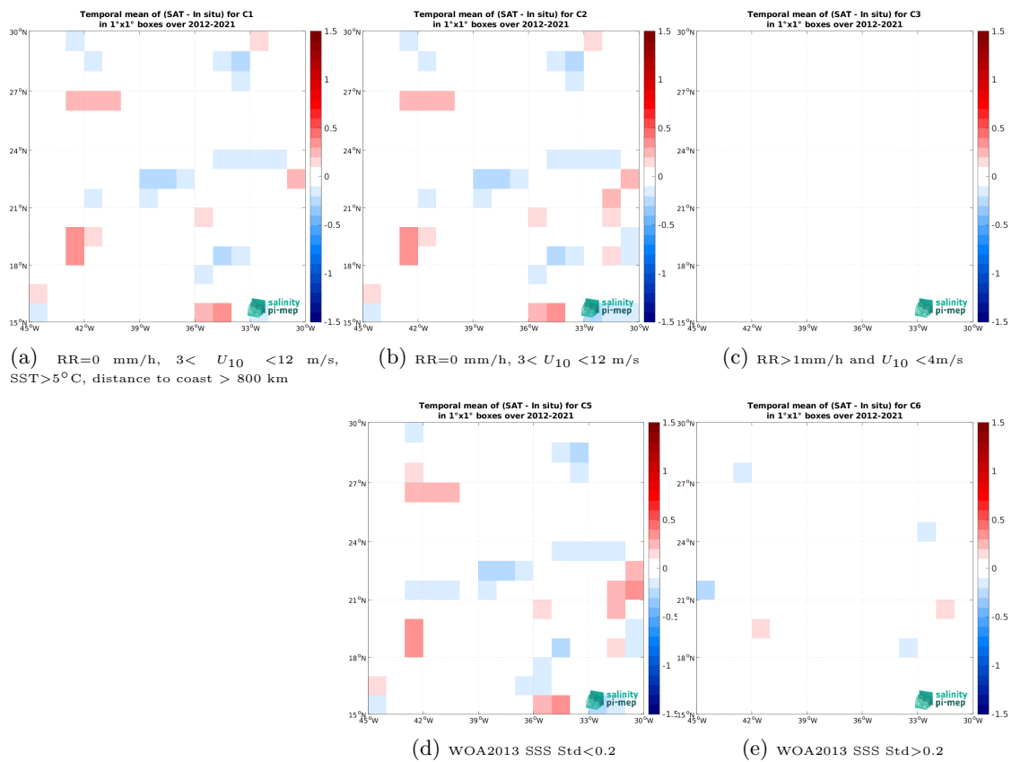
Figure 14: Temporal mean gridded over spatial boxes of size 1^\circ \times 1^\circ of \Delta SSS (ISAS - TSG (GOSUD-Research-vessel)) for 5 different subdatasets corresponding to:RR=0 mm/h, 3 < U_{10} < 12 m/s, SST>5°C, distance to coast > 800 km (a), RR=0 mm/h, 3 < U_{10} < 12 m/s (b), RR>1mm/h and U_{10} < 4 m/s (c), WOA2013 SSS Std<0.2 (d), WOA2013 SSS Std>0.2 (e).
