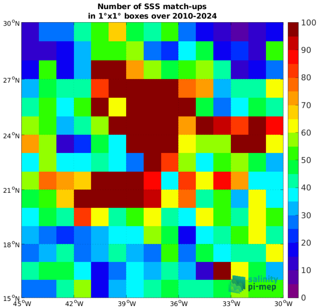
Figure 5: Number of SSS match-ups between Argo SSS and the ISAS SSS product for the SPURS 1 Pi-MEP region over 1°×1° boxes and for the full satellite product period.
