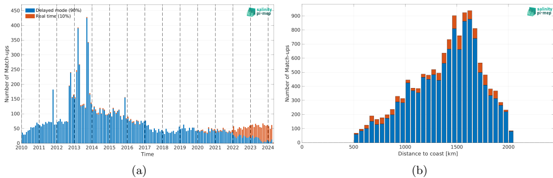
Figure 2: Number of match-ups between Argo and ISAS SSS as a function of time (a) and as function of the distance to coast (b) over the SPURS 1 Pi-MEP region and for the full satellite product period.
