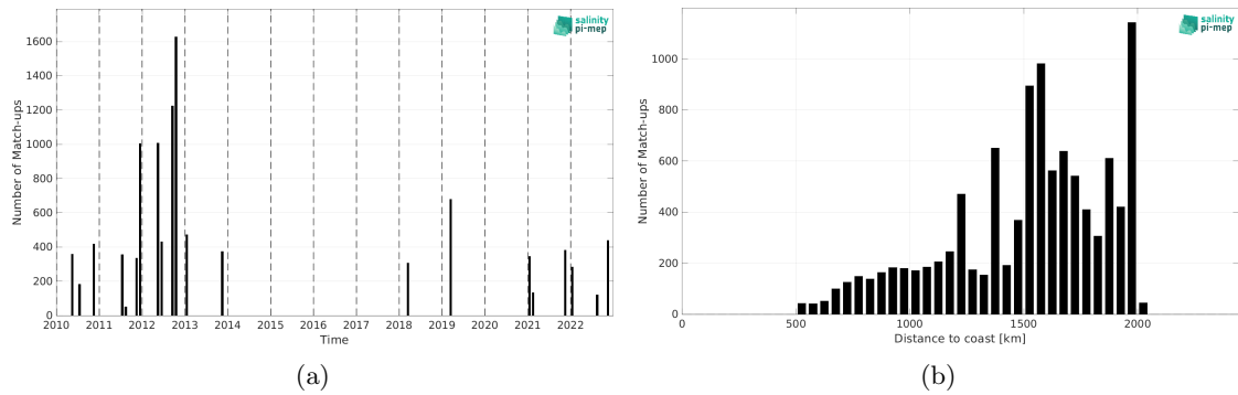
Figure 2: Number of match-ups between TSG (SAMOS) and CCI SSS L4 Merged-OI v5.5 - 7-day running (ESA) SSS as a function of time (a) and as function of the distance to coast (b) over the SPURS 1 Pi-MEP region and for the full satellite product period.
