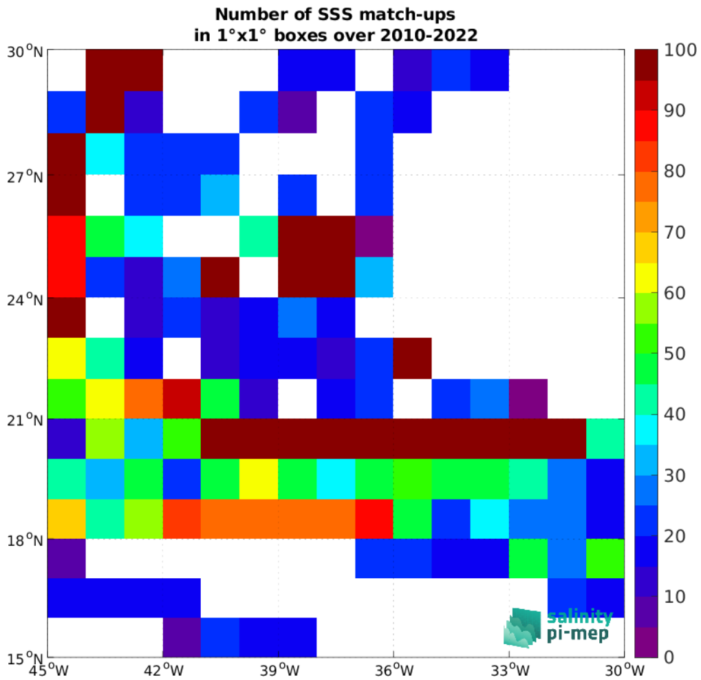
Figure 5: Number of SSS match-ups between TSG (SAMOS) SSS and the CCI SSS L4 Merged-OI v5.5 - 7-day running (ESA) SSS product for the SPURS 1 Pi-MEP region over 1°x1° boxes and for the full satellite product period.
