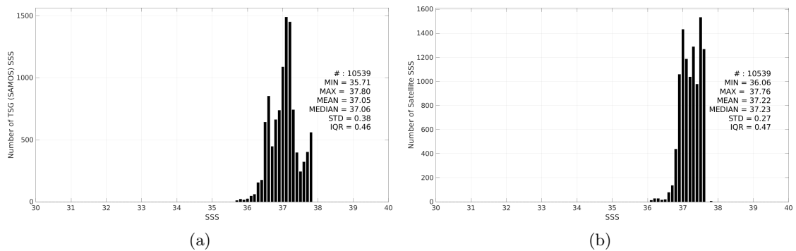
Figure 3: Histograms of SSS from TSG (SAMOS) (a) and CCI SSS L4 Merged-OI v5.5 - 7-day running (ESA) (b) considering all match-up pairs per bins of 0.1 over the SPURS 1 Pi-MEP region and for the full satellite product period.
