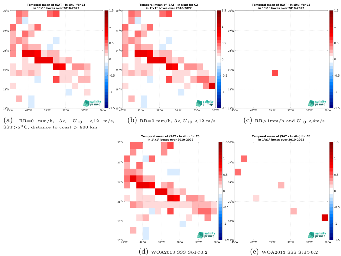
Figure 14: Temporal mean gridded over spatial boxes of size 1^\circ \times 1^\circ of \Delta SSS (CCI SSS L4 Merged-OI v5.5 - 7-day running (ESA) - TSG (SAMOS)) for 5 different subdatasets corresponding to:RR=0 mm/h, 3 < U_{10} < 12 m/s, SST >5^\circ C, distance to coast > 800 km (a), RR=0 mm/h, 3 < U_{10} < 12 m/s (b), RR >1 mm/h and U_{10} < 4 m/s (c), WOA2013 SSS Std <0.2 (d), WOA2013 SSS Std >0.2 (e).
