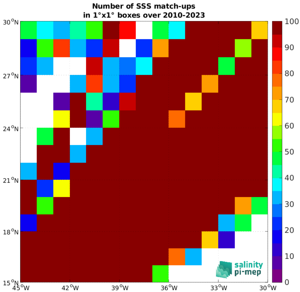
Figure 5: Number of SSS match-ups between TSG (LEGOS-DM) SSS and the CCI SSS L4 Merged-OI v5.5 - 7-day running (ESA) SSS product for the SPURS 1 Pi-MEP region over 1°x1° boxes and for the full satellite product period.
