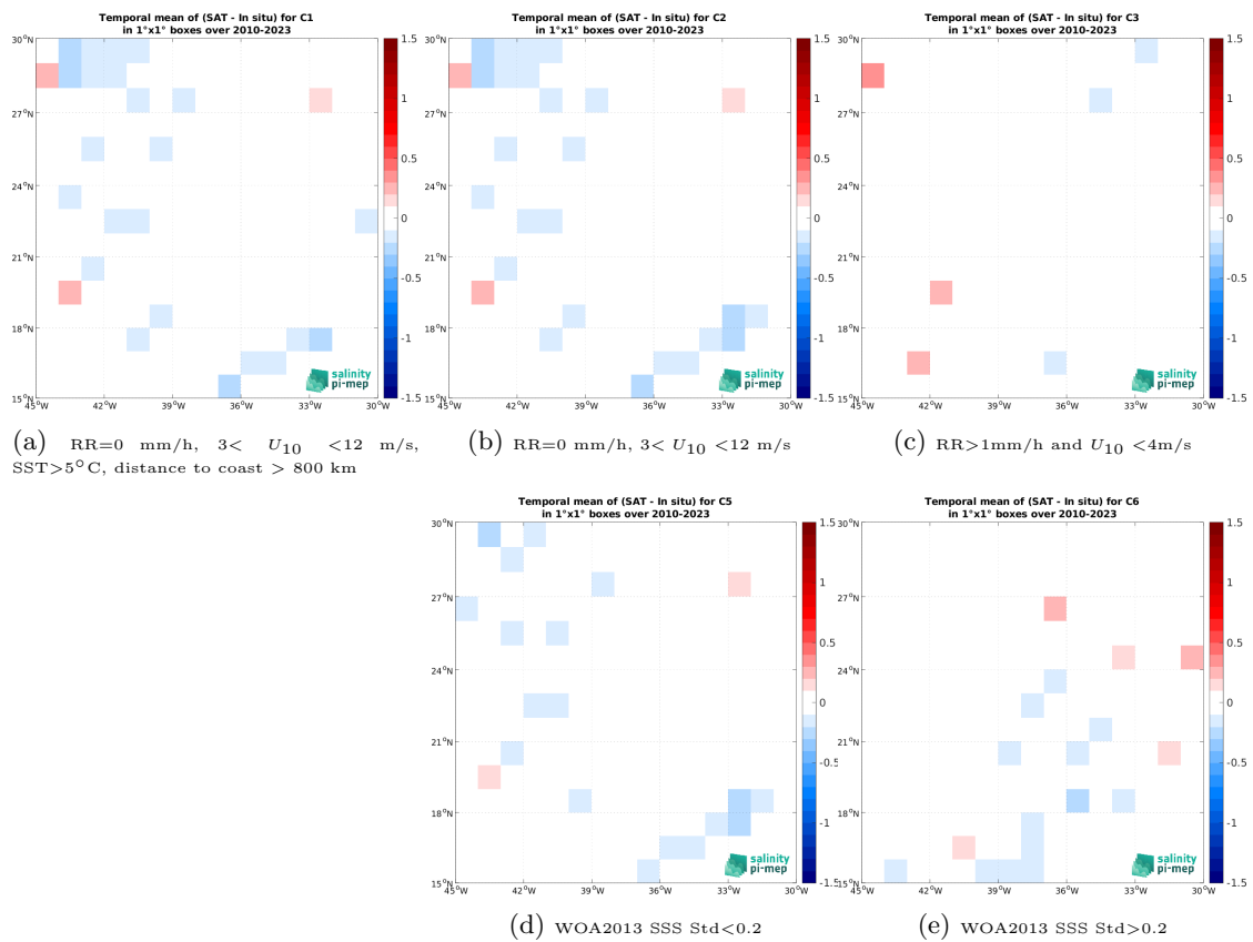
Figure 14: Temporal mean gridded over spatial boxes of size 1^\circ \times 1^\circ of \Delta\text{SSS} (CCI SSS L4 Merged-OI v5.5 - 7-day running (ESA) - TSG (LEGOS-DM)) for 5 different subdatasets corresponding to: \text{RR}=0 mm/h, 3 < U_{10} < 12 m/s, \text{SST} > 5^\circ\text{C} , distance to coast > 800 km (a), \text{RR}=0 mm/h, 3 < U_{10} < 12 m/s (b), \text{RR} > 1 mm/h and U_{10} < 4 m/s (c), WOA2013 SSS Std < 0.2 (d), WOA2013 SSS Std > 0.2 (e).
