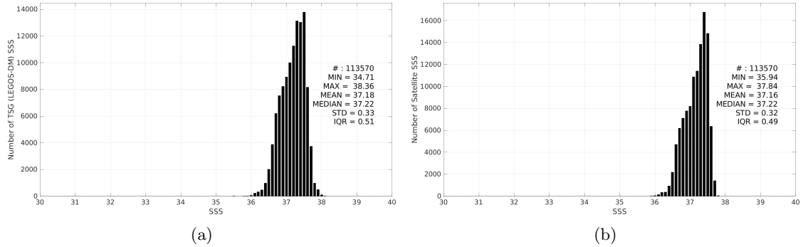
Figure 3: Histograms of SSS from TSG (LEGOS-DM) (a) and CCI SSS L4 Merged-OI v5.5 - 7-day running (ESA) (b) considering all match-up pairs per bins of 0.1 over the SPURS 1 Pi-MEP region and for the full satellite product period.
