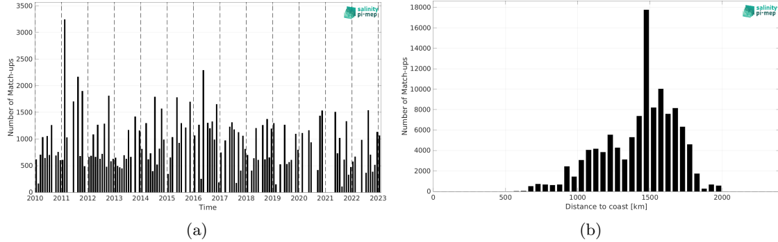
Figure 2: Number of match-ups between TSG (LEGOS-DM) and CCI SSS L4 Merged-OI v5.5 - 7-day running (ESA) SSS as a function of time (a) and as function of the distance to coast (b) over the SPURS 1 Pi-MEP region and for the full satellite product period.
