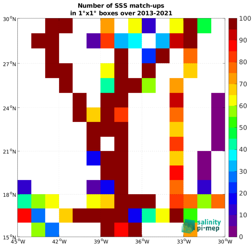
Figure 5: Number of SSS match-ups between TSG (GOSUD-Sailing-ship) SSS and the CCI SSS L4 Merged-OI v5.5 - 7-day running (ESA) SSS product for the SPURS 1 Pi-MEP region over 1^\circ \times 1^\circ boxes and for the full satellite product period.
