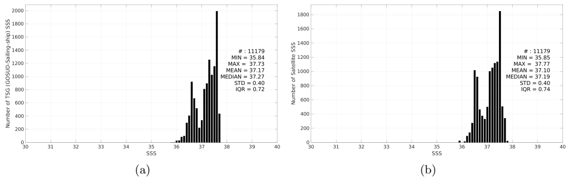
Figure 3: Histograms of SSS from TSG (GOSUD-Sailing-ship) (a) and CCI SSS L4 Merged-OI v5.5 - 7-day running (ESA) (b) considering all match-up pairs per bins of 0.1 over the SPURS 1 Pi-MEP region and for the full satellite product period.
