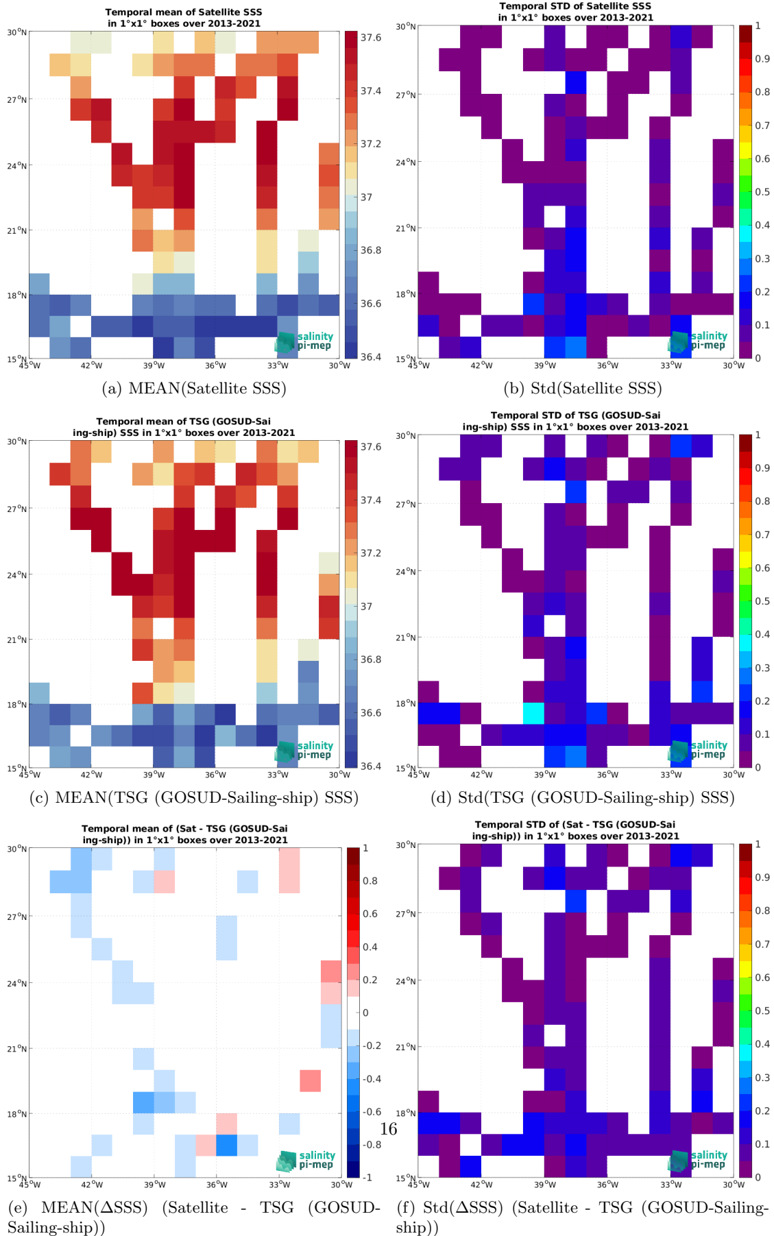
Figure 7: Temporal mean (left) and Std (right) of SSS from CCI SSS L4 Merged-OI v5.5 - 7-day running (ESA) (top), TSG (GOSUD-Sailing-ship) (middle), and of \Delta SSS (Satellite - TSG (GOSUD-Sailing-ship)). Only match-up pairs are used to generate these maps.
