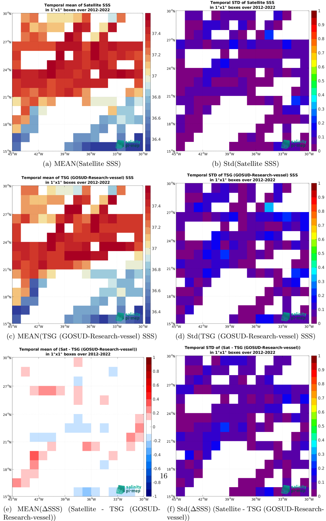
Figure 7: Temporal mean (left) and Std (right) of SSS from CCI SSS L4 Merged-OI v5.5 - 7-day running (ESA) (top), TSG (GOSUD-Research-vessel) (middle), and of \Delta SSS (Satellite - TSG (GOSUD-Research-vessel)). Only match-up pairs are used to generate these maps.
