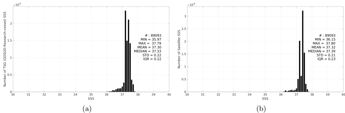
Figure 3: Histograms of SSS from TSG (GOSUD-Research-vessel) (a) and CCI SSS L4 Merged-OI v5.5 - 7-day running (ESA) (b) considering all match-up pairs per bins of 0.1 over the SPURS 1 Pi-MEP region and for the full satellite product period.
