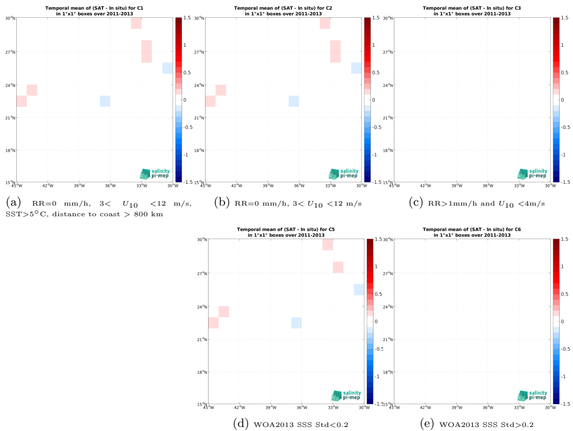
Figure 14: Temporal mean gridded over spatial boxes of size 1^\circ \times 1^\circ of \Delta SSS (CCI SSS L4 Merged-OI v5.5 - 7-day running (ESA) - TSG (CSIC-UTM)) for 5 different subdatasets corresponding to:RR=0 mm/h, 3 < U_{10} < 12 m/s, SST >5^\circ C, distance to coast > 800 km (a), RR=0 mm/h, 3 < U_{10} < 12 m/s (b), RR >1 mm/h and U_{10} < 4 m/s (c), WOA2013 SSS Std <0.2 (d), WOA2013 SSS Std >0.2 (e).
