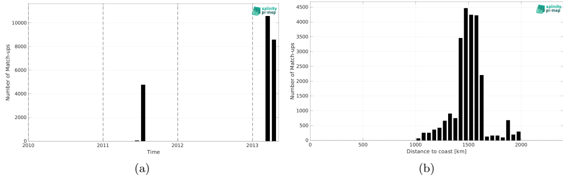
Figure 2: Number of match-ups between TSG (CSIC-UTM) and CCI SSS L4 Merged-OI v5.5 - 7-day running (ESA) SSS as a function of time (a) and as function of the distance to coast (b) over the SPURS 1 Pi-MEP region and for the full satellite product period.
