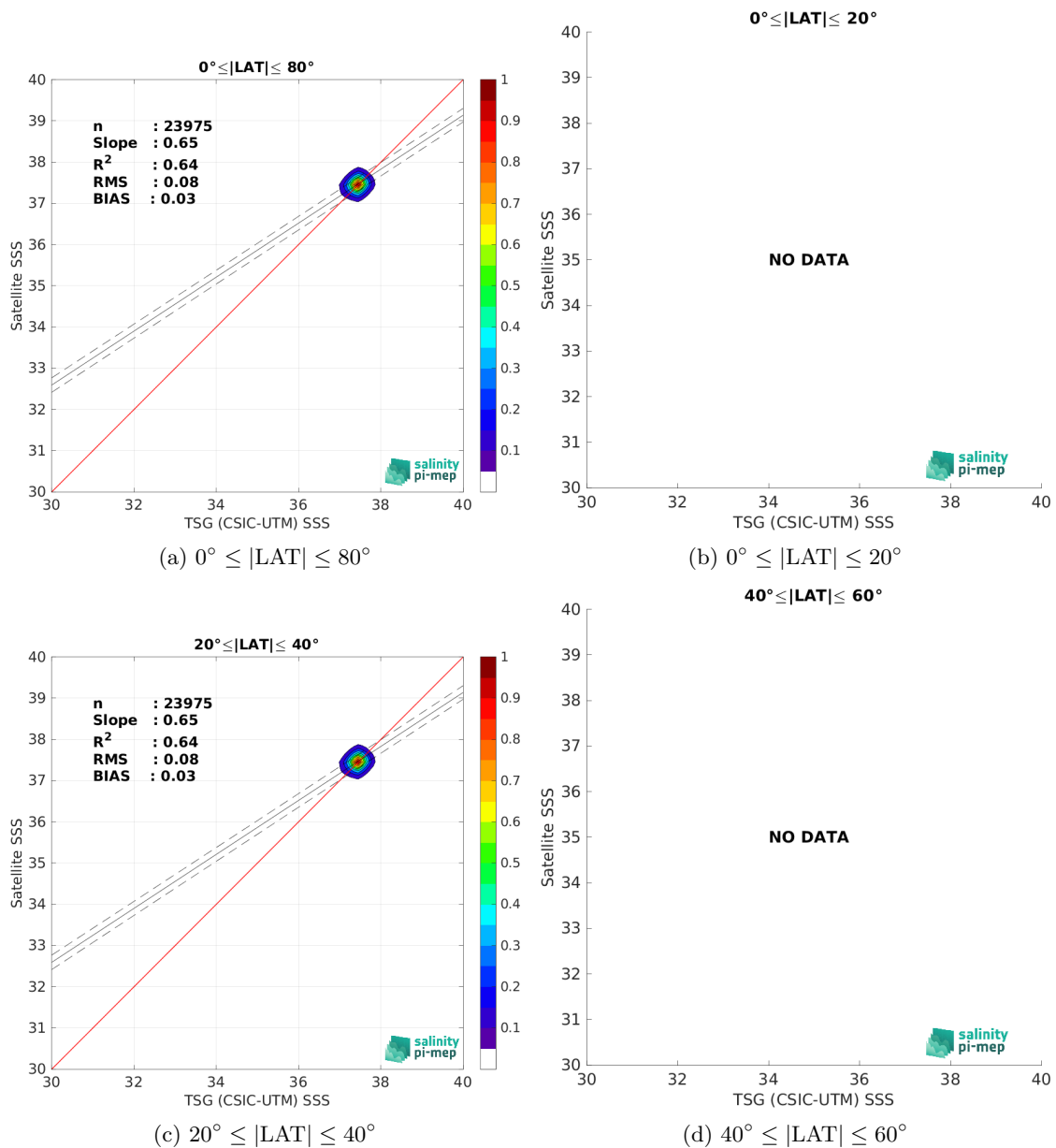
Figure 10: Contour maps of the concentration of CCI SSS L4 Merged-OI v5.5 - 7-day running (ESA) SSS (y-axis) versus TSG (CSIC-UTM) SSS (x-axis) at match-up pairs for different latitude bands. For each plot, the red line shows x=y . The black thin and dashed lines indicate a linear fit through the data cloud and the \pm 95\% confidence levels, respectively. The number match-up pairs n , the slope and R^2 coefficient of the linear fit, the root mean square (RMS) and the mean bias between satellite and in situ data are indicated for each latitude band in each plot.
