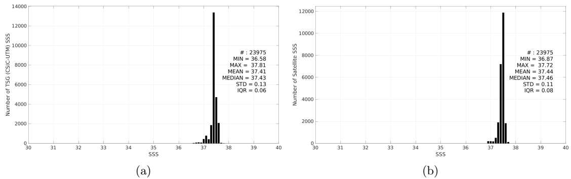
Figure 3: Histograms of SSS from TSG (CSIC-UTM) (a) and CCI SSS L4 Merged-OI v5.5 - 7-day running (ESA) (b) considering all match-up pairs per bins of 0.1 over the SPURS 1 Pi-MEP region and for the full satellite product period.
