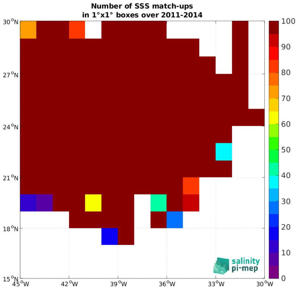
Figure 4: Number of SSS match-ups between Surface drifters SSS and the CCI SSS L4 Merged-OI v5.5 - 7-day running (ESA) SSS product for the SPURS 1 Pi-MEP region over 1°x1° boxes and for the full satellite product period.
