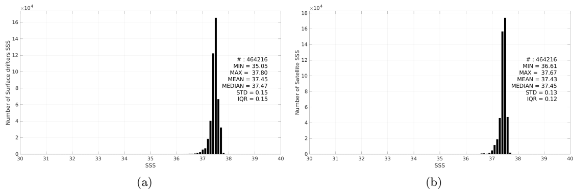
Figure 3: Histograms of SSS from Surface drifters (a) and CCI SSS L4 Merged-OI v5.5 - 7-day running (ESA) (b) considering all match-up pairs per bins of 0.1 over the SPURS 1 Pi-MEP region and for the full satellite product period.
