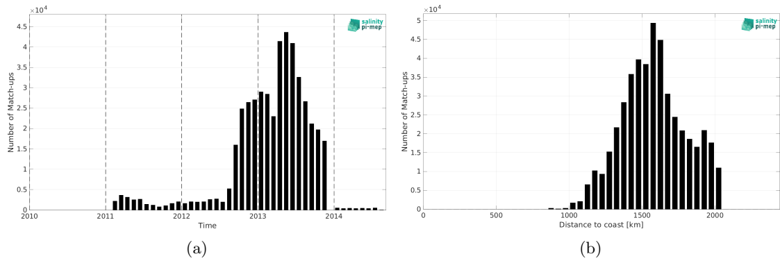
Figure 2: Number of match-ups between Surface drifters and CCI SSS L4 Merged-OI v5.5 - 7-day running (ESA) SSS as a function of time (a) and as function of the distance to coast (b) over the SPURS 1 Pi-MEP region and for the full satellite product period.
