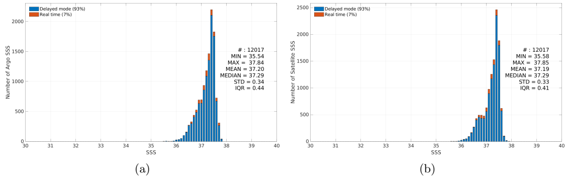
Figure 3: Histograms of SSS from Argo (a) and CCI SSS L4 Merged-OI v5.5 - 7-day running (ESA) (b) considering all match-up pairs per bins of 0.1 over the SPURS 1 Pi-MEP region and for the full satellite product period.
