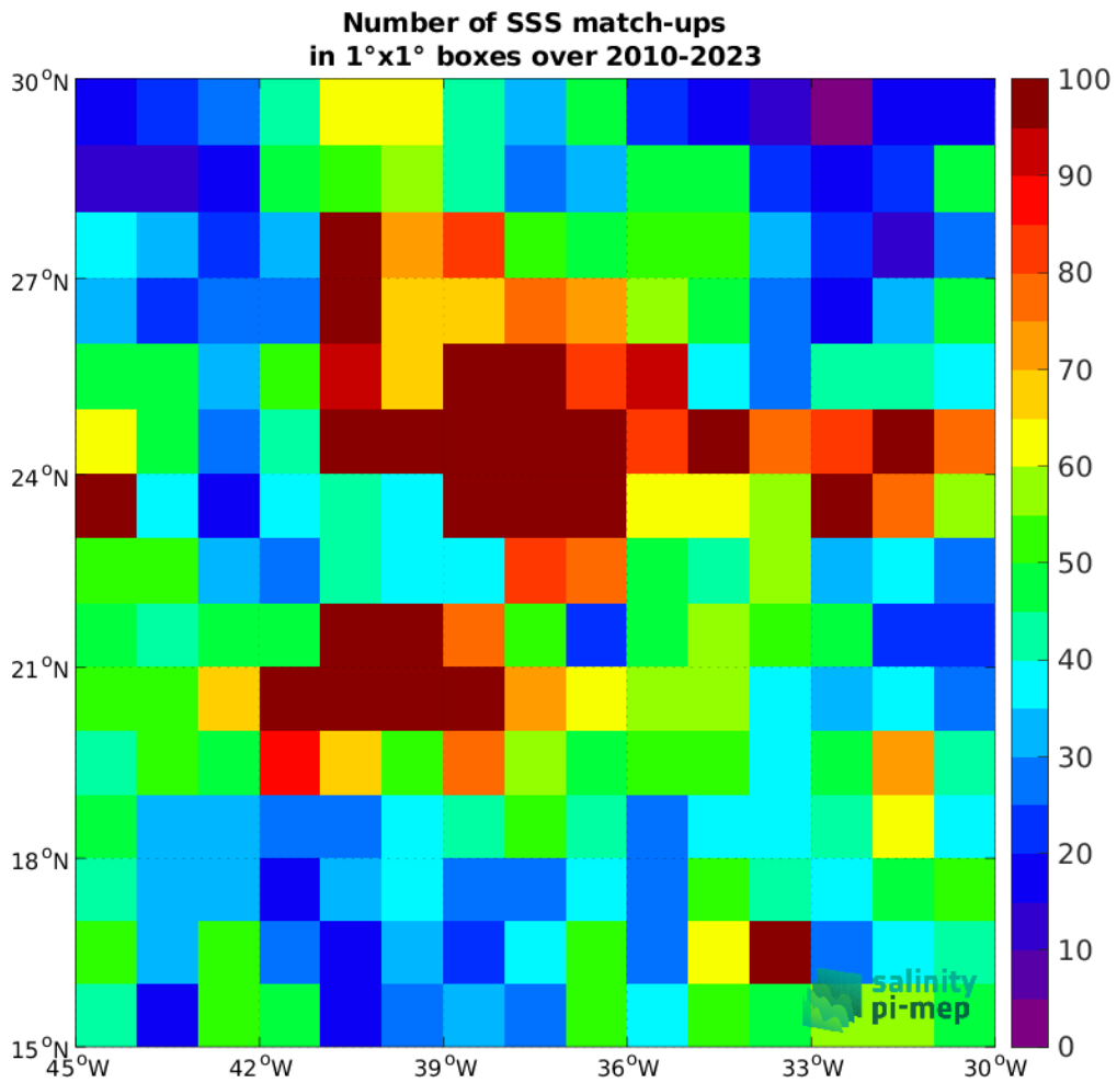
Figure 5: Number of SSS match-ups between Argo SSS and the CCI SSS L4 Merged-OI v5.5 - 7-day running (ESA) SSS product for the SPURS 1 Pi-MEP region over 1°x1° boxes and for the full satellite product period.
