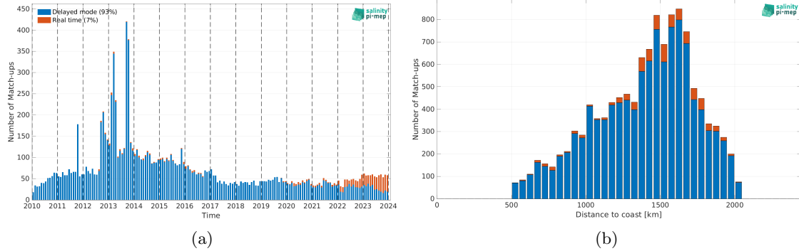
Figure 2: Number of match-ups between Argo and CCI SSS L4 Merged-OI v5.5 - 7-day running (ESA) SSS as a function of time (a) and as function of the distance to coast (b) over the SPURS 1 Pi-MEP region and for the full satellite product period.
