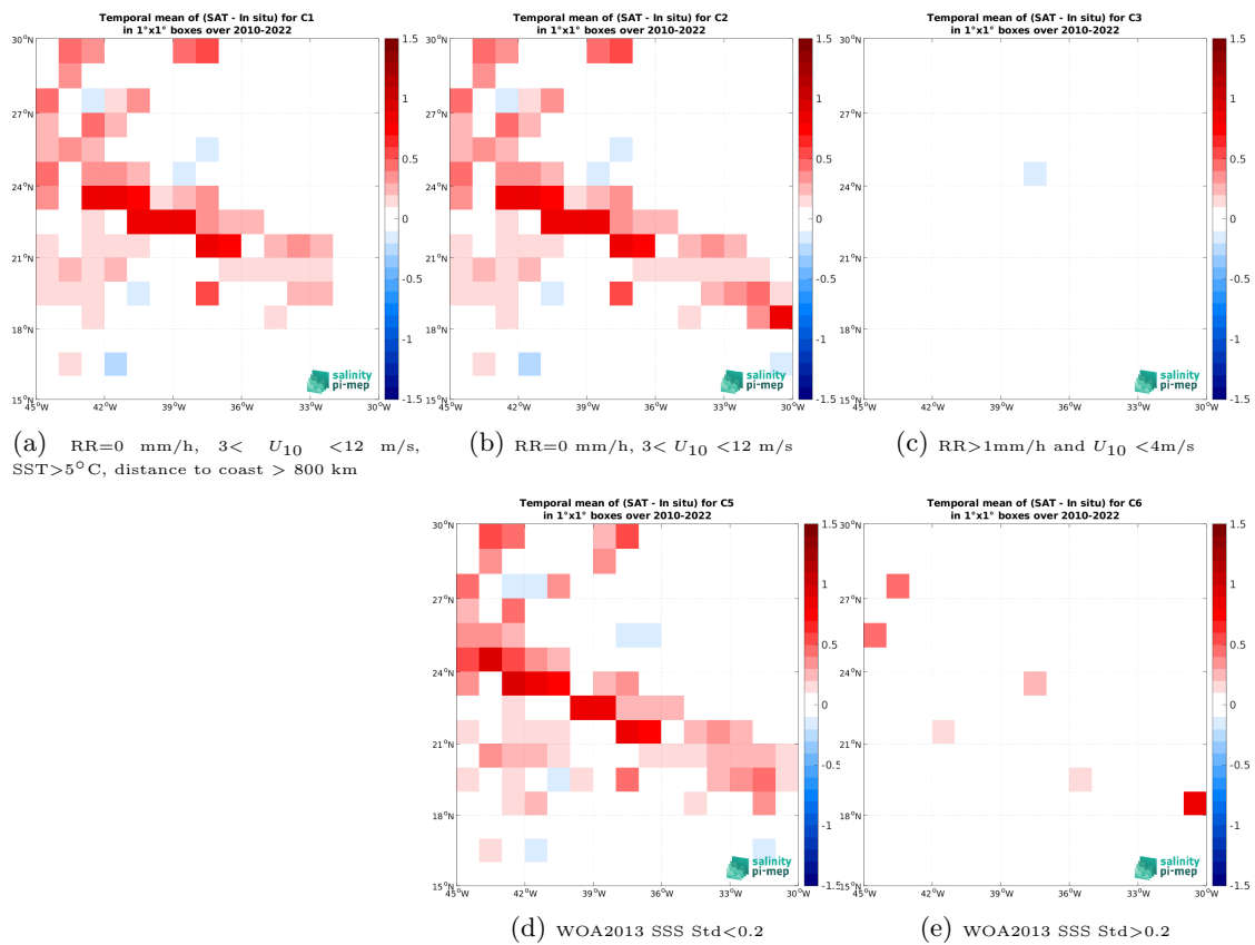
Figure 14: Temporal mean gridded over spatial boxes of size 1^\circ \times 1^\circ of \Delta SSS (CCI SSS L4 Merged-OI v5.5 - 30-day running (ESA) - TSG (SAMOS)) for 5 different subdatasets corresponding to:RR=0 mm/h, 3 < U_{10} < 12 m/s, SST >5^\circ C, distance to coast > 800 km (a), RR=0 mm/h, 3 < U_{10} < 12 m/s (b), RR >1 mm/h and U_{10} < 4 m/s (c), WOA2013 SSS Std <0.2 (d), WOA2013 SSS Std >0.2 (e).
