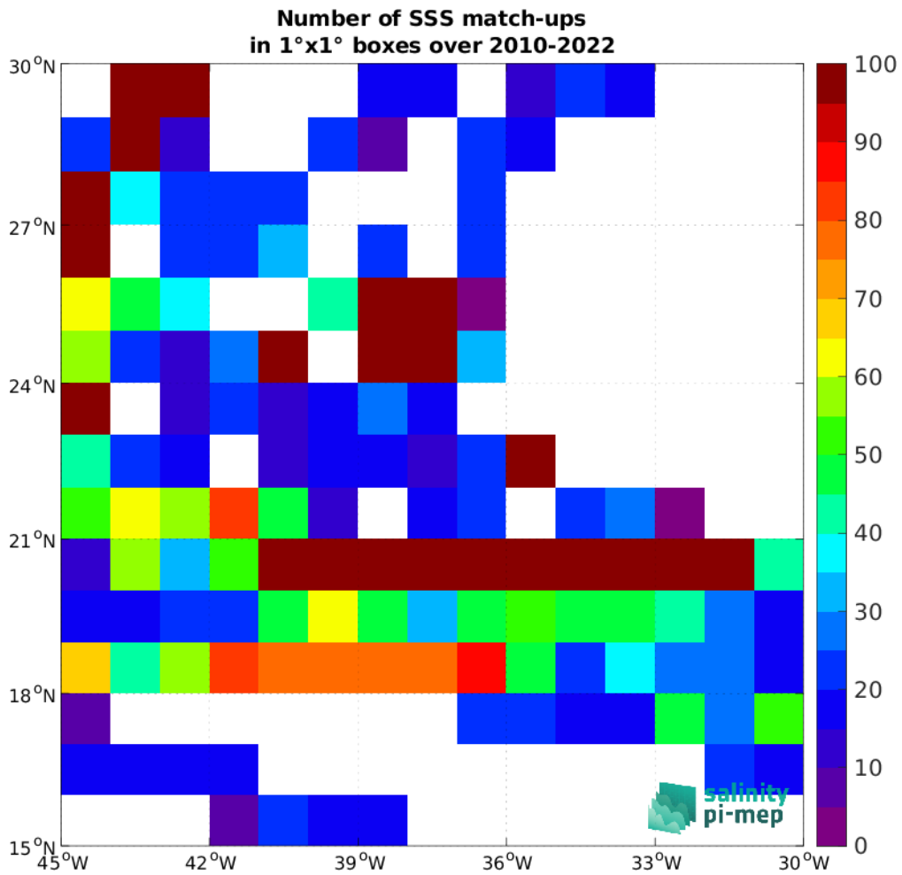
Figure 5: Number of SSS match-ups between TSG (SAMOS) SSS and the CCI SSS L4 Merged-OI v5.5 - 30-day running (ESA) SSS product for the SPURS 1 Pi-MEP region over 1^\circ \times 1^\circ boxes and for the full satellite product period.
