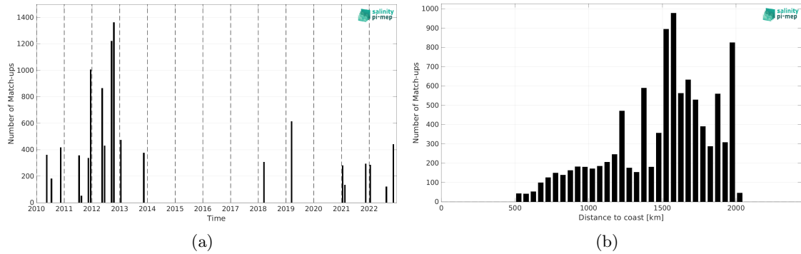
Figure 2: Number of match-ups between TSG (SAMOS) and CCI SSS L4 Merged-OI v5.5 - 30-day running (ESA) SSS as a function of time (a) and as function of the distance to coast (b) over the SPURS 1 Pi-MEP region and for the full satellite product period.
