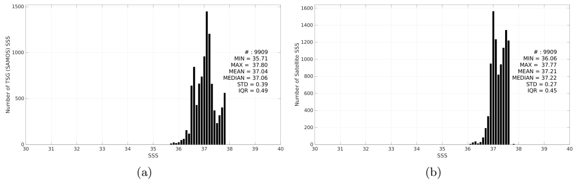
Figure 3: Histograms of SSS from TSG (SAMOS) (a) and CCI SSS L4 Merged-OI v5.5 - 30-day running (ESA) (b) considering all match-up pairs per bins of 0.1 over the SPURS 1 Pi-MEP region and for the full satellite product period.
