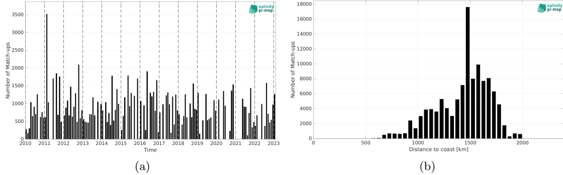
Figure 2: Number of match-ups between TSG (LEGOS-DM) and CCI SSS L4 Merged-OI v5.5 - 30-day running (ESA) SSS as a function of time (a) and as function of the distance to coast (b) over the SPURS 1 Pi-MEP region and for the full satellite product period.
