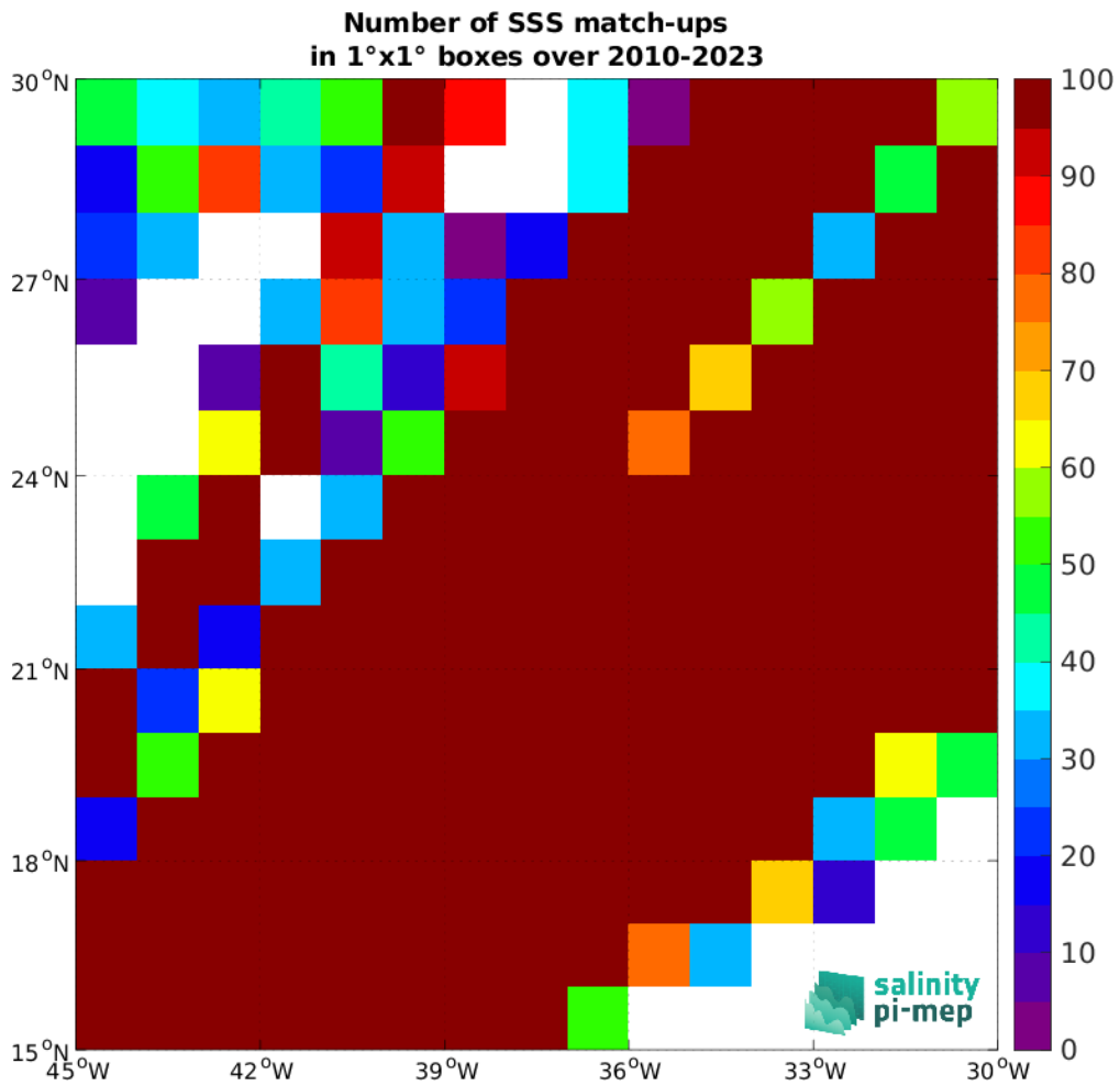
Figure 5: Number of SSS match-ups between TSG (LEGOS-DM) SSS and the CCI SSS L4 Merged-OI v5.5 - 30-day running (ESA) SSS product for the SPURS 1 Pi-MEP region over 1^\circ \times 1^\circ boxes and for the full satellite product period.
