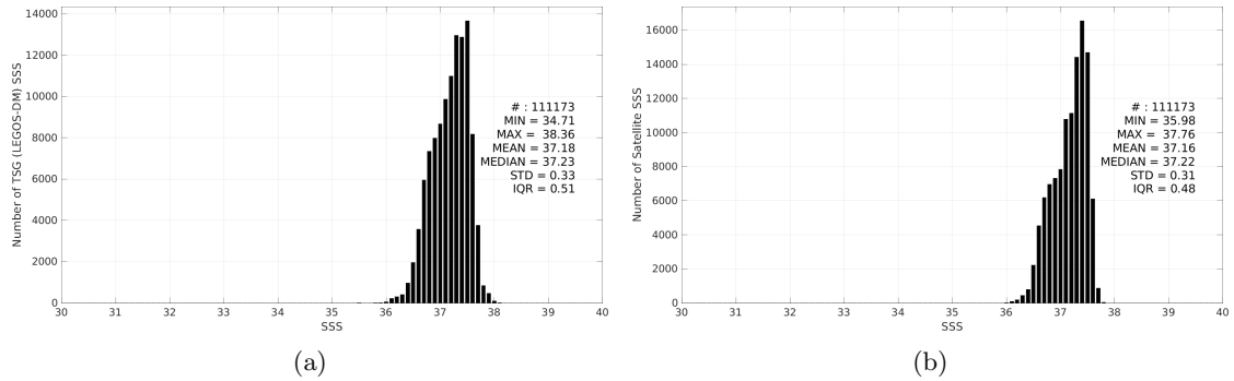
Figure 3: Histograms of SSS from TSG (LEGOS-DM) (a) and CCI SSS L4 Merged-OI v5.5 - 30-day running (ESA) (b) considering all match-up pairs per bins of 0.1 over the SPURS 1 Pi-MEP region and for the full satellite product period.
