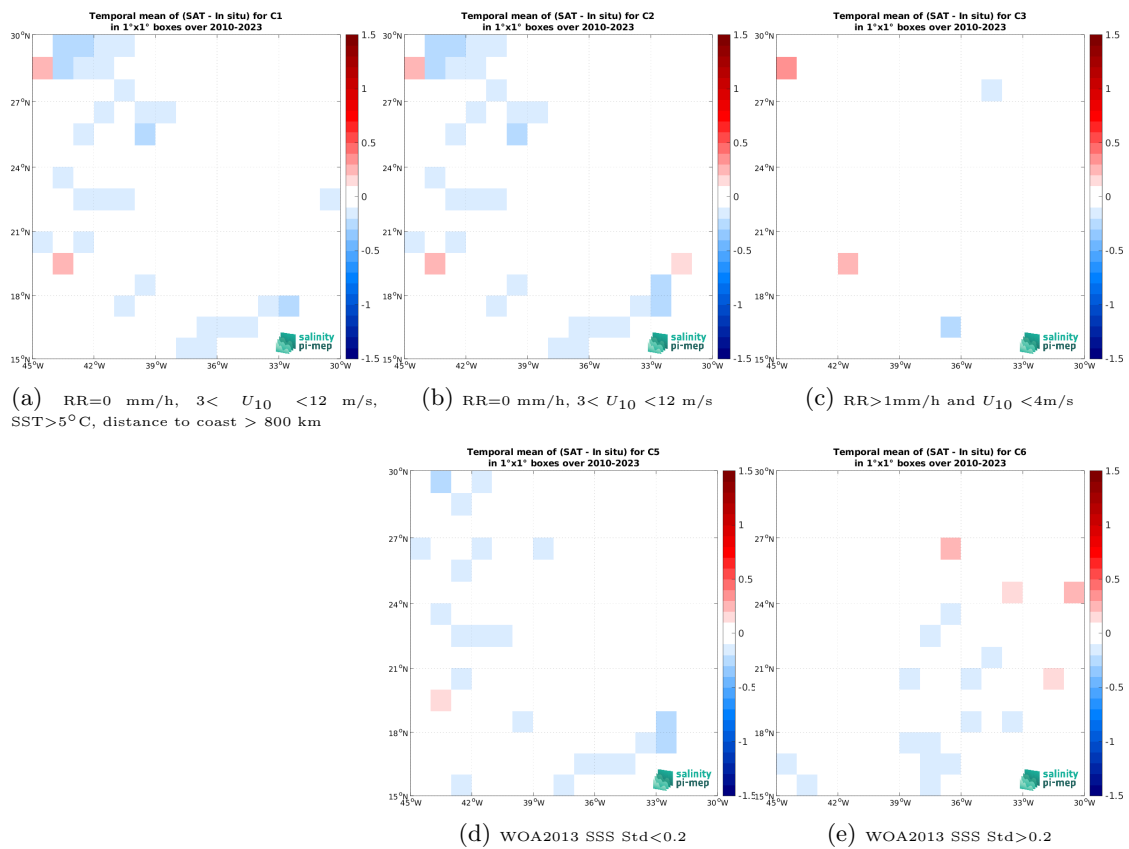
Figure 14: Temporal mean gridded over spatial boxes of size 1^\circ \times 1^\circ of \Delta SSS (CCI SSS L4 Merged-OI v5.5 - 30-day running (ESA) - TSG (LEGOS-DM)) for 5 different subdatasets corresponding to: RR=0 mm/h, 3 < U_{10} < 12 m/s, SST > 5^\circ C , distance to coast > 800 km (a), RR=0 mm/h, 3 < U_{10} < 12 m/s (b), RR > 1 mm/h and U_{10} < 4 m/s (c), WOA2013 SSS Std < 0.2 (d), WOA2013 SSS Std > 0.2 (e).
