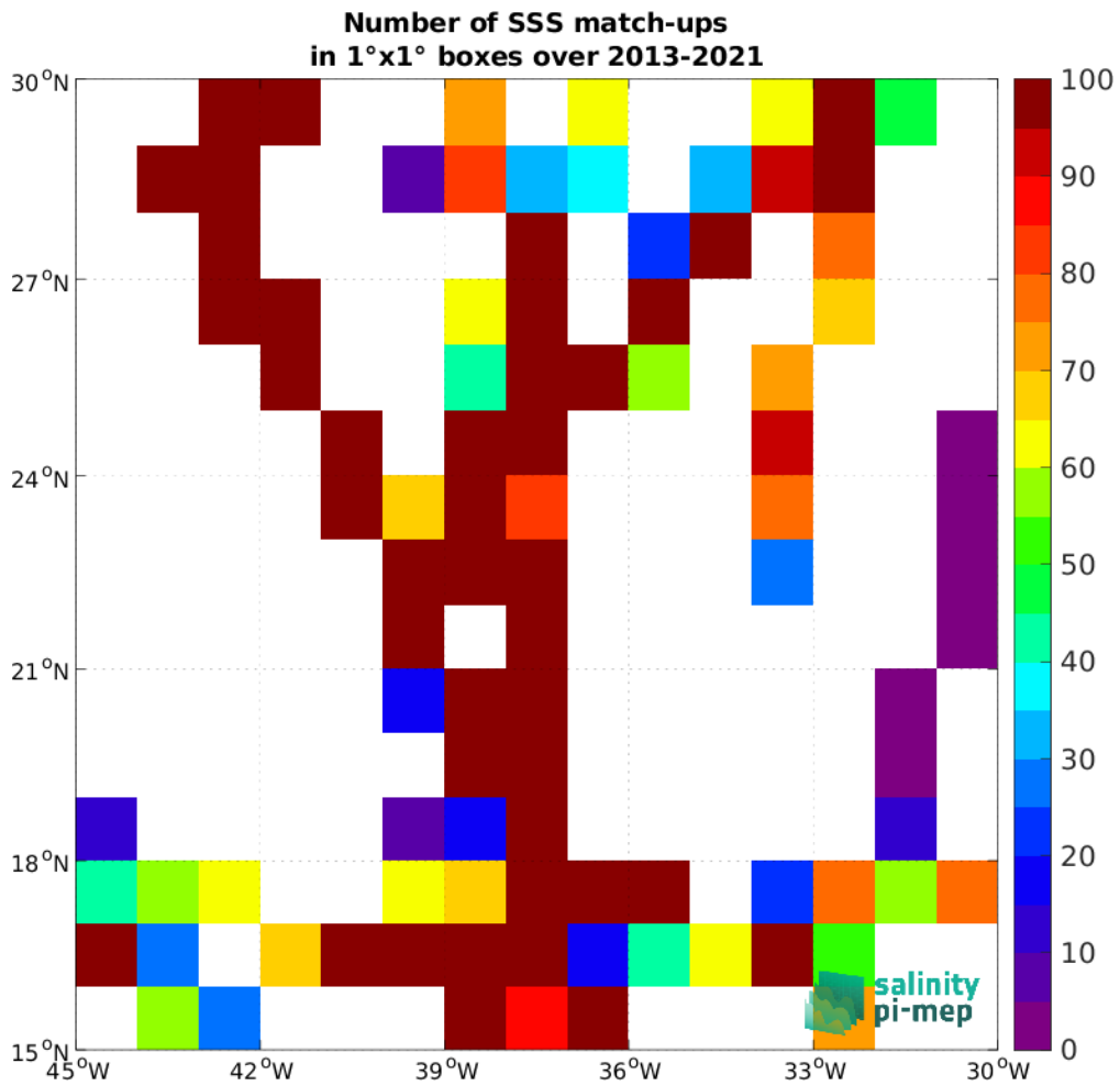
Figure 5: Number of SSS match-ups between TSG (GOSUD-Sailing-ship) SSS and the CCI SSS L4 Merged-OI v5.5 - 30-day running (ESA) SSS product for the SPURS 1 Pi-MEP region over 1^\circ \times 1^\circ boxes and for the full satellite product period.
