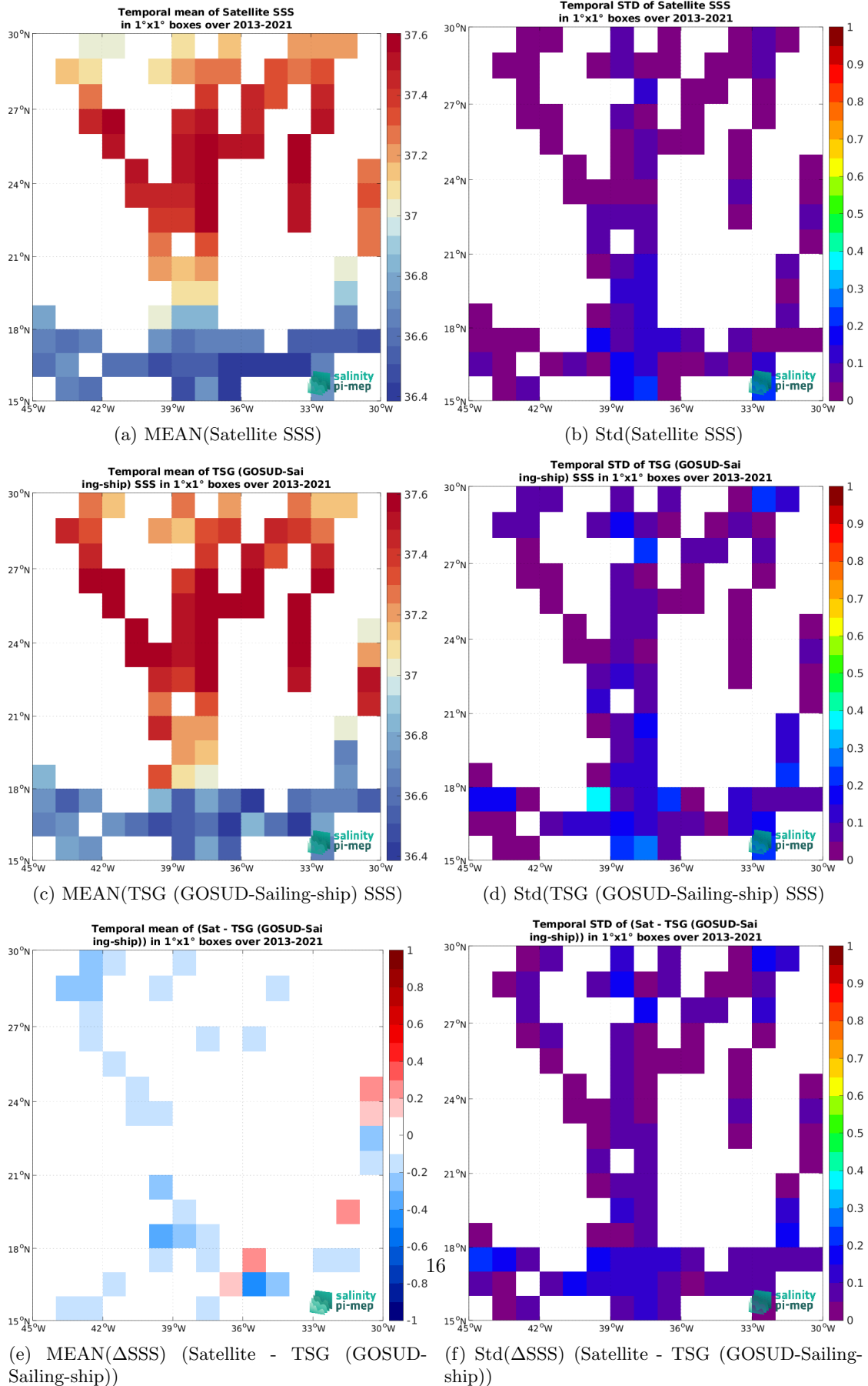
Figure 7: Temporal mean (left) and Std (right) of SSS from CCI SSS L4 Merged-OI v5.5 - 30-day running (ESA) (top), TSG (GOSUD-Sailing-ship) (middle), and of \Delta SSS (Satellite - TSG (GOSUD-Sailing-ship)). Only match-up pairs are used to generate these maps.
