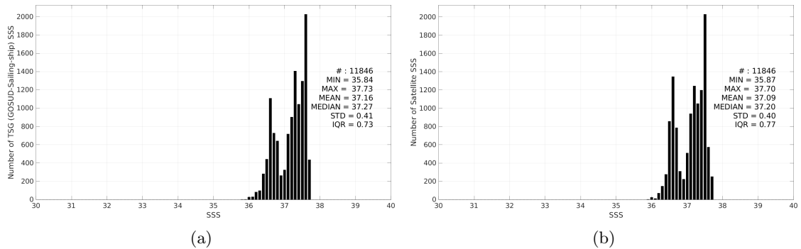
Figure 3: Histograms of SSS from TSG (GOSUD-Sailing-ship) (a) and CCI SSS L4 Merged-OI v5.5 - 30-day running (ESA) (b) considering all match-up pairs per bins of 0.1 over the SPURS 1 Pi-MEP region and for the full satellite product period.
