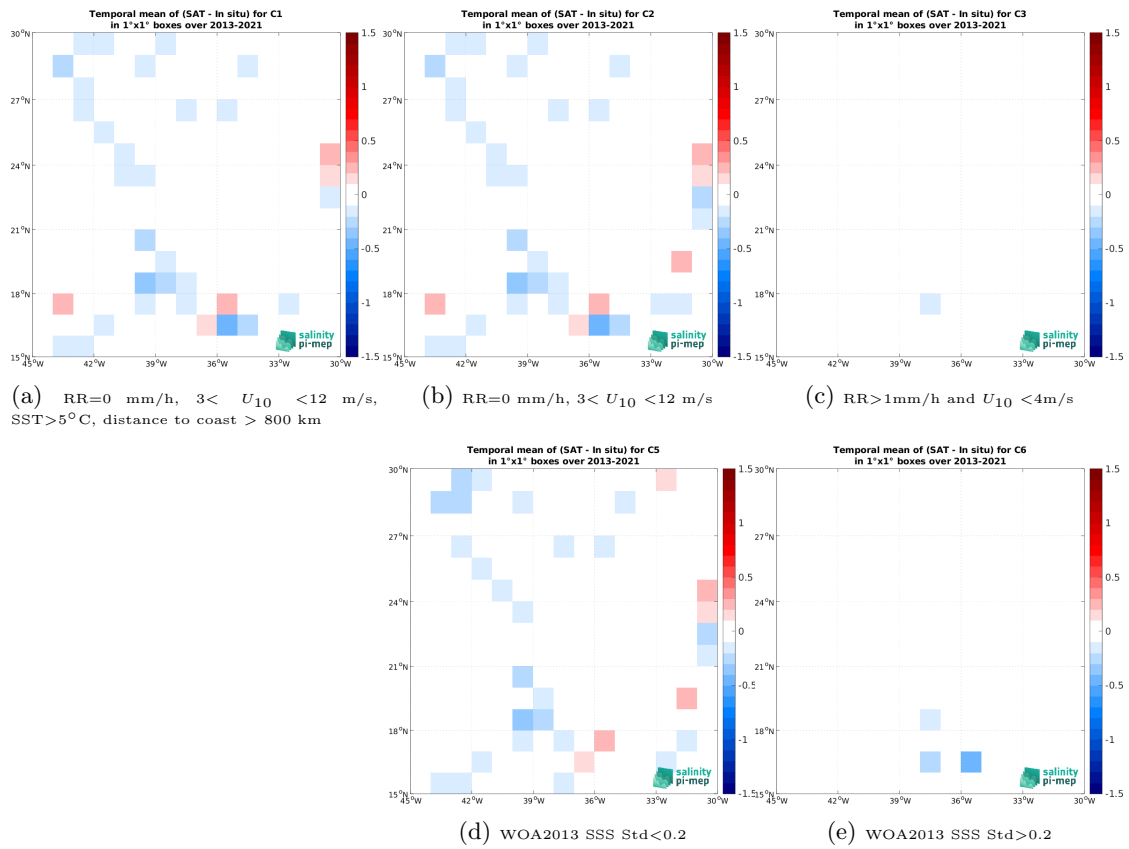
Figure 14: Temporal mean gridded over spatial boxes of size 1^\circ \times 1^\circ of \Delta SSS (CCI SSS L4 Merged-OI v5.5 - 30-day running (ESA) - TSG (GOSUD-Sailing-ship)) for 5 different subdatasets corresponding to: RR=0 mm/h, 3 < U_{10} < 12 m/s, SST > 5^\circ C , distance to coast > 800 km (a), RR=0 mm/h, 3 < U_{10} < 12 m/s (b), RR > 1 mm/h and U_{10} < 4 m/s (c), WOA2013 SSS Std < 0.2 (d), WOA2013 SSS Std > 0.2 (e).
