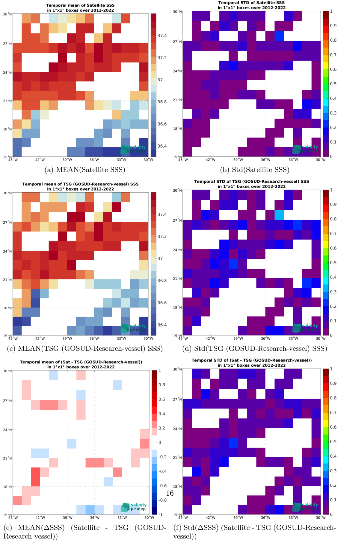
Figure 7: Temporal mean (left) and Std (right) of SSS from CCI SSS L4 Merged-OI v5.5 - 30-day running (ESA) (top), TSG (GOSUD-Research-vessel) (middle), and of \Delta SSS (Satellite - TSG (GOSUD-Research-vessel)). Only match-up pairs are used to generate these maps.
