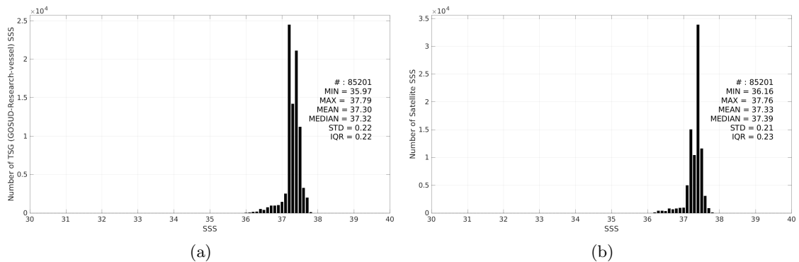
Figure 3: Histograms of SSS from TSG (GOSUD-Research-vessel) (a) and CCI SSS L4 Merged-OI v5.5 - 30-day running (ESA) (b) considering all match-up pairs per bins of 0.1 over the SPURS 1 Pi-MEP region and for the full satellite product period.
