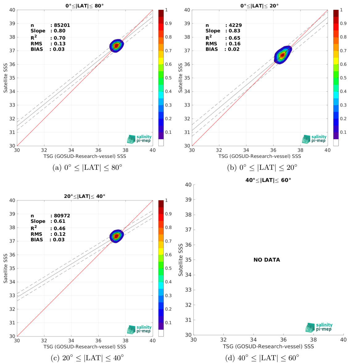
Figure 10: Contour maps of the concentration of CCI SSS L4 Merged-OI v5.5 - 30-day running (ESA) SSS (y-axis) versus TSG (GOSUD-Research-vessel) SSS (x-axis) at match-up pairs for different latitude bands. For each plot, the red line shows x=y . The black thin and dashed lines indicate a linear fit through the data cloud and the \pm 95\% confidence levels, respectively. The number match-up pairs n , the slope and R^2 coefficient of the linear fit, the root mean square (RMS) and the mean bias between satellite and in situ data are indicated for each latitude band in each plots.
