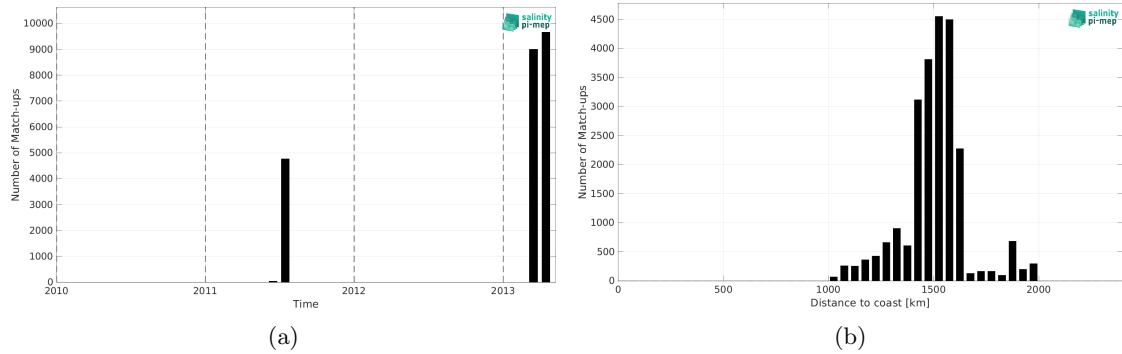
Figure 2: Number of match-ups between TSG (CSIC-UTM) and CCI SSS L4 Merged-OI v5.5 - 30-day running (ESA) SSS as a function of time (a) and as function of the distance to coast (b) over the SPURS 1 Pi-MEP region and for the full satellite product period.
