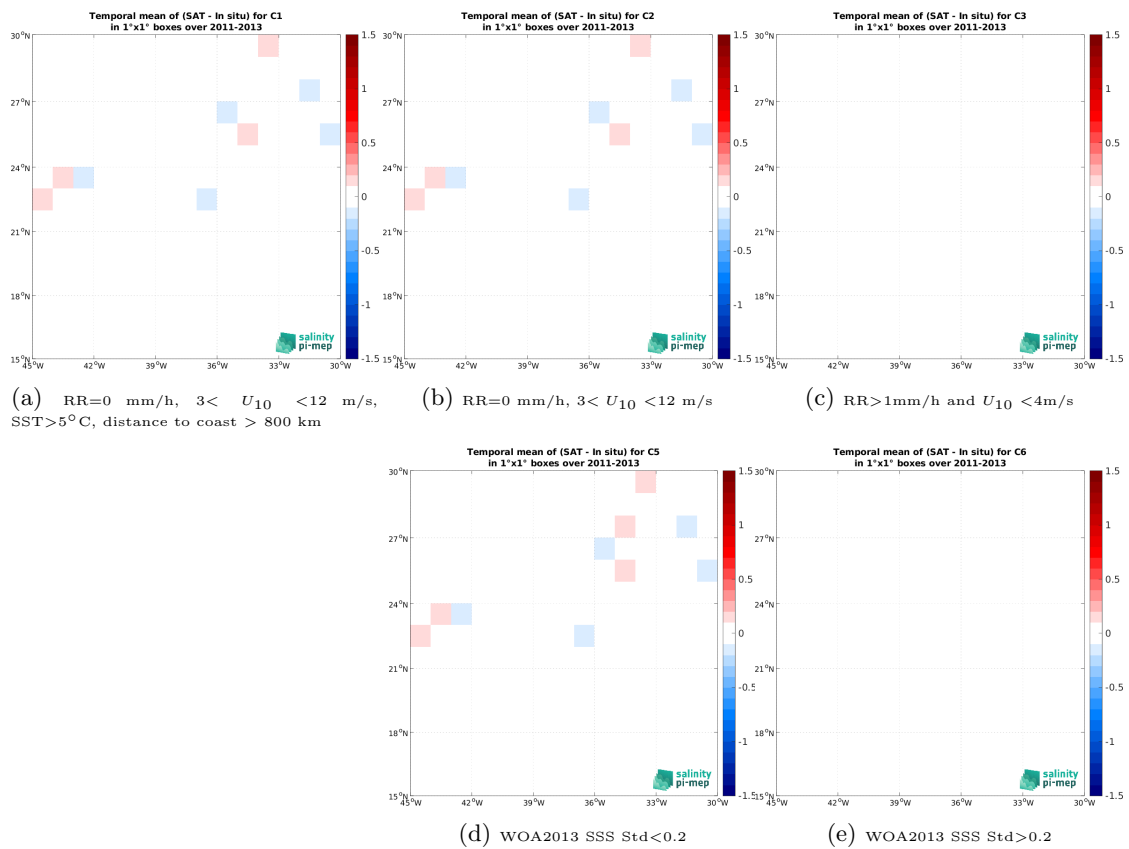
Figure 14: Temporal mean gridded over spatial boxes of size 1^\circ \times 1^\circ of \Delta\text{SSS} (CCI SSS L4 Merged-OI v5.5 - 30-day running (ESA) - TSG (CSIC-UTM)) for 5 different subdatasets corresponding to:RR=0 mm/h, 3 < U_{10} < 12 m/s, SST >5^\circ\text{C} , distance to coast > 800 km (a), RR=0 mm/h, 3 < U_{10} < 12 m/s (b), RR >1 mm/h and U_{10} < 4 m/s (c), WOA2013 SSS Std <0.2 (d), WOA2013 SSS Std >0.2 (e).
