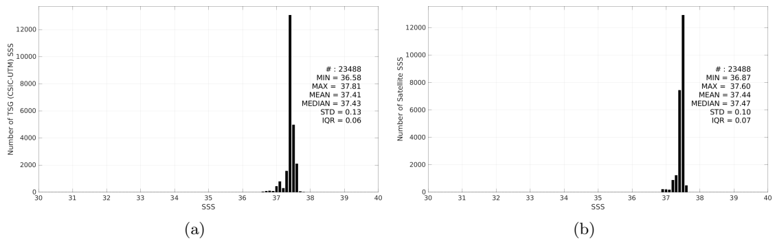
Figure 3: Histograms of SSS from TSG (CSIC-UTM) (a) and CCI SSS L4 Merged-OI v5.5 - 30-day running (ESA) (b) considering all match-up pairs per bins of 0.1 over the SPURS 1 Pi-MEP region and for the full satellite product period.
