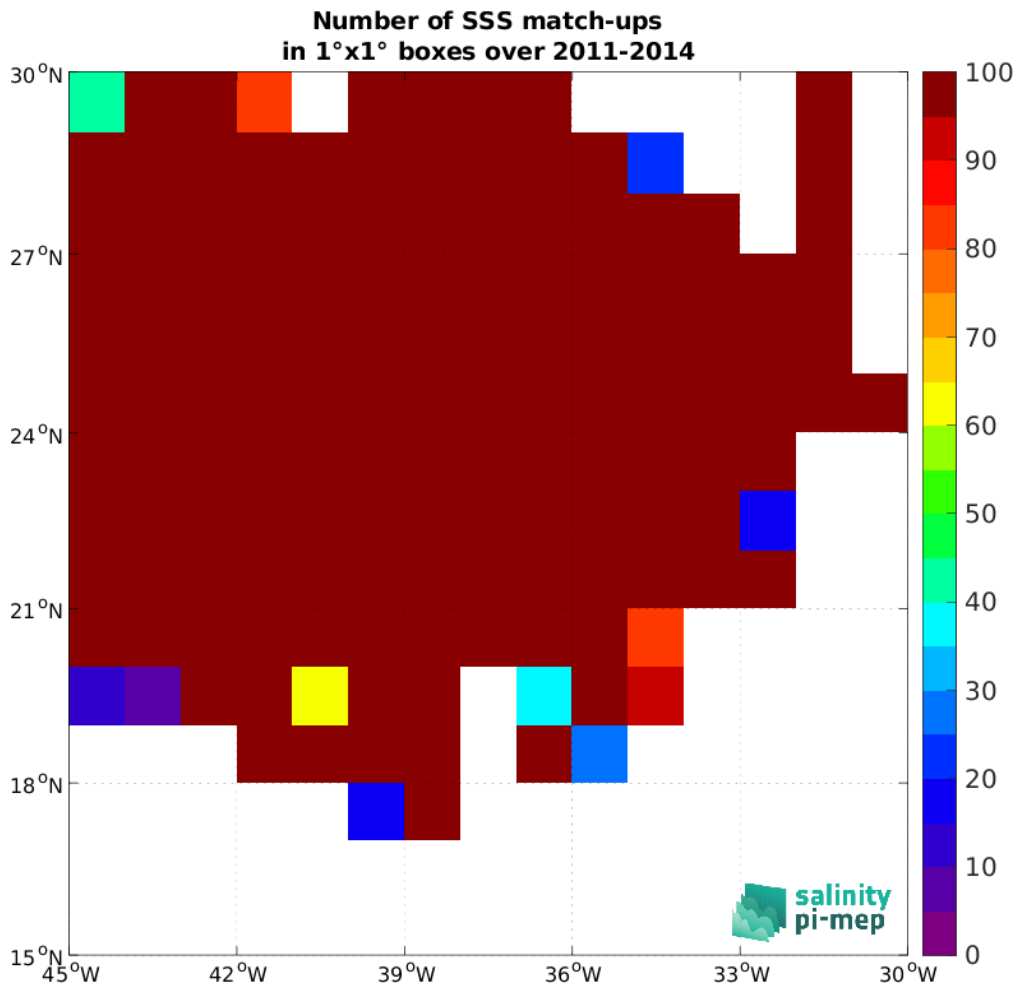
Figure 4: Number of SSS match-ups between Surface drifters SSS and the CCI SSS L4 Merged-OI v5.5 - 30-day running (ESA) SSS product for the SPURS 1 Pi-MEP region over 1^\circ \times 1^\circ boxes and for the full satellite product period.
