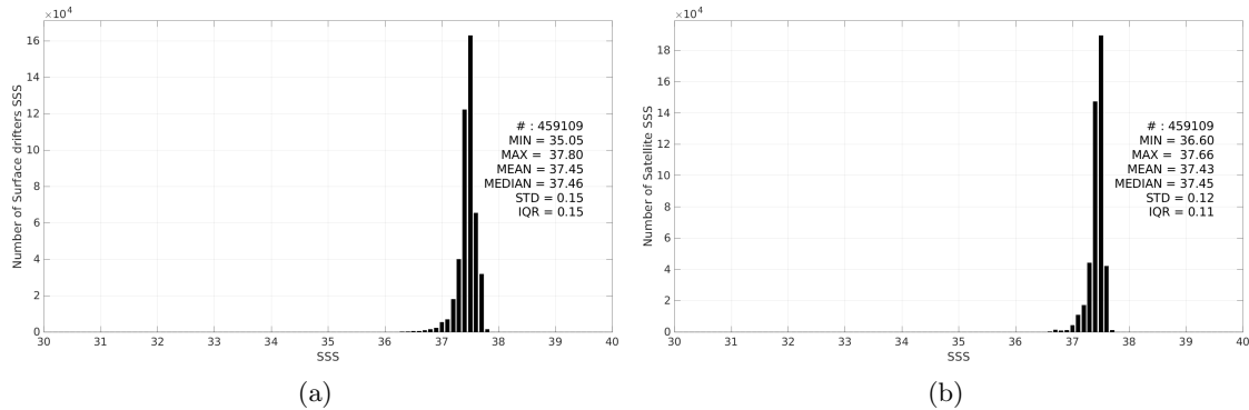
Figure 3: Histograms of SSS from Surface drifters (a) and CCI SSS L4 Merged-OI v5.5 - 30-day running (ESA) (b) considering all match-up pairs per bins of 0.1 over the SPURS 1 Pi-MEP region and for the full satellite product period.
