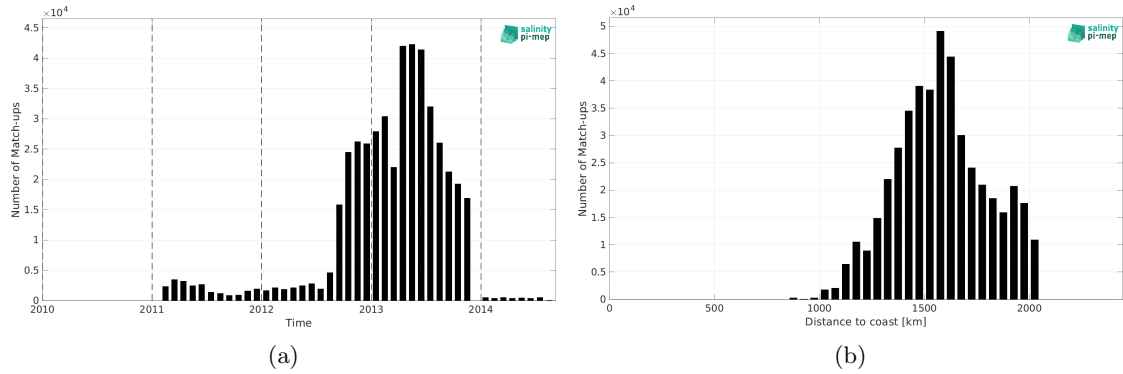
Figure 2: Number of match-ups between Surface drifters and CCI SSS L4 Merged-OI v5.5 - 30-day running (ESA) SSS as a function of time (a) and as function of the distance to coast (b) over the SPURS 1 Pi-MEP region and for the full satellite product period.
