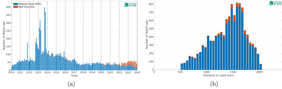
Figure 2: Number of match-ups between Argo and CCI SSS L4 Merged-OI v5.5 - 30-day running (ESA) SSS as a function of time (a) and as function of the distance to coast (b) over the SPURS 1 Pi-MEP region and for the full satellite product period.
