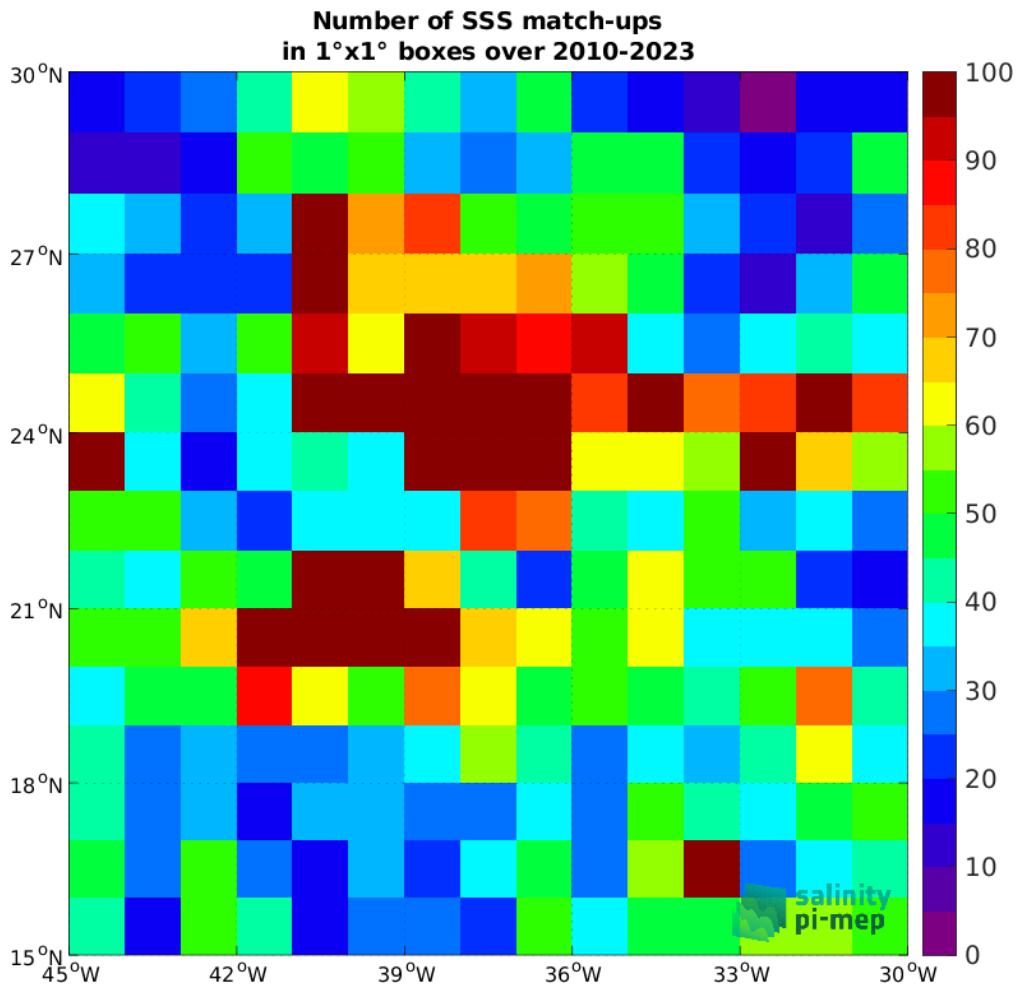
Figure 5: Number of SSS match-ups between Argo SSS and the CCI SSS L4 Merged-OI v5.5 - 30-day running (ESA) SSS product for the SPURS 1 Pi-MEP region over 1^\circ \times 1^\circ boxes and for the full satellite product period.
