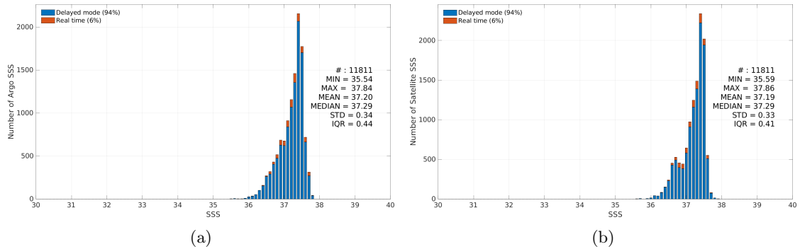
Figure 3: Histograms of SSS from Argo (a) and CCI SSS L4 Merged-OI v5.5 - 30-day running (ESA) (b) considering all match-up pairs per bins of 0.1 over the SPURS 1 Pi-MEP region and for the full satellite product period.
