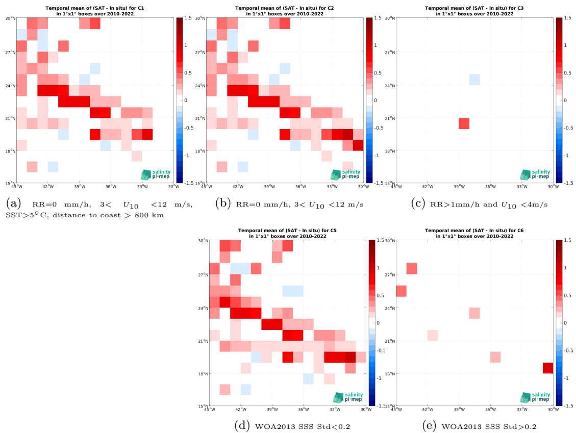
Figure 14: Temporal mean gridded over spatial boxes of size 1^\circ \times 1^\circ of \Delta SSS (CCI SSS L4 Merged-OI v4.41 - 7-day running (ESA) - TSG (SAMOS)) for 5 different subdatasets corresponding to: RR=0 mm/h, 3 < U_{10} < 12 m/s, SST > 5^\circ C , distance to coast > 800 km (a), RR=0 mm/h, 3 < U_{10} < 12 m/s (b), RR > 1 mm/h and U_{10} < 4 m/s (c), WOA2013 SSS Std < 0.2 (d), WOA2013 SSS Std > 0.2 (e).
