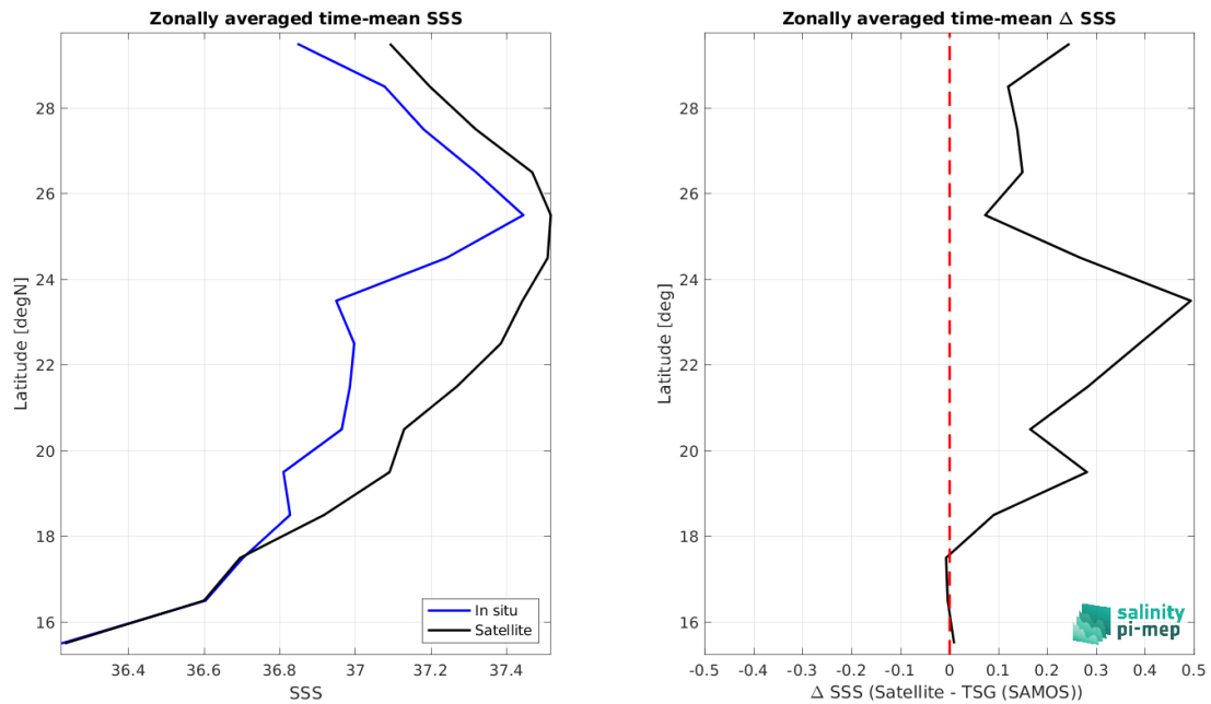
Figure 9: Left panel: Zonal mean SSS from CCI SSS L4 Merged-OI v4.41 - 7-day running (ESA) satellite product (black) and from TSG (SAMOS) (blue). Right panel: Zonal mean of \Delta SSS (Satellite - TSG (SAMOS)) for all the collected Pi-MEP match-up pairs estimated over the full satellite product period.
