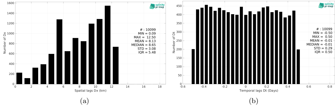
Figure 6: Histograms of the spatial (a) and temporal (b) lags between the location/time of the TSG (SAMOS) measurement and the date of the corresponding CCI SSS L4 Merged-OI v4.41 - 7-day running (ESA) SSS pixel.
