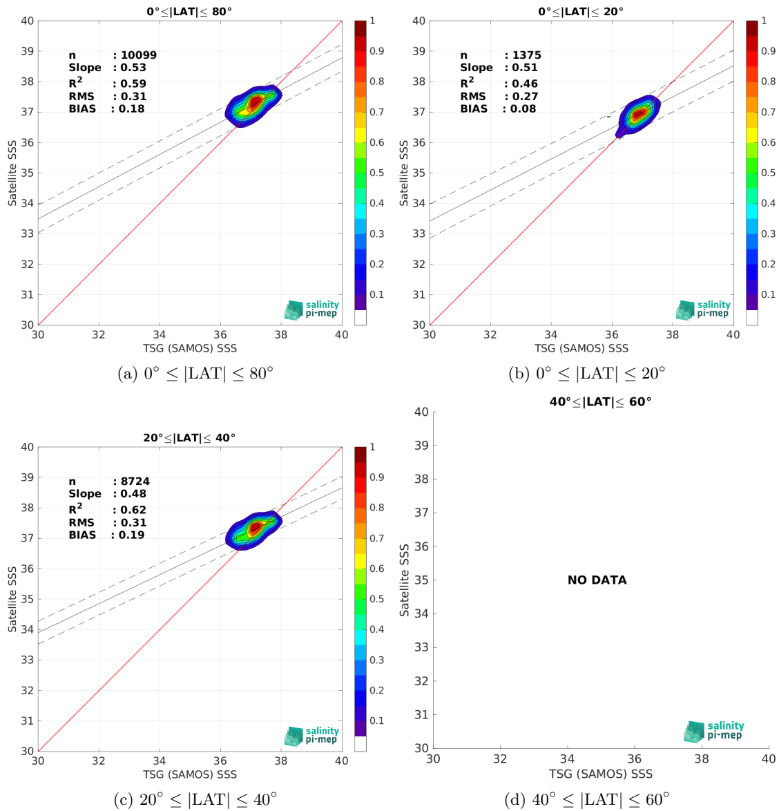
Figure 10: Contour maps of the concentration of CCI SSS L4 Merged-OI v4.41 - 7-day running (ESA) SSS (y-axis) versus TSG (SAMOS) SSS (x-axis) at match-up pairs for different latitude bands. For each plot, the red line shows x=y . The black thin and dashed lines indicate a linear fit through the data cloud and the \pm 95\% confidence levels, respectively. The number match-up pairs n , the slope and R^2 coefficient of the linear fit, the root mean square (RMS) and the mean bias between satellite and in situ data are indicated for each latitude band in each plots.
