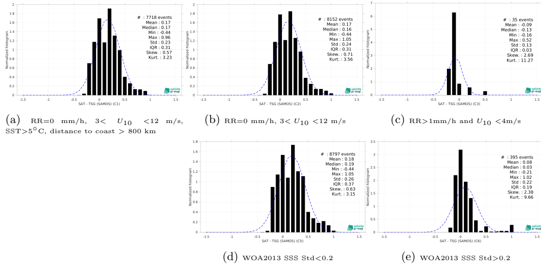
Figure 15: Normalized histogram of \Delta SSS (CCI SSS L4 Merged-OI v4.41 - 7-day running (ESA) - TSG (SAMOS)) for 5 different subdatasets corresponding to: RR=0 mm/h, 3 < U_{10} < 12 m/s, SST>5°C, distance to coast > 800 km (a), RR=0 mm/h, 3 < U_{10} < 12 m/s (b), RR>1mm/h and U_{10} < 4 m/s (c), WOA2013 SSS Std<0.2 (d), WOA2013 SSS Std>0.2 (e).
