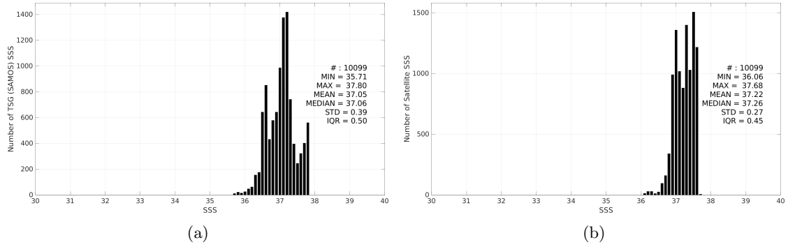
Figure 3: Histograms of SSS from TSG (SAMOS) (a) and CCI SSS L4 Merged-OI v4.41 - 7-day running (ESA) (b) considering all match-up pairs per bins of 0.1 over the SPURS 1 Pi-MEP region and for the full satellite product period.
