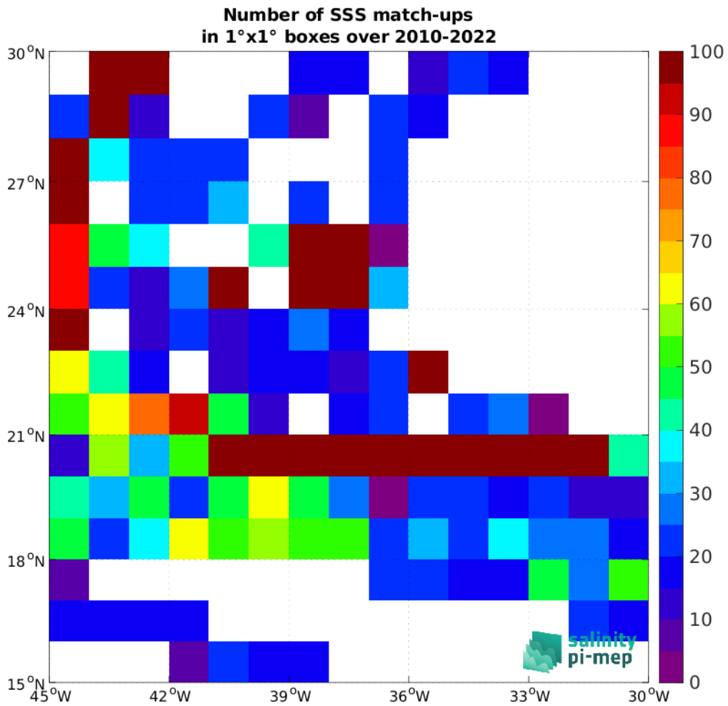
Figure 5: Number of SSS match-ups between TSG (SAMOS) SSS and the CCI SSS L4 Merged-OI v4.41 - 7-day running (ESA) SSS product for the SPURS 1 Pi-MEP region over 1°x1° boxes and for the full satellite product period.
