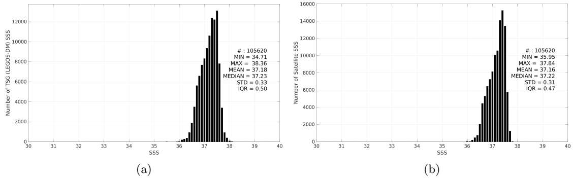
Figure 3: Histograms of SSS from TSG (LEGOS-DM) (a) and CCI SSS L4 Merged-OI v4.41 - 7-day running (ESA) (b) considering all match-up pairs per bins of 0.1 over the SPURS 1 Pi-MEP region and for the full satellite product period.
