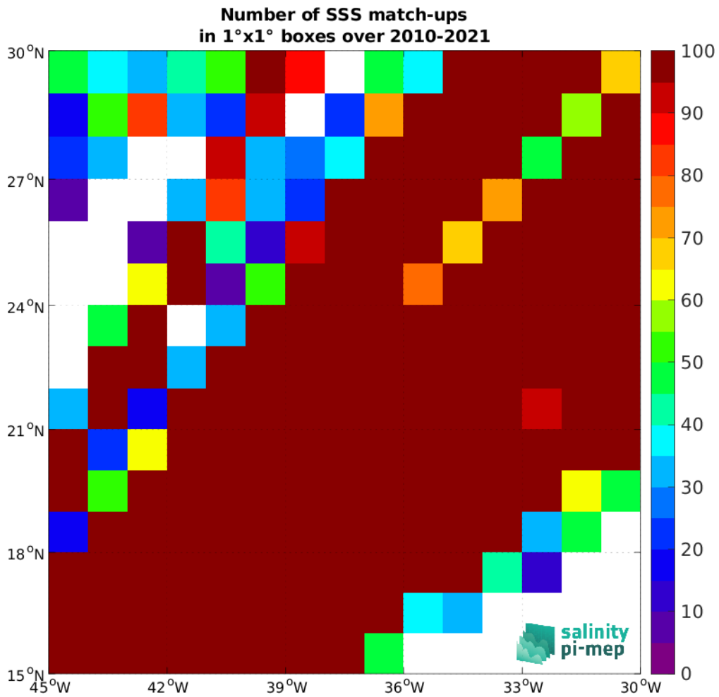
Figure 5: Number of SSS match-ups between TSG (LEGOS-DM) SSS and the CCI SSS L4 Merged-OI v4.41 - 7-day running (ESA) SSS product for the SPURS 1 Pi-MEP region over 1^\circ \times 1^\circ boxes and for the full satellite product period.
