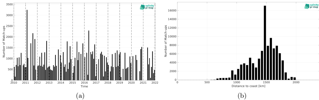
Figure 2: Number of match-ups between TSG (LEGOS-DM) and CCI SSS L4 Merged-OI v4.41 - 7-day running (ESA) SSS as a function of time (a) and as function of the distance to coast (b) over the SPURS 1 Pi-MEP region and for the full satellite product period.
