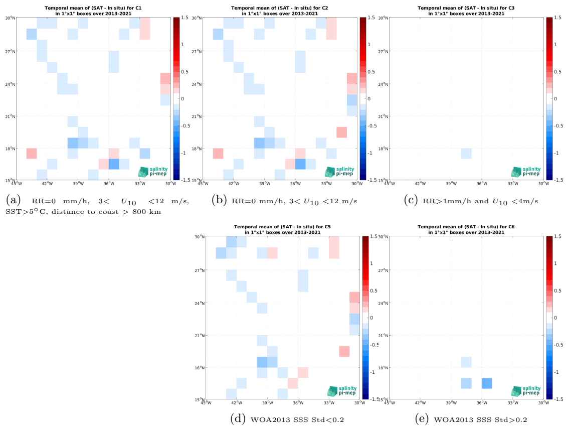
Figure 14: Temporal mean gridded over spatial boxes of size 1^\circ \times 1^\circ of \Delta SSS (CCI SSS L4 Merged-OI v4.41 - 7-day running (ESA) - TSG (GOSUD-Sailing-ship)) for 5 different subdatasets corresponding to: RR=0 mm/h, 3 < U_{10} < 12 m/s, SST > 5^\circ\text{C} , distance to coast > 800 km (a), RR=0 mm/h, 3 < U_{10} < 12 m/s (b), RR > 1 mm/h and U_{10} < 4 m/s (c), WOA2013 SSS Std < 0.2 (d), WOA2013 SSS Std > 0.2 (e).
