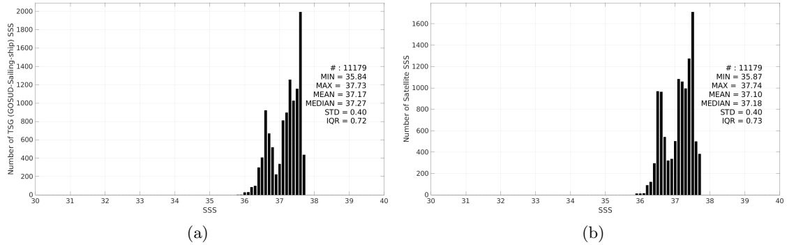
Figure 3: Histograms of SSS from TSG (GOSUD-Sailing-ship) (a) and CCI SSS L4 Merged-OI v4.41 - 7-day running (ESA) (b) considering all match-up pairs per bins of 0.1 over the SPURS 1 Pi-MEP region and for the full satellite product period.
