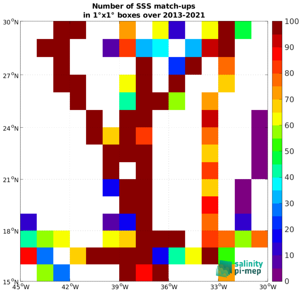
Figure 5: Number of SSS match-ups between TSG (GOSUD-Sailing-ship) SSS and the CCI SSS L4 Merged-OI v4.41 - 7-day running (ESA) SSS product for the SPURS 1 Pi-MEP region over 1^\circ \times 1^\circ boxes and for the full satellite product period.
