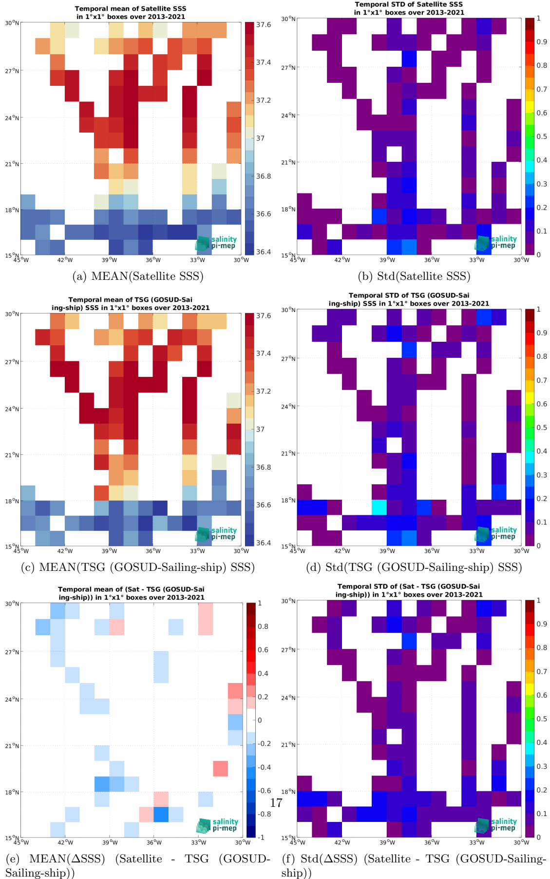
Figure 7: Temporal mean (left) and Std (right) of SSS from CCI SSS L4 Merged-OI v4.41 - 7-day running (ESA) (top), TSG (GOSUD-Sailing-ship) (middle), and of \Delta SSS (Satellite - TSG (GOSUD-Sailing-ship)). Only match-up pairs are used to generate these maps.
