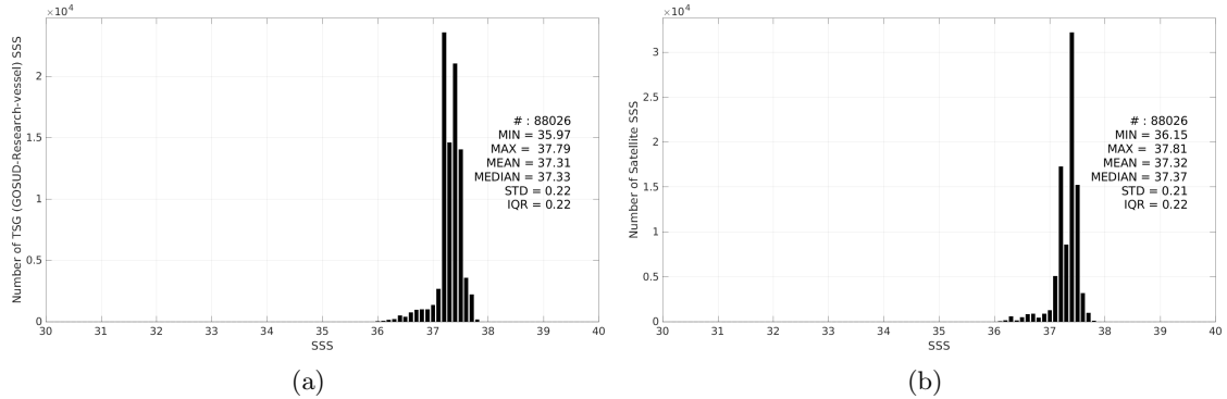
Figure 3: Histograms of SSS from TSG (GOSUD-Research-vessel) (a) and CCI SSS L4 Merged-OI v4.41 - 7-day running (ESA) (b) considering all match-up pairs per bins of 0.1 over the SPURS 1 Pi-MEP region and for the full satellite product period.
