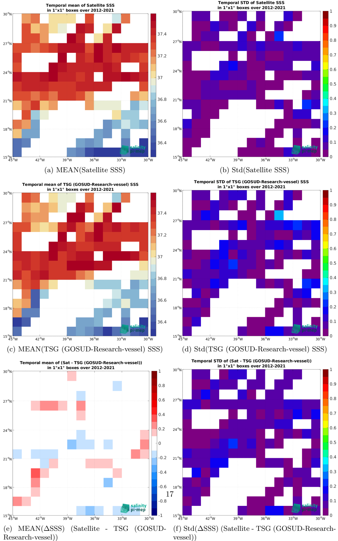
Figure 7: Temporal mean (left) and Std (right) of SSS from CCI SSS L4 Merged-OI v4.41 - 7-day running (ESA) (top), TSG (GOSUD-Research-vessel) (middle), and of \Delta SSS (Satellite - TSG (GOSUD-Research-vessel)). Only match-up pairs are used to generate these maps.
