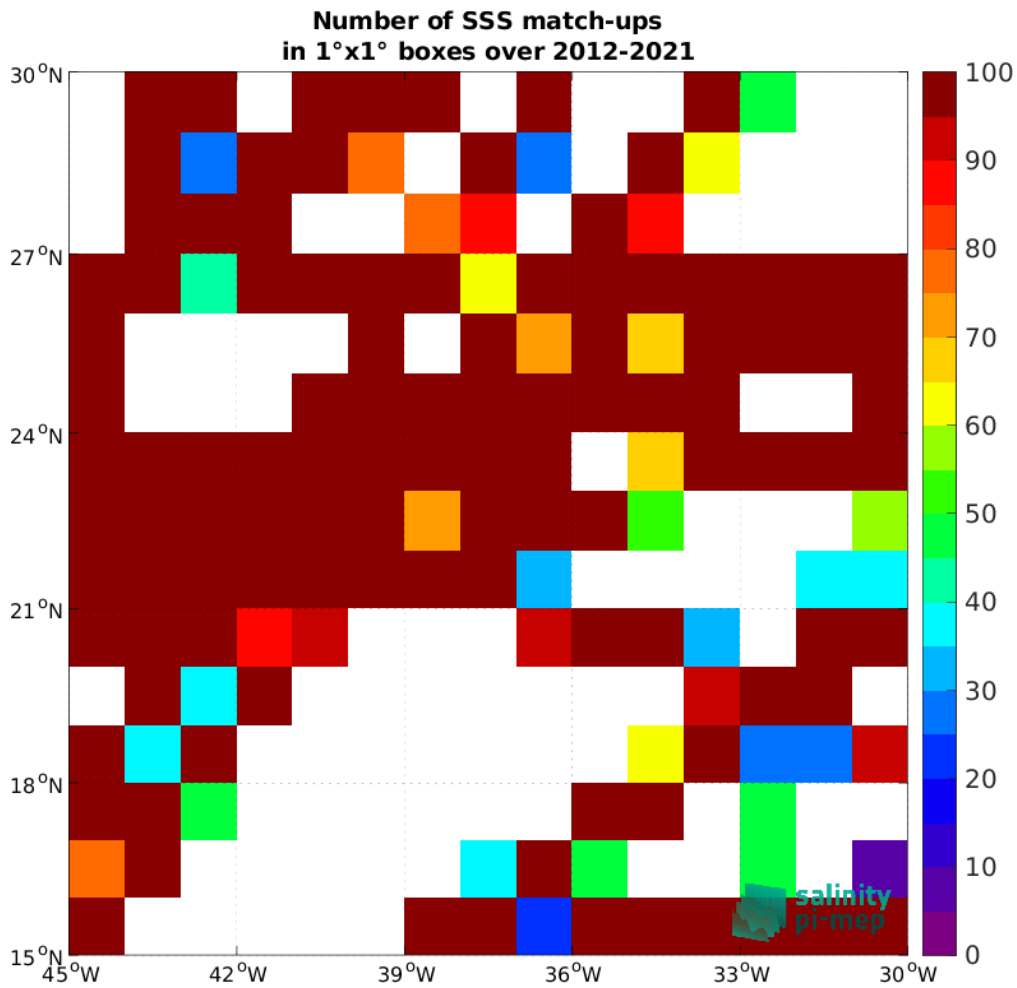
Figure 5: Number of SSS match-ups between TSG (GOSUD-Research-vessel) SSS and the CCI SSS L4 Merged-OI v4.41 - 7-day running (ESA) SSS product for the SPURS 1 Pi-MEP region over 1°x1° boxes and for the full satellite product period.
