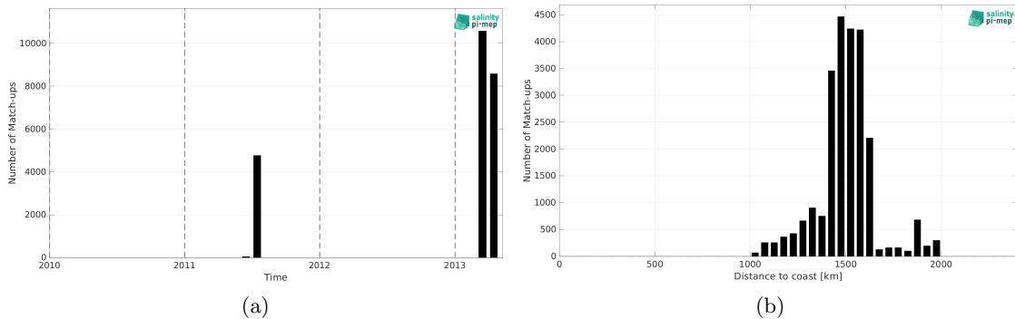
Figure 2: Number of match-ups between TSG (CSIC-UTM) and CCI SSS L4 Merged-OI v4.41 - 7-day running (ESA) SSS as a function of time (a) and as function of the distance to coast (b) over the SPURS 1 Pi-MEP region and for the full satellite product period.
