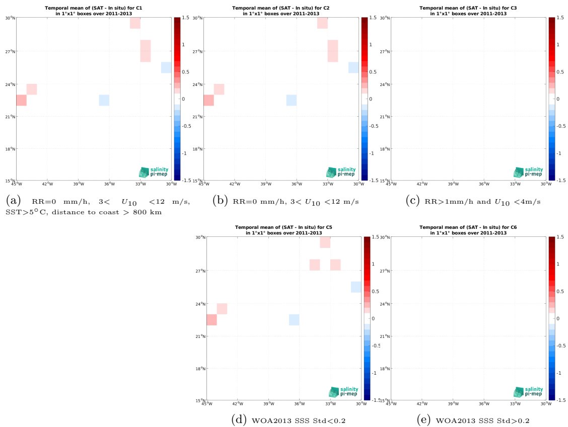
Figure 14: Temporal mean gridded over spatial boxes of size 1^\circ \times 1^\circ of \Delta SSS (CCI SSS L4 Merged-OI v4.41 - 7-day running (ESA) - TSG (CSIC-UTM)) for 5 different subdatasets corresponding to:RR=0 mm/h, 3 < U_{10} < 12 m/s, SST >5^\circ C, distance to coast > 800 km (a), RR=0 mm/h, 3 < U_{10} < 12 m/s (b), RR >1 mm/h and U_{10} < 4 m/s (c), WOA2013 SSS Std <0.2 (d), WOA2013 SSS Std >0.2 (e).
