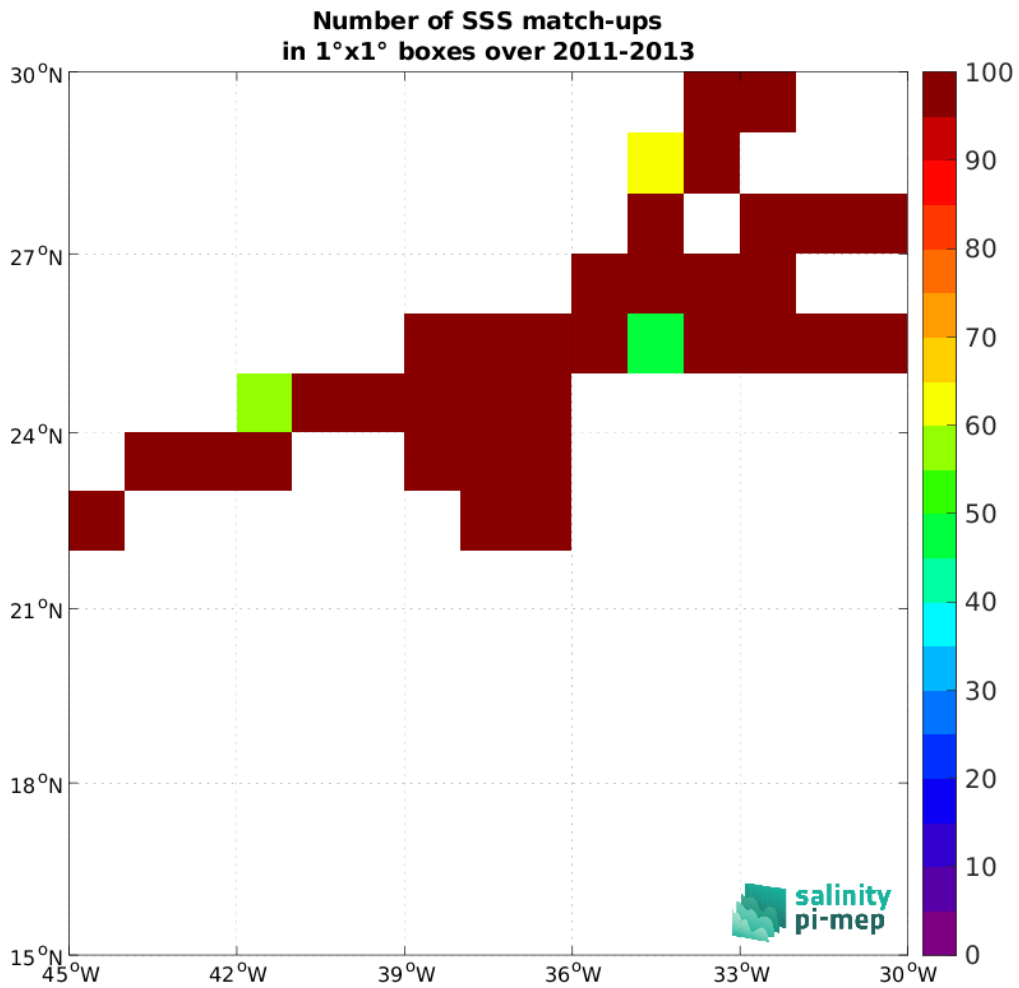
Figure 5: Number of SSS match-ups between TSG (CSIC-UTM) SSS and the CCI SSS L4 Merged-OI v4.41 - 7-day running (ESA) SSS product for the SPURS 1 Pi-MEP region over 1^\circ \times 1^\circ boxes and for the full satellite product period.
