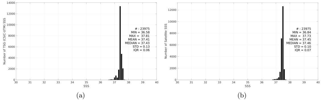
Figure 3: Histograms of SSS from TSG (CSIC-UTM) (a) and CCI SSS L4 Merged-OI v4.41 - 7-day running (ESA) (b) considering all match-up pairs per bins of 0.1 over the SPURS 1 Pi-MEP region and for the full satellite product period.
