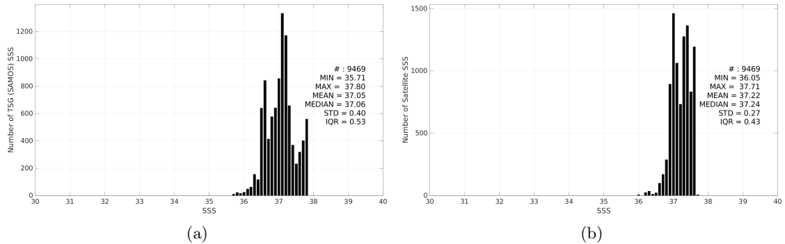
Figure 3: Histograms of SSS from TSG (SAMOS) (a) and CCI SSS L4 Merged-OI v4.41 - 30-day running (ESA) (b) considering all match-up pairs per bins of 0.1 over the SPURS 1 Pi-MEP region and for the full satellite product period.
