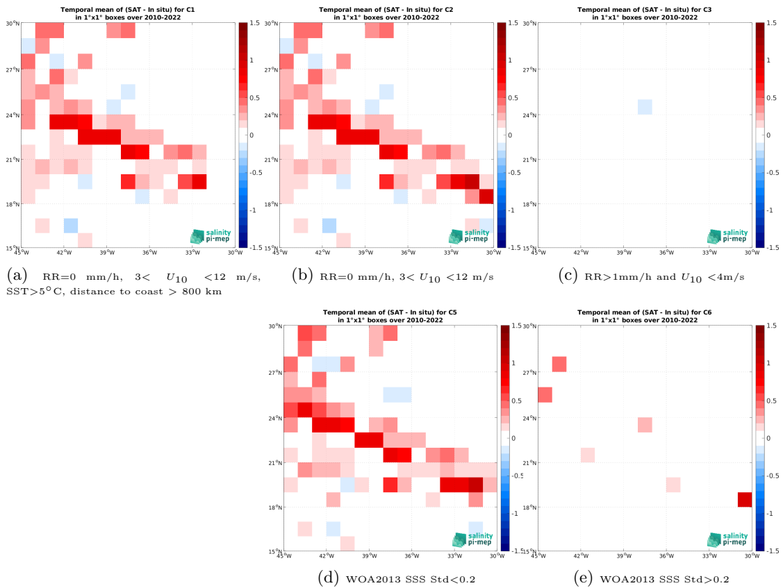
Figure 14: Temporal mean gridded over spatial boxes of size 1^\circ \times 1^\circ of \Delta SSS (CCI SSS L4 Merged-OI v4.41 - 30-day running (ESA) - TSG (SAMOS)) for 5 different subdatasets corresponding to:RR=0 mm/h, 3 < U_{10} < 12 m/s, SST >5^\circ C, distance to coast > 800 km (a), RR=0 mm/h, 3 < U_{10} < 12 m/s (b), RR >1 mm/h and U_{10} < 4 m/s (c), WOA2013 SSS Std <0.2 (d), WOA2013 SSS Std >0.2 (e).
