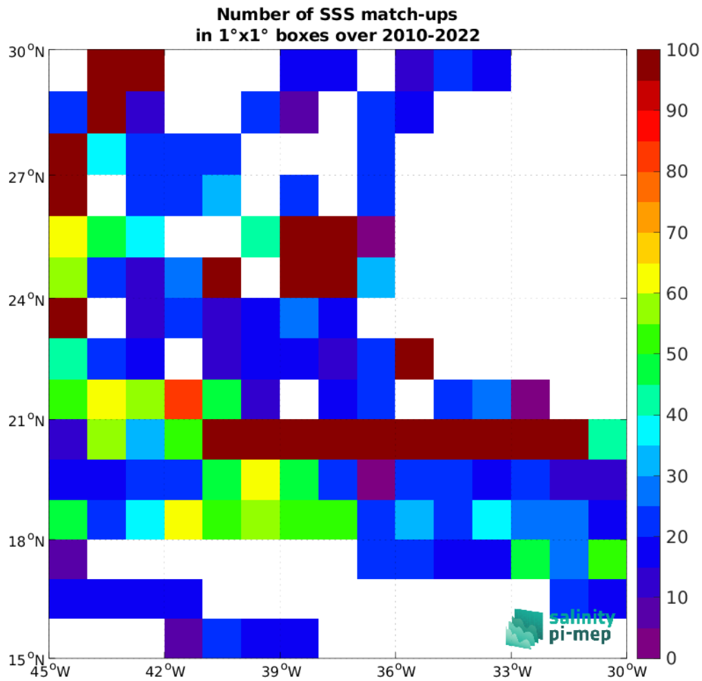
Figure 5: Number of SSS match-ups between TSG (SAMOS) SSS and the CCI SSS L4 Merged-OI v4.41 - 30-day running (ESA) SSS product for the SPURS 1 Pi-MEP region over 1^\circ \times 1^\circ boxes and for the full satellite product period.
