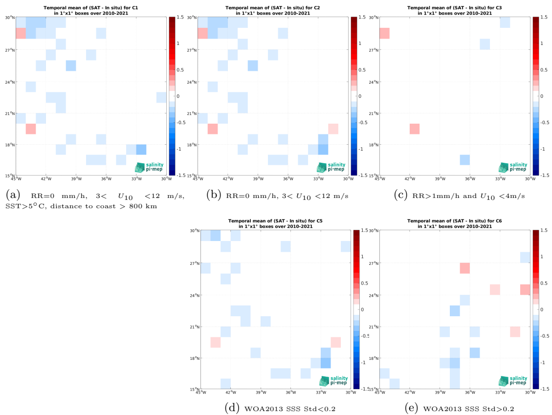
Figure 14: Temporal mean gridded over spatial boxes of size 1^\circ \times 1^\circ of \Delta SSS (CCI SSS L4 Merged-OI v4.41 - 30-day running (ESA) - TSG (LEGOS-DM)) for 5 different subdatasets corresponding to:RR=0 mm/h, 3 < U_{10} < 12 m/s, SST >5^\circ C, distance to coast > 800 km (a), RR=0 mm/h, 3 < U_{10} < 12 m/s (b), RR >1 mm/h and U_{10} < 4 m/s (c), WOA2013 SSS Std <0.2 (d), WOA2013 SSS Std >0.2 (e).
