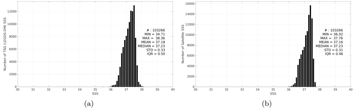
Figure 3: Histograms of SSS from TSG (LEGOS-DM) (a) and CCI SSS L4 Merged-OI v4.41 - 30-day running (ESA) (b) considering all match-up pairs per bins of 0.1 over the SPURS 1 Pi-MEP region and for the full satellite product period.
