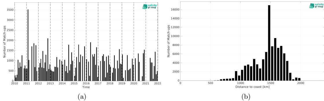
Figure 2: Number of match-ups between TSG (LEGOS-DM) and CCI SSS L4 Merged-OI v4.41 - 30-day running (ESA) SSS as a function of time (a) and as function of the distance to coast (b) over the SPURS 1 Pi-MEP region and for the full satellite product period.
