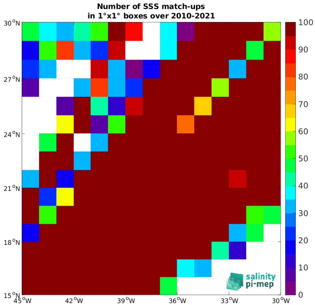
Figure 5: Number of SSS match-ups between TSG (LEGOS-DM) SSS and the CCI SSS L4 Merged-OI v4.41 - 30-day running (ESA) SSS product for the SPURS 1 Pi-MEP region over 1^\circ \times 1^\circ boxes and for the full satellite product period.
