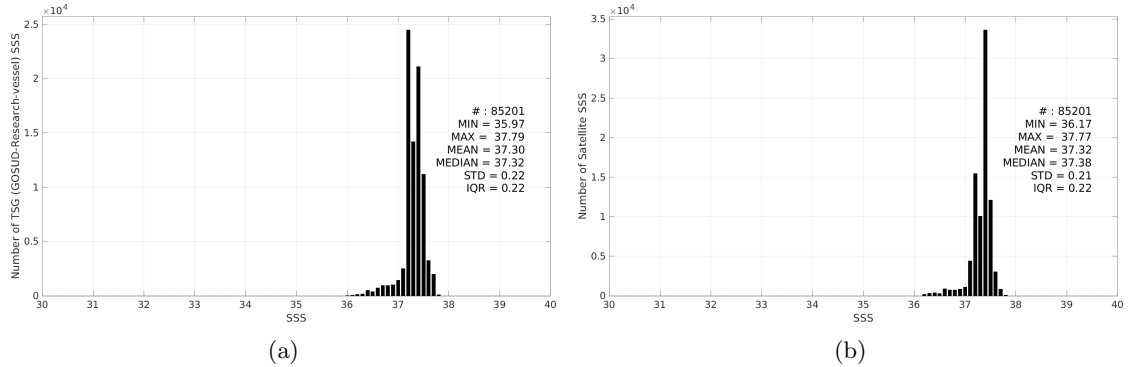
Figure 3: Histograms of SSS from TSG (GOSUD-Research-vessel) (a) and CCI SSS L4 Merged-OI v4.41 - 30-day running (ESA) (b) considering all match-up pairs per bins of 0.1 over the SPURS 1 Pi-MEP region and for the full satellite product period.
