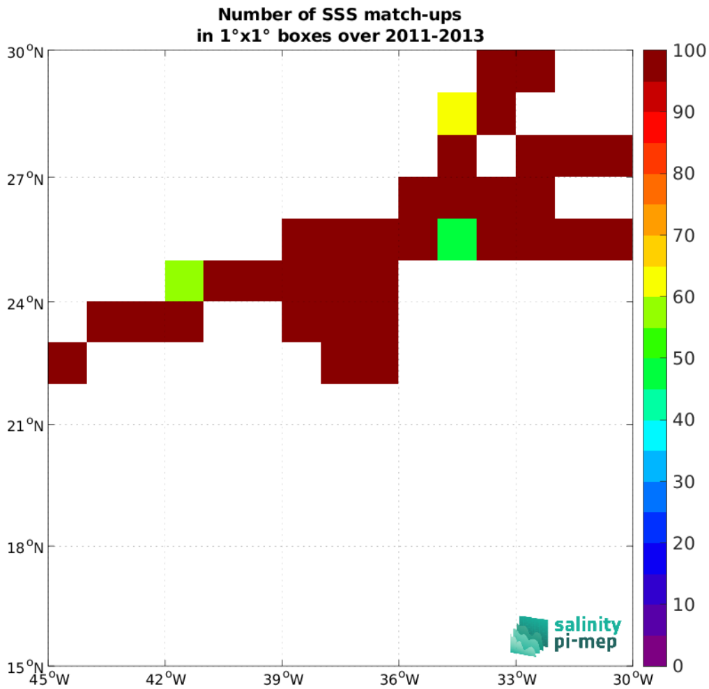
Figure 5: Number of SSS match-ups between TSG (CSIC-UTM) SSS and the CCI SSS L4 Merged-OI v4.41 - 30-day running (ESA) SSS product for the SPURS 1 Pi-MEP region over 1^\circ \times 1^\circ boxes and for the full satellite product period.
