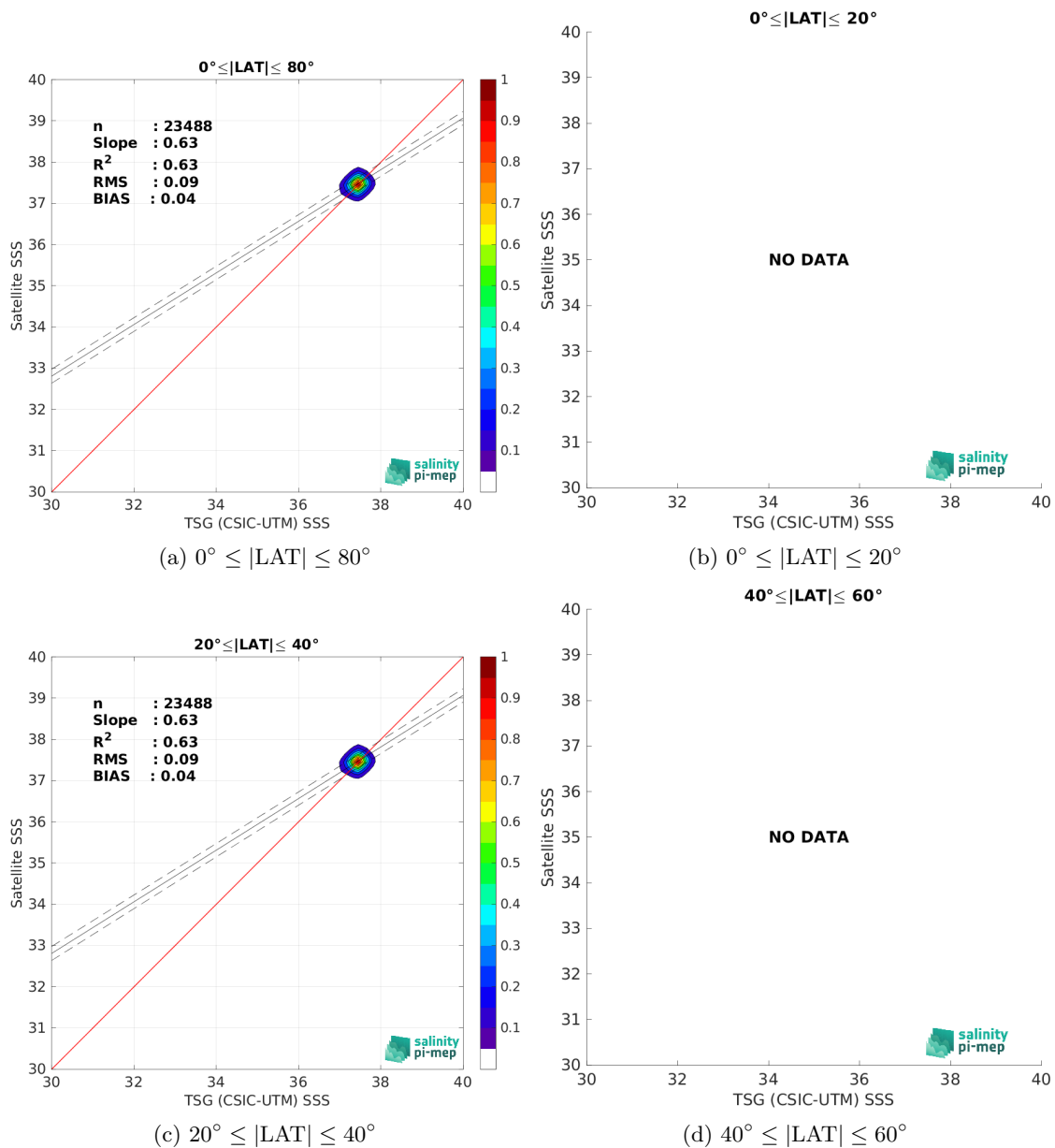
Figure 10: Contour maps of the concentration of CCI SSS L4 Merged-OI v4.41 - 30-day running (ESA) SSS (y-axis) versus TSG (CSIC-UTM) SSS (x-axis) at match-up pairs for different latitude bands. For each plot, the red line shows x=y . The black thin and dashed lines indicate a linear fit through the data cloud and the \pm 95\% confidence levels, respectively. The number match-up pairs n , the slope and R^2 coefficient of the linear fit, the root mean square (RMS) and the mean bias between satellite and in situ data are indicated for each latitude band in each plot.
