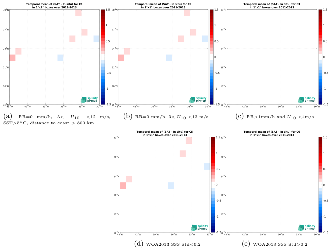
Figure 14: Temporal mean gridded over spatial boxes of size 1^\circ \times 1^\circ of \Delta SSS (CCI SSS L4 Merged-OI v4.41 - 30-day running (ESA) - TSG (CSIC-UTM)) for 5 different subdatasets corresponding to: RR=0 mm/h, 3 < U_{10} < 12 m/s, SST > 5^\circ C , distance to coast > 800 km (a), RR=0 mm/h, 3 < U_{10} < 12 m/s (b), RR > 1 mm/h and U_{10} < 4 m/s (c), WOA2013 SSS Std < 0.2 (d), WOA2013 SSS Std > 0.2 (e).
