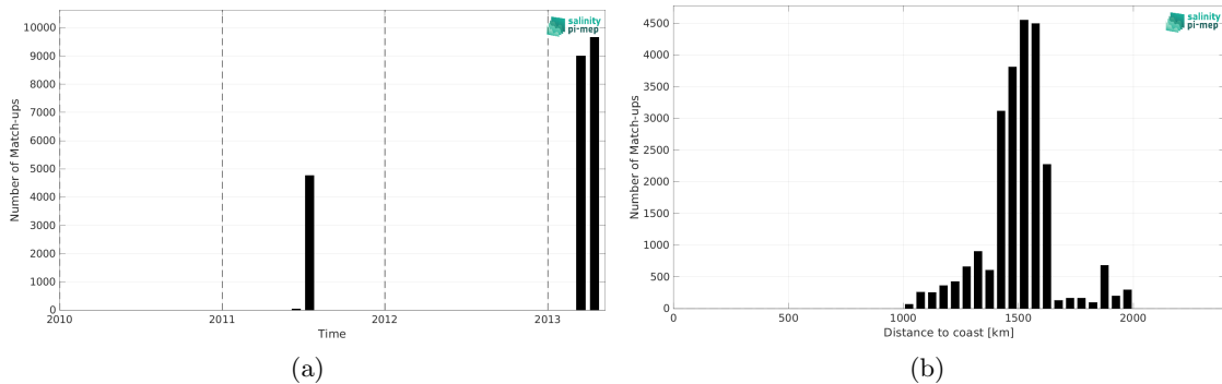
Figure 2: Number of match-ups between TSG (CSIC-UTM) and CCI SSS L4 Merged-OI v4.41 - 30-day running (ESA) SSS as a function of time (a) and as function of the distance to coast (b) over the SPURS 1 Pi-MEP region and for the full satellite product period.
