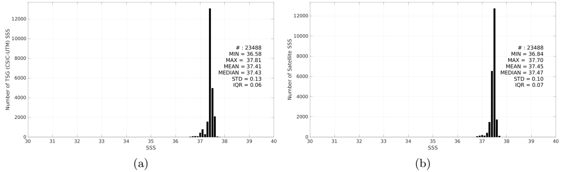
Figure 3: Histograms of SSS from TSG (CSIC-UTM) (a) and CCI SSS L4 Merged-OI v4.41 - 30-day running (ESA) (b) considering all match-up pairs per bins of 0.1 over the SPURS 1 Pi-MEP region and for the full satellite product period.
