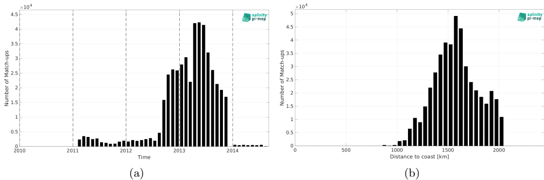
Figure 2: Number of match-ups between Surface drifters and CCI SSS L4 Merged-OI v4.41 - 30-day running (ESA) SSS as a function of time (a) and as function of the distance to coast (b) over the SPURS 1 Pi-MEP region and for the full satellite product period.
