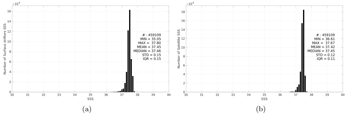
Figure 3: Histograms of SSS from Surface drifters (a) and CCI SSS L4 Merged-OI v4.41 - 30-day running (ESA) (b) considering all match-up pairs per bins of 0.1 over the SPURS 1 Pi-MEP region and for the full satellite product period.
