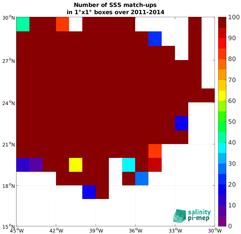
Figure 4: Number of SSS match-ups between Surface drifters SSS and the CCI SSS L4 Merged-OI v4.41 - 30-day running (ESA) SSS product for the SPURS 1 Pi-MEP region over 1°x1° boxes and for the full satellite product period.
