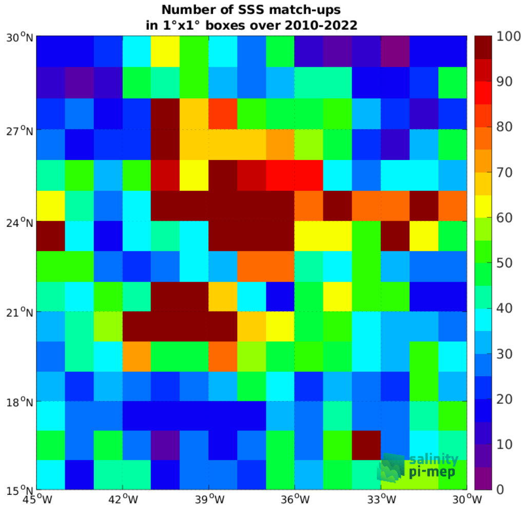
Figure 5: Number of SSS match-ups between Argo SSS and the CCI SSS L4 Merged-OI v4.41 - 30-day running (ESA) SSS product for the SPURS 1 Pi-MEP region over 1^\circ \times 1^\circ boxes and for the full satellite product period.
