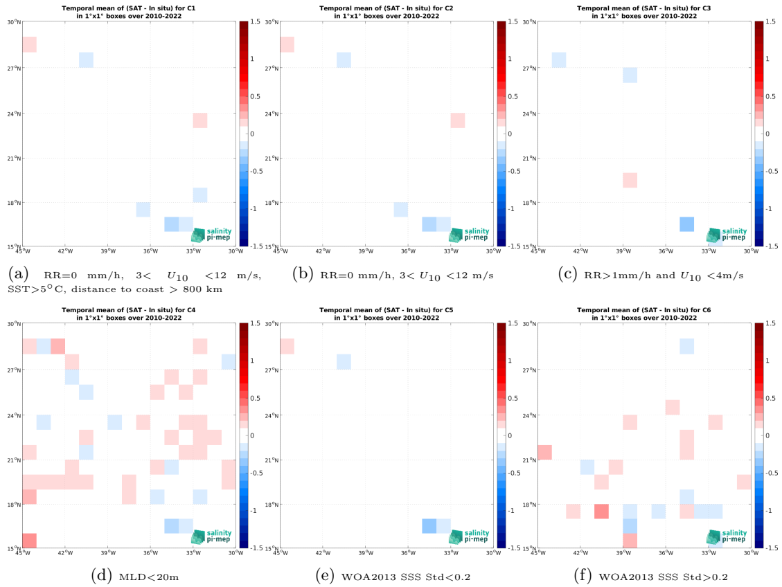
Figure 14: Temporal mean gridded over spatial boxes of size 1^\circ \times 1^\circ of \Delta SSS (CCI SSS L4 Merged-OI v4.41 - 30-day running (ESA) - Argo) for 6 different subdatasets corresponding to:RR=0 mm/h, 3 < U_{10} < 12 m/s, SST >5^\circ C, distance to coast > 800 km (a), RR=0 mm/h, 3 < U_{10} < 12 m/s (b), RR >1 mm/h and U_{10} < 4 m/s (c),MLD <20 m (d),WOA2013 SSS Std <0.2 (e),WOA2013 SSS Std >0.2 (f).
