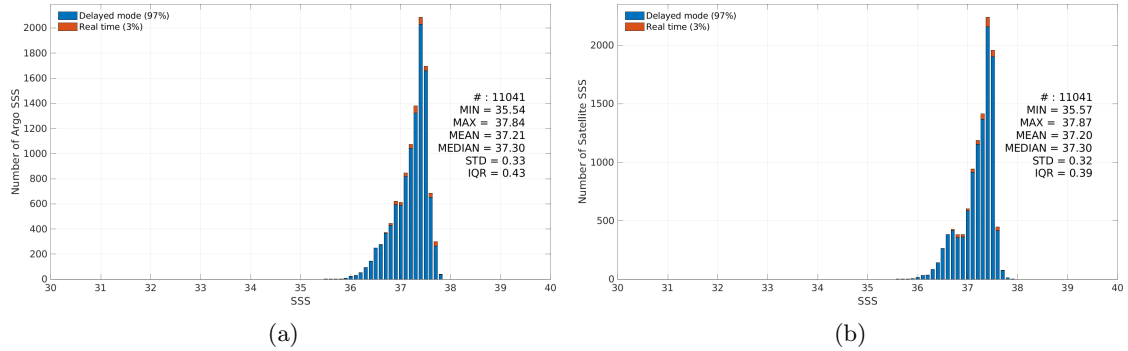
Figure 3: Histograms of SSS from Argo (a) and CCI SSS L4 Merged-OI v4.41 - 30-day running (ESA) (b) considering all match-up pairs per bins of 0.1 over the SPURS 1 Pi-MEP region and for the full satellite product period.
