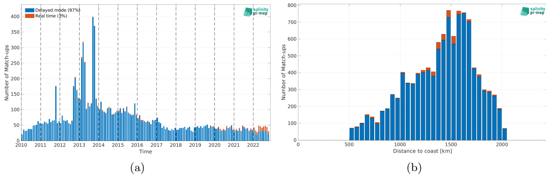
Figure 2: Number of match-ups between Argo and CCI SSS L4 Merged-OI v4.41 - 30-day running (ESA) SSS as a function of time (a) and as function of the distance to coast (b) over the SPURS 1 Pi-MEP region and for the full satellite product period.
