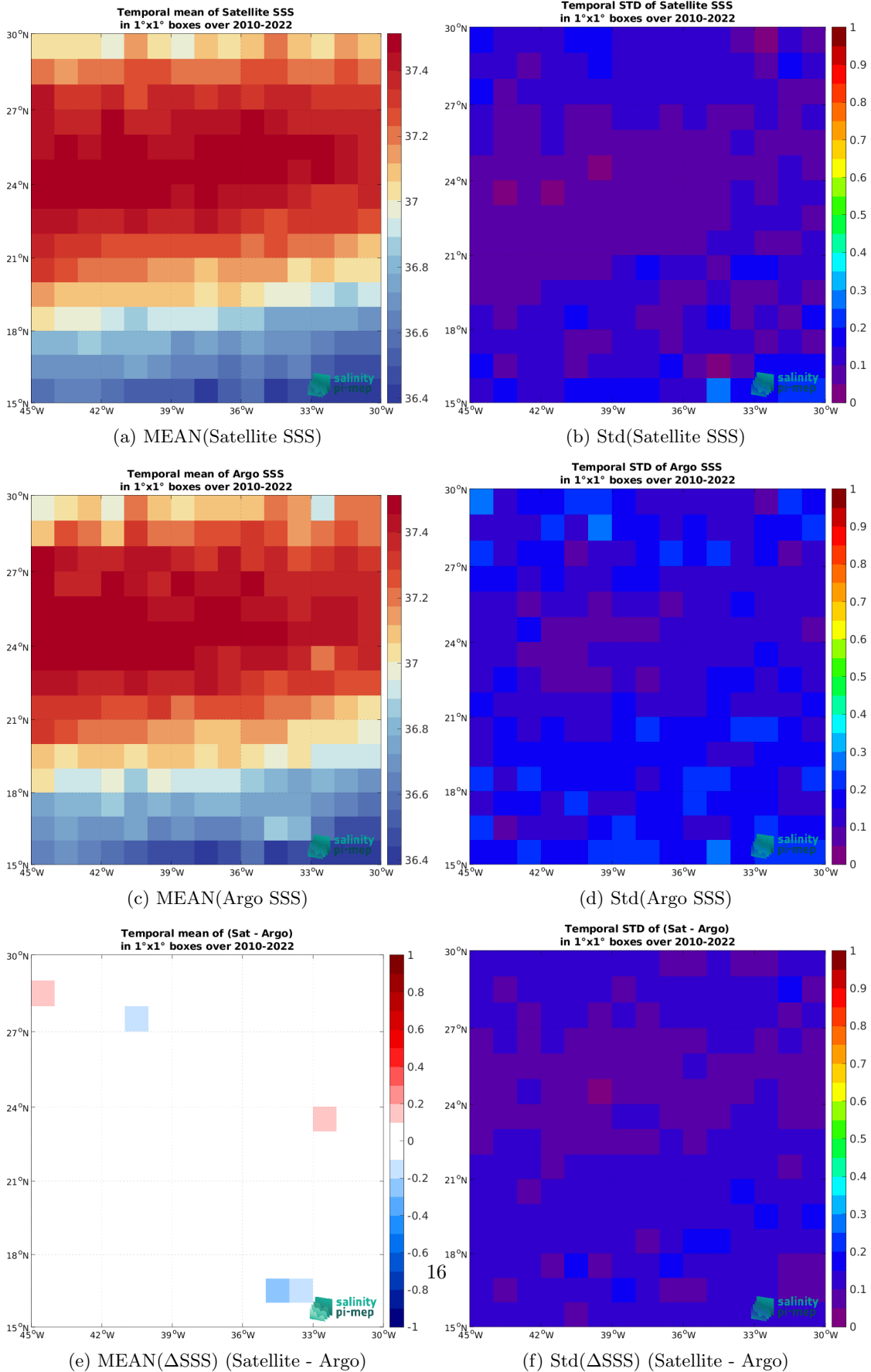
Figure 7: Temporal mean (left) and Std (right) of SSS from CCI SSS L4 Merged-OI v4.41 - 30-day running (ESA) (top), Argo (middle), and of \Delta SSS (Satellite - Argo). Only match-up pairs are used to generate these maps.
