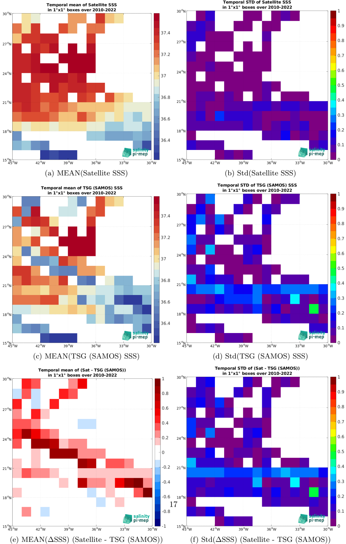
Figure 6: Temporal mean (left) and Std (right) of SSS from CCI SSS L4 Merged-OI v4.4 - 7-day running (ESA) (top), TSG (SAMOS) (middle), and of \Delta SSS (Satellite - TSG (SAMOS)). Only match-up pairs are used to generate these maps.
