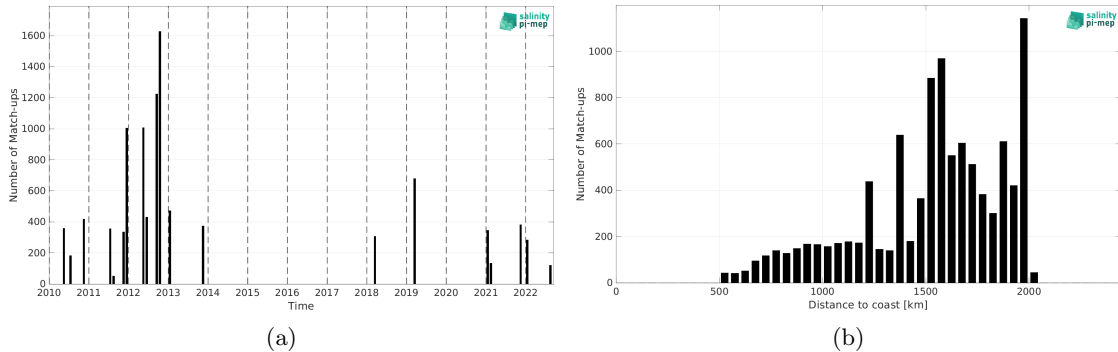
Figure 1: Number of match-ups between TSG (SAMOS) and CCI SSS L4 Merged-OI v4.4 - 7-day running (ESA) SSS as a function of time (a) and as function of the distance to coast (b) over the SPURS 1 Pi-MEP region and for the full satellite product period.
