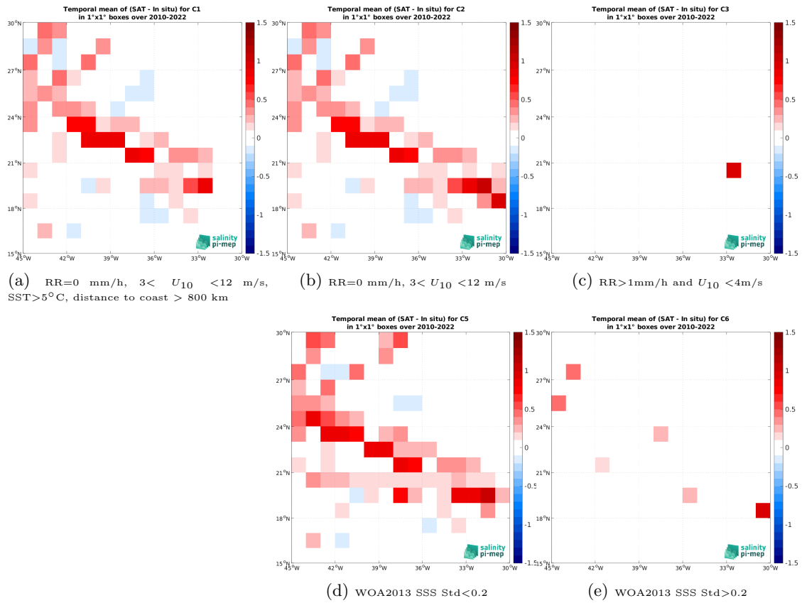
Figure 12: Temporal mean gridded over spatial boxes of size 1^\circ \times 1^\circ of \Delta SSS (CCI SSS L4 Merged-OI v4.4 - 7-day running (ESA) - TSG (SAMOS)) for 5 different subdatasets corresponding to:RR=0 mm/h, 3 < U_{10} < 12 m/s, SST >5^\circ C, distance to coast > 800 km (a), RR=0 mm/h, 3 < U_{10} < 12 m/s (b), RR >1 mm/h and U_{10} < 4 m/s (c), WOA2013 SSS Std <0.2 (d), WOA2013 SSS Std >0.2 (e).
