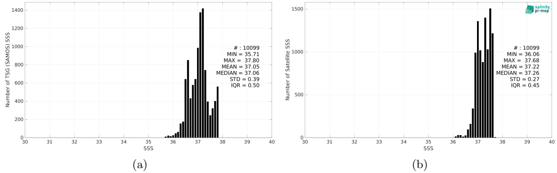
Figure 2: Histograms of SSS from TSG (SAMOS) (a) and CCI SSS L4 Merged-OI v4.4 - 7-day running (ESA) (b) considering all match-up pairs per bins of 0.1 over the SPURS 1 Pi-MEP region and for the full satellite product period.
