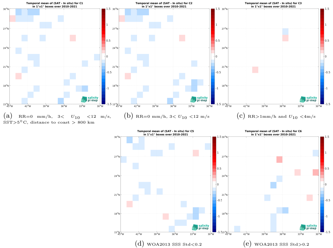
Figure 12: Temporal mean gridded over spatial boxes of size 1^{\circ}\times 1^{\circ} of \Delta\text{SSS} (CCI SSS L4 Merged-OI v4.4 - 7-day running (ESA) - TSG (LEGOS-DM)) for 5 different subdatasets corresponding to:RR=0 mm/h, 3 < U_{10} < 12 m/s, SST >5^{\circ}\text{C} , distance to coast > 800 km (a), RR=0 mm/h, 3 < U_{10} < 12 m/s (b), RR >1 mm/h and U_{10} < 4 m/s (c), WOA2013 SSS Std <0.2 (d), WOA2013 SSS Std >0.2 (e).
