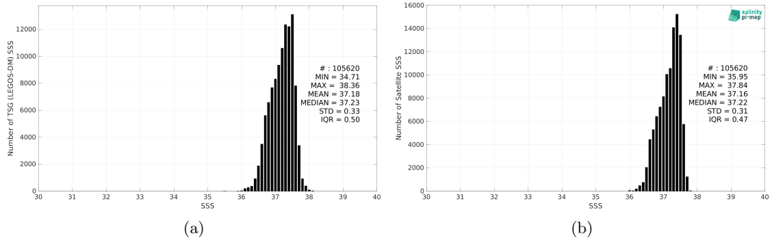
Figure 2: Histograms of SSS from TSG (LEGOS-DM) (a) and CCI SSS L4 Merged-OI v4.4 - 7-day running (ESA) (b) considering all match-up pairs per bins of 0.1 over the SPURS 1 Pi-MEP region and for the full satellite product period.
