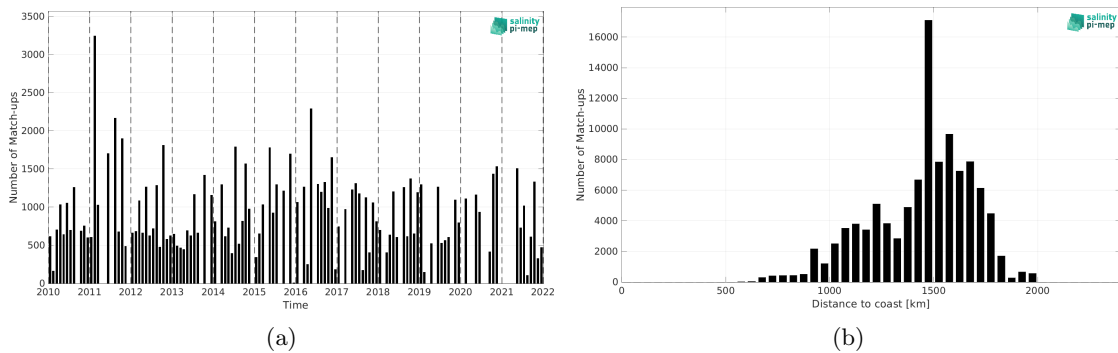
Figure 1: Number of match-ups between TSG (LEGOS-DM) and CCI SSS L4 Merged-OI v4.4 - 7-day running (ESA) SSS as a function of time (a) and as function of the distance to coast (b) over the SPURS 1 Pi-MEP region and for the full satellite product period.
