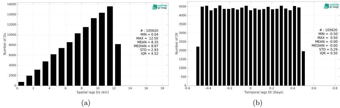
Figure 5: Histograms of the spatial (a) and temporal (b) lags between the location/time of the TSG (LEGOS-DM) measurement and the date of the corresponding CCI SSS L4 Merged-OI v4.4 - 7-day running (ESA) SSS pixel.
