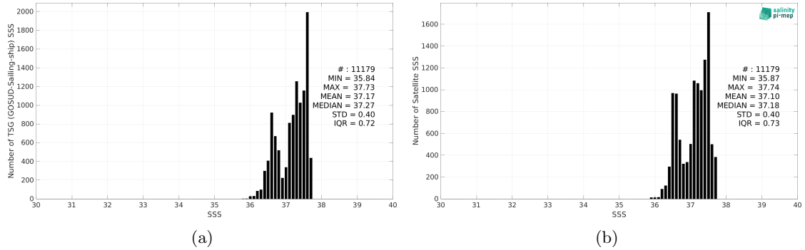
Figure 2: Histograms of SSS from TSG (GOSUD-Sailing-ship) (a) and CCI SSS L4 Merged-OI v4.4 - 7-day running (ESA) (b) considering all match-up pairs per bins of 0.1 over the SPURS 1 Pi-MEP region and for the full satellite product period.
