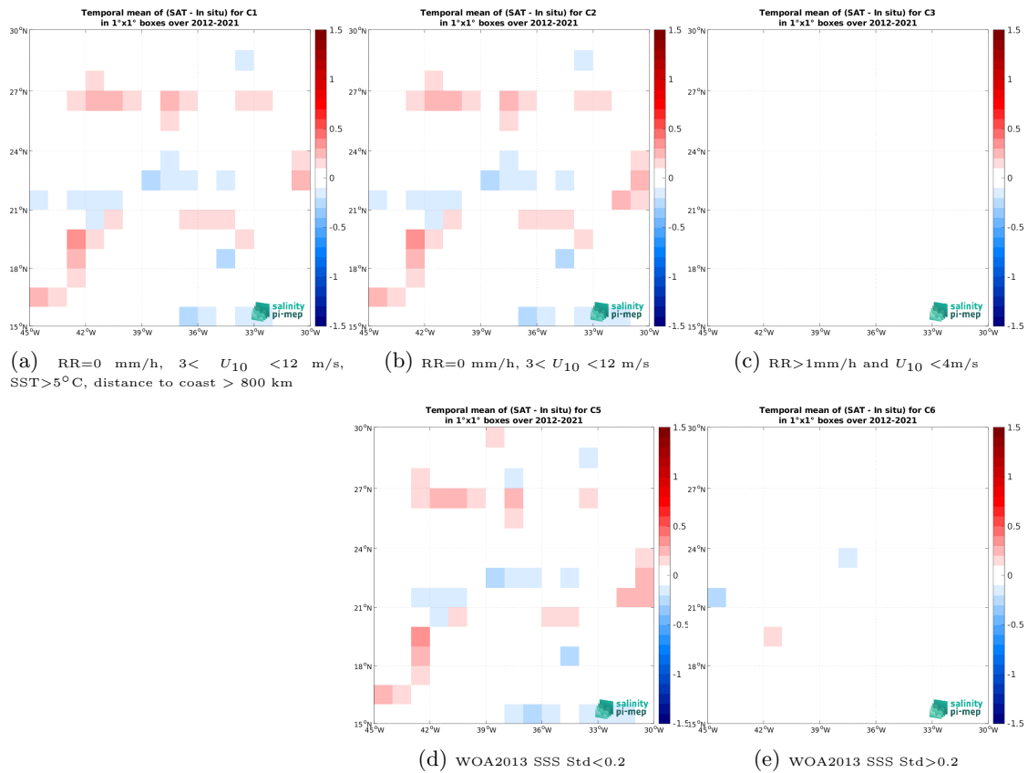
Figure 12: Temporal mean gridded over spatial boxes of size 1^\circ \times 1^\circ of \Delta SSS (CCI SSS L4 Merged-OI v4.4 - 7-day running (ESA) - TSG (GOSUD-Research-vessel)) for 5 different subdatasets corresponding to: RR=0 mm/h, 3 < U_{10} < 12 m/s, SST > 5°C, distance to coast > 800 km (a), RR=0 mm/h, 3 < U_{10} < 12 m/s (b), RR > 1mm/h and U_{10} < 4 m/s (c), WOA2013 SSS Std < 0.2 (d), WOA2013 SSS Std > 0.2 (e).
