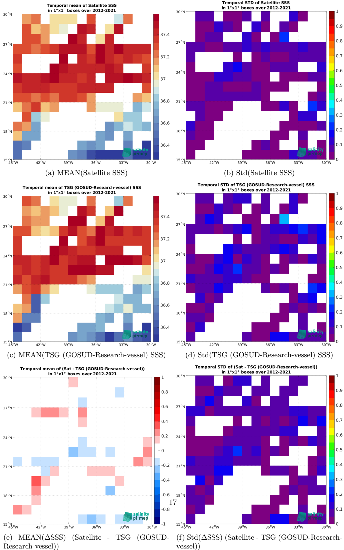
Figure 6: Temporal mean (left) and Std (right) of SSS from CCI SSS L4 Merged-OI v4.4 - 7-day running (ESA) (top), TSG (GOSUD-Research-vessel) (middle), and of \Delta SSS (Satellite - TSG (GOSUD-Research-vessel)). Only match-up pairs are used to generate these maps.
