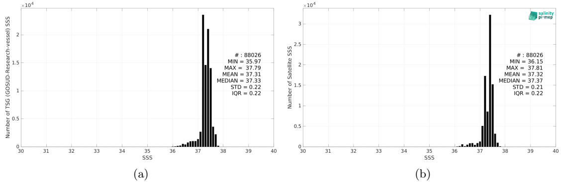
Figure 2: Histograms of SSS from TSG (GOSUD-Research-vessel) (a) and CCI SSS L4 Merged-OI v4.4 - 7-day running (ESA) (b) considering all match-up pairs per bins of 0.1 over the SPURS 1 Pi-MEP region and for the full satellite product period.
