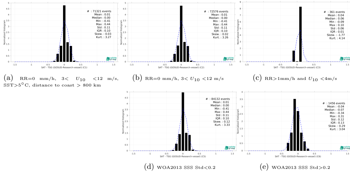
Figure 13: Normalized histogram of \Delta\text{SSS} (CCI SSS L4 Merged-OI v4.4 - 7-day running (ESA) - TSG (GOSUD-Research-vessel)) for 5 different subdatasets corresponding to: RR=0 mm/h, 3 < U_{10} < 12 m/s, SST > 5^{\circ}\text{C} , distance to coast > 800 km (a), RR=0 mm/h, 3 < U_{10} < 12 m/s (b), RR > 1\text{mm/h} and U_{10} < 4\text{m/s} (c), WOA2013 SSS Std < 0.2 (d), WOA2013 SSS Std > 0.2 (e).
