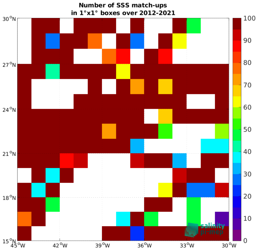
Figure 4: Number of SSS match-ups between TSG (GOSUD-Research-vessel) SSS and the CCI SSS L4 Merged-OI v4.4 - 7-day running (ESA) SSS product for the SPURS 1 Pi-MEP region over 1°x1° boxes and for the full satellite product period.
