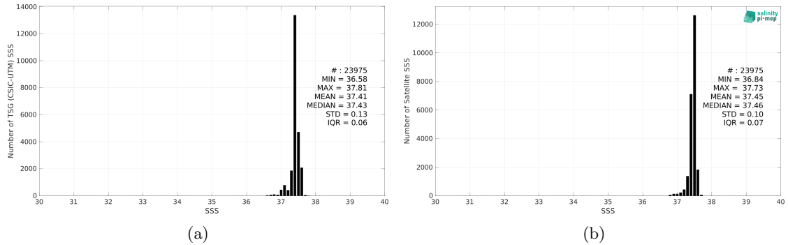
Figure 2: Histograms of SSS from TSG (CSIC-UTM) (a) and CCI SSS L4 Merged-OI v4.4 - 7-day running (ESA) (b) considering all match-up pairs per bins of 0.1 over the SPURS 1 Pi-MEP region and for the full satellite product period.
