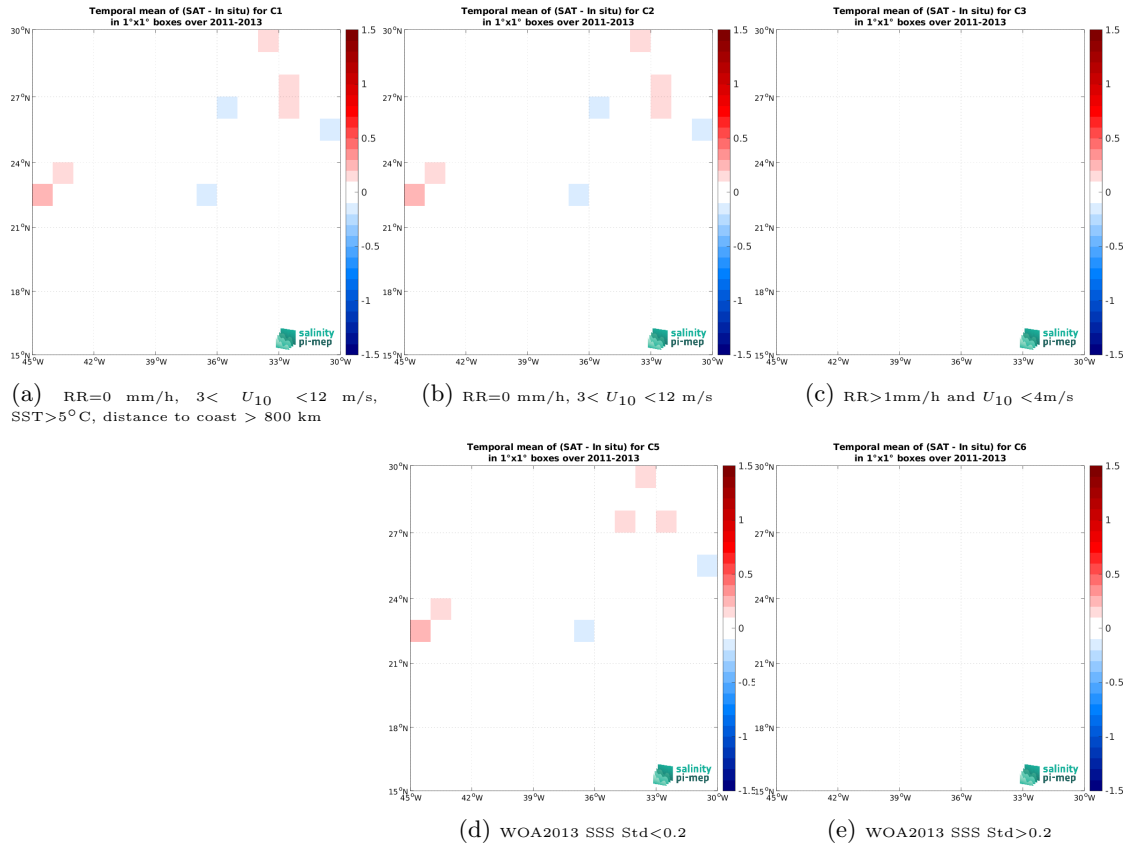
Figure 12: Temporal mean gridded over spatial boxes of size 1^{\circ}\times 1^{\circ} of \Delta\text{SSS} (CCI SSS L4 Merged-OI v4.4 - 7-day running (ESA) - TSG (CSIC-UTM)) for 5 different subdatasets corresponding to:RR=0 mm/h, 3 < U_{10} < 12 m/s, SST >5^{\circ}\text{C} , distance to coast > 800 km (a), RR=0 mm/h, 3 < U_{10} < 12 m/s (b), RR >1 mm/h and U_{10} < 4 m/s (c), WOA2013 SSS Std <0.2 (d), WOA2013 SSS Std >0.2 (e).
