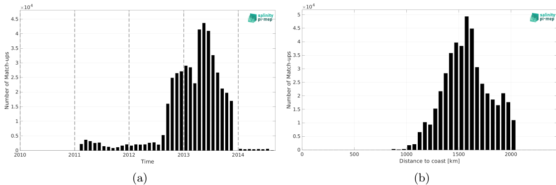
Figure 1: Number of match-ups between Surface drifters and CCI SSS L4 Merged-OI v4.4 - 7-day running (ESA) SSS as a function of time (a) and as function of the distance to coast (b) over the SPURS 1 Pi-MEP region and for the full satellite product period.
