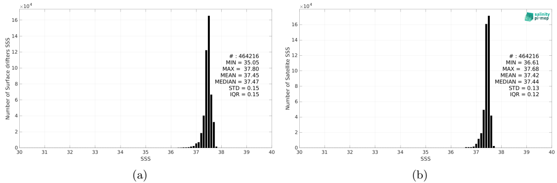
Figure 2: Histograms of SSS from Surface drifters (a) and CCI SSS L4 Merged-OI v4.4 - 7-day running (ESA) (b) considering all match-up pairs per bins of 0.1 over the SPURS 1 Pi-MEP region and for the full satellite product period.
