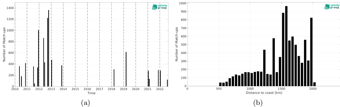
Figure 1: Number of match-ups between TSG (SAMOS) and CCI SSS L4 Merged-OI v4.4 - 30-day running (ESA) SSS as a function of time (a) and as function of the distance to coast (b) over the SPURS 1 Pi-MEP region and for the full satellite product period.
