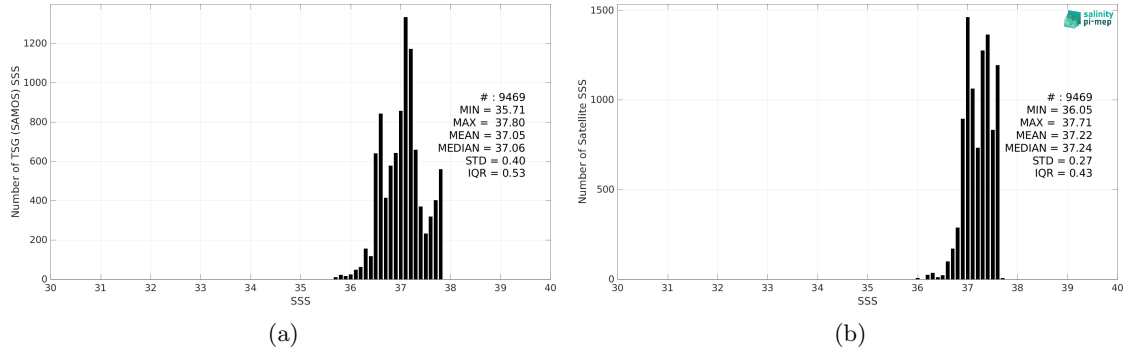
Figure 2: Histograms of SSS from TSG (SAMOS) (a) and CCI SSS L4 Merged-OI v4.4 - 30-day running (ESA) (b) considering all match-up pairs per bins of 0.1 over the SPURS 1 Pi-MEP region and for the full satellite product period.
