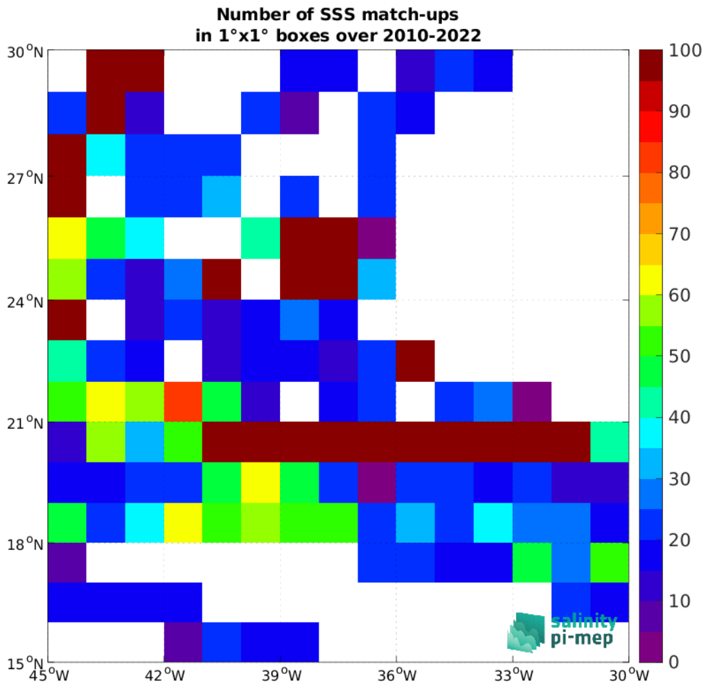
Figure 4: Number of SSS match-ups between TSG (SAMOS) SSS and the CCI SSS L4 Merged-OI v4.4 - 30-day running (ESA) SSS product for the SPURS 1 Pi-MEP region over 1°x1° boxes and for the full satellite product period.
