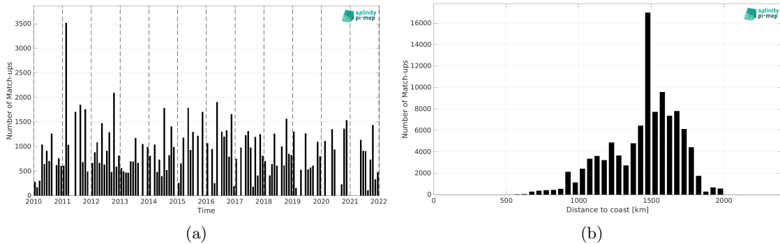
Figure 1: Number of match-ups between TSG (LEGOS-DM) and CCI SSS L4 Merged-OI v4.4 - 30-day running (ESA) SSS as a function of time (a) and as function of the distance to coast (b) over the SPURS 1 Pi-MEP region and for the full satellite product period.
