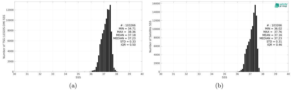
Figure 2: Histograms of SSS from TSG (LEGOS-DM) (a) and CCI SSS L4 Merged-OI v4.4 - 30-day running (ESA) (b) considering all match-up pairs per bins of 0.1 over the SPURS 1 Pi-MEP region and for the full satellite product period.
