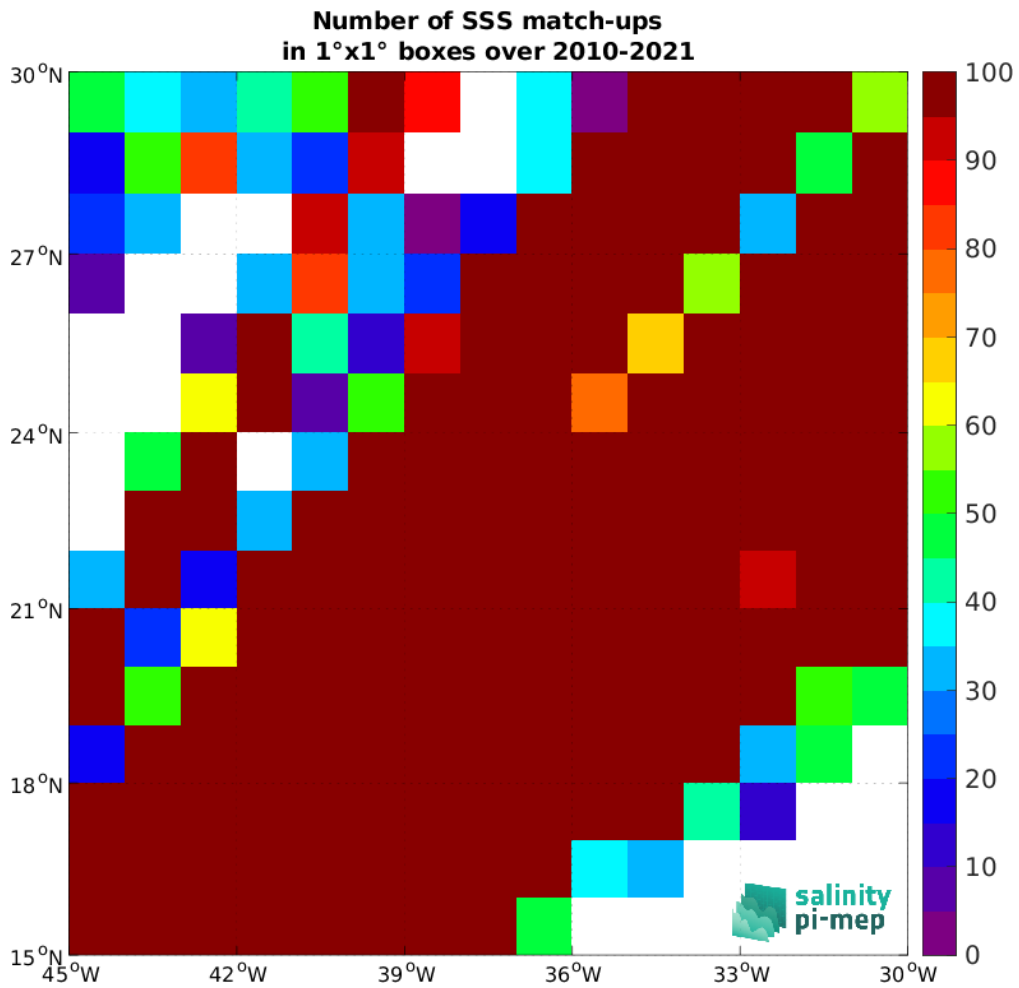
Figure 4: Number of SSS match-ups between TSG (LEGOS-DM) SSS and the CCI SSS L4 Merged-OI v4.4 - 30-day running (ESA) SSS product for the SPURS 1 Pi-MEP region over 1^\circ \times 1^\circ boxes and for the full satellite product period.
