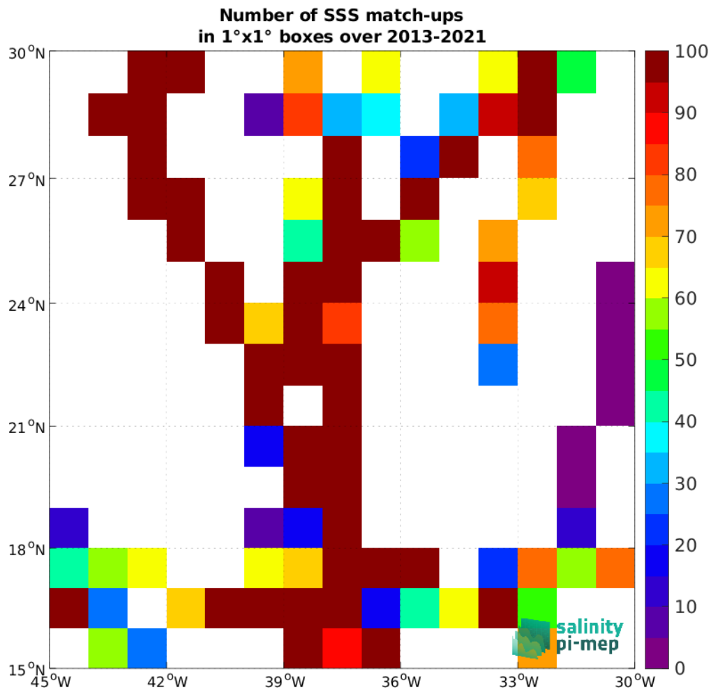
Figure 4: Number of SSS match-ups between TSG (GOSUD-Sailing-ship) SSS and the CCI SSS L4 Merged-OI v4.4 - 30-day running (ESA) SSS product for the SPURS 1 Pi-MEP region over 1^\circ \times 1^\circ boxes and for the full satellite product period.
