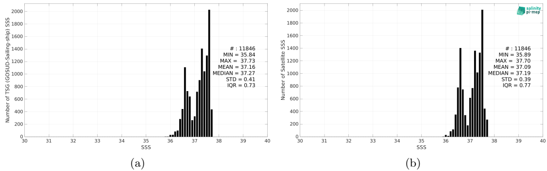
Figure 2: Histograms of SSS from TSG (GOSUD-Sailing-ship) (a) and CCI SSS L4 Merged-OI v4.4 - 30-day running (ESA) (b) considering all match-up pairs per bins of 0.1 over the SPURS 1 Pi-MEP region and for the full satellite product period.
