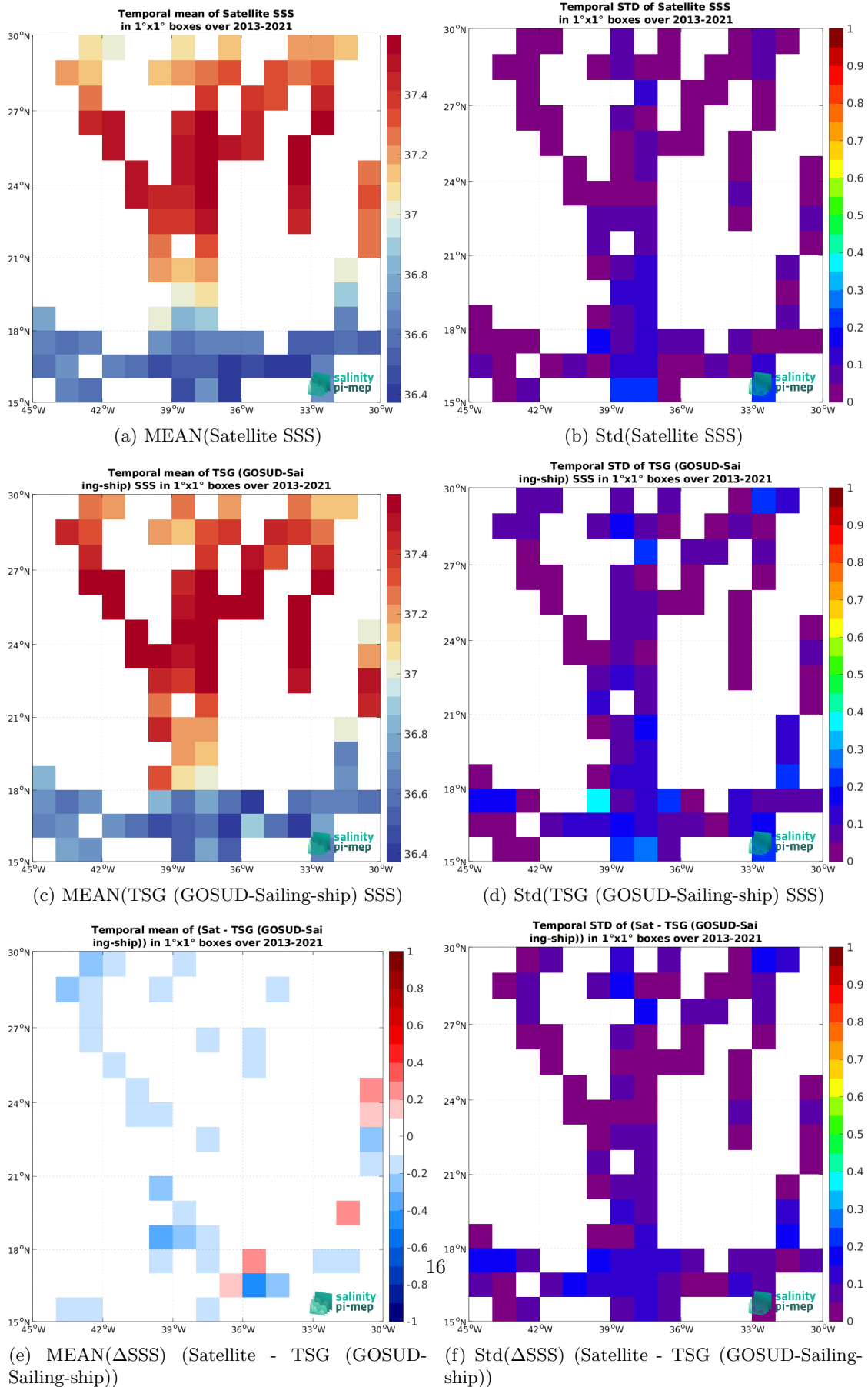
Figure 6: Temporal mean (left) and Std (right) of SSS from CCI SSS L4 Merged-OI v4.4 - 30-day running (ESA) (top), TSG (GOSUD-Sailing-ship) (middle), and of \Delta SSS (Satellite - TSG (GOSUD-Sailing-ship)). Only match-up pairs are used to generate these maps.
