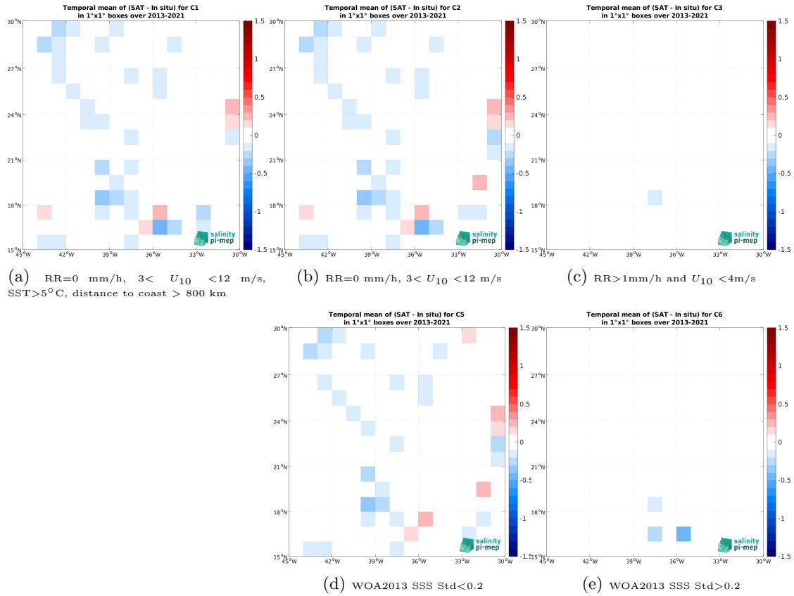
Figure 12: Temporal mean gridded over spatial boxes of size 1^{\circ} \times 1^{\circ} of \Delta\text{SSS} (CCI SSS L4 Merged-OI v4.4 - 30-day running (ESA) - TSG (GOSUD-Sailing-ship)) for 5 different subdatasets corresponding to: RR=0 mm/h, 3 < U_{10} < 12 m/s, SST > 5^{\circ}\text{C} , distance to coast > 800 km (a), RR=0 mm/h, 3 < U_{10} < 12 m/s (b), RR > 1\text{mm/h} and U_{10} < 4\text{m/s} (c), WOA2013 SSS Std < 0.2 (d), WOA2013 SSS Std > 0.2 (e).
