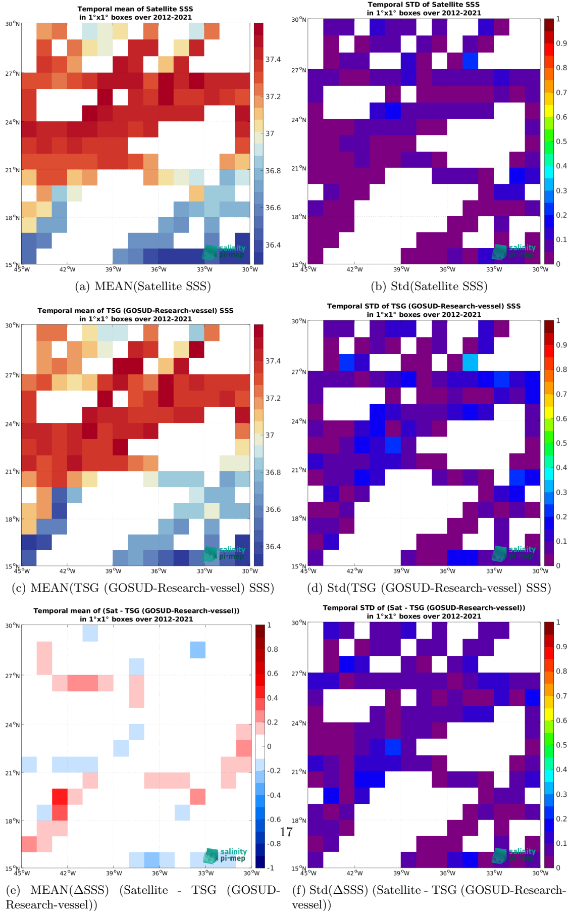
Figure 6: Temporal mean (left) and Std (right) of SSS from CCI SSS L4 Merged-OI v4.4 - 30-day running (ESA) (top), TSG (GOSUD-Research-vessel) (middle), and of \Delta SSS (Satellite - TSG (GOSUD-Research-vessel)). Only match-up pairs are used to generate these maps.
