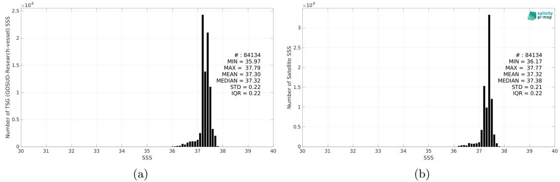
Figure 2: Histograms of SSS from TSG (GOSUD-Research-vessel) (a) and CCI SSS L4 Merged-OI v4.4 - 30-day running (ESA) (b) considering all match-up pairs per bins of 0.1 over the SPURS 1 Pi-MEP region and for the full satellite product period.
