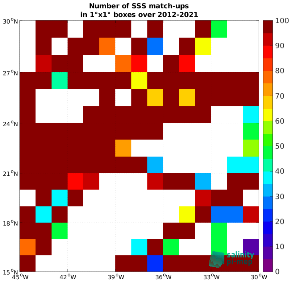
Figure 4: Number of SSS match-ups between TSG (GOSUD-Research-vessel) SSS and the CCI SSS L4 Merged-OI v4.4 - 30-day running (ESA) SSS product for the SPURS 1 Pi-MEP region over 1°x1° boxes and for the full satellite product period.
