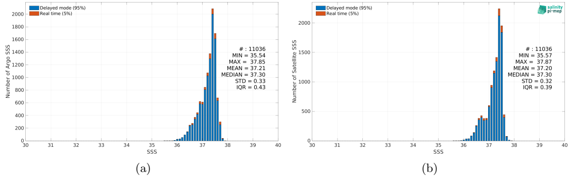
Figure 2: Histograms of SSS from Argo (a) and CCI SSS L4 Merged-OI v4.4 - 30-day running (ESA) (b) considering all match-up pairs per bins of 0.1 over the SPURS 1 Pi-MEP region and for the full satellite product period.
