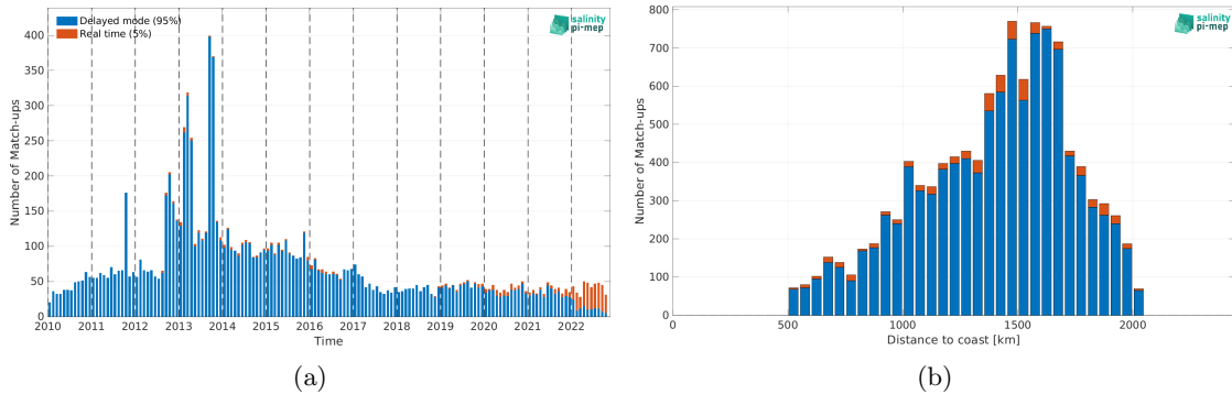
Figure 1: Number of match-ups between Argo and CCI SSS L4 Merged-OI v4.4 - 30-day running (ESA) SSS as a function of time (a) and as function of the distance to coast (b) over the SPURS 1 Pi-MEP region and for the full satellite product period.
