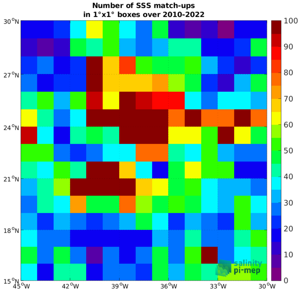
Figure 4: Number of SSS match-ups between Argo SSS and the CCI SSS L4 Merged-OI v4.4 - 30-day running (ESA) SSS product for the SPURS 1 Pi-MEP region over 1^\circ \times 1^\circ boxes and for the full satellite product period.
