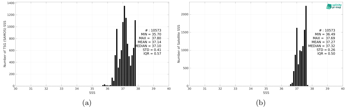
Figure 2: Histograms of SSS from TSG (SAMOS) (a) and CCI SSS L4 Merged-OI v3.2 - 7-day running (ESA) (b) considering all match-up pairs per bins of 0.1 over the SPURS 1 Pi-MEP region and for the full satellite product period.
