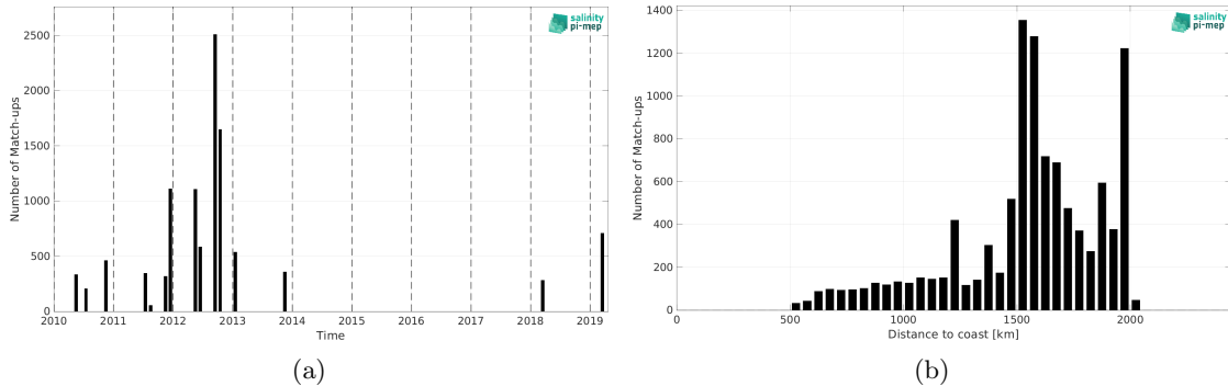
Figure 1: Number of match-ups between TSG (SAMOS) and CCI SSS L4 Merged-OI v3.2 - 7-day running (ESA) SSS as a function of time (a) and as function of the distance to coast (b) over the SPURS 1 Pi-MEP region and for the full satellite product period.
