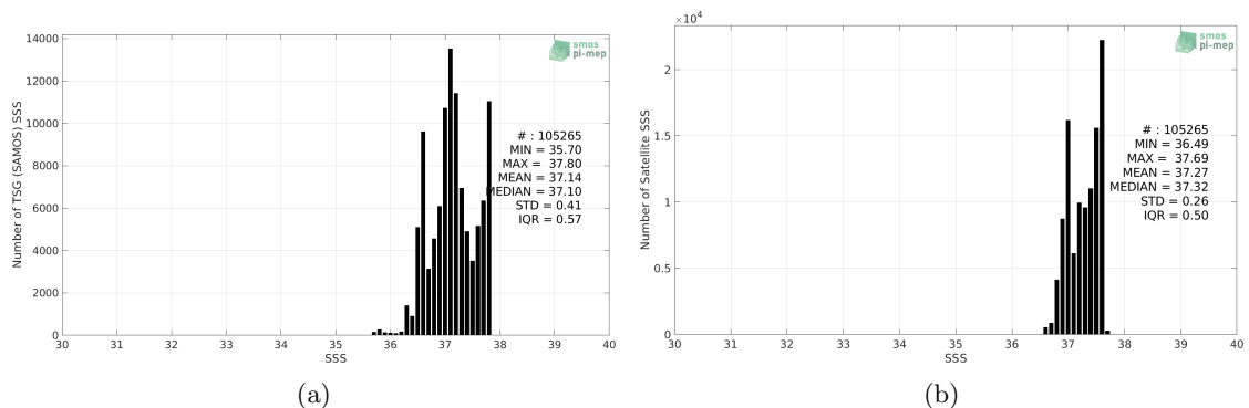
Figure 2: Histograms of SSS from TSG (SAMOS) (a) and CCI SSS L4 Merged-OI v3.2 - 7-day running (ESA) (b) considering all match-up pairs per bins of 0.1 over the SPURS 1 Pi-MEP region and for the full satellite product period.
