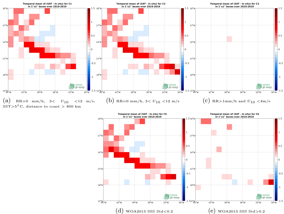
Figure 12: Temporal mean gridded over spatial boxes of size 1^\circ \times 1^\circ of \Delta\text{SSS} (CCI SSS L4 Merged-OI v3.2 - 7-day running (ESA) - TSG (SAMOS)) for 5 different subdatasets corresponding to:RR=0 mm/h, 3 < U_{10} < 12 m/s, SST >5^\circ\text{C} , distance to coast > 800 km (a), RR=0 mm/h, 3 < U_{10} < 12 m/s (b), RR >1 mm/h and U_{10} < 4 m/s (c), WOA2013 SSS Std <0.2 (d), WOA2013 SSS Std >0.2 (e).
