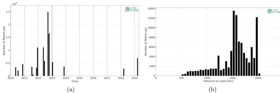
Figure 1: Number of match-ups between TSG (SAMOS) and CCI SSS L4 Merged-OI v3.2 - 7-day running (ESA) SSS as a function of time (a) and as function of the distance to coast (b) over the SPURS 1 Pi-MEP region and for the full satellite product period.
