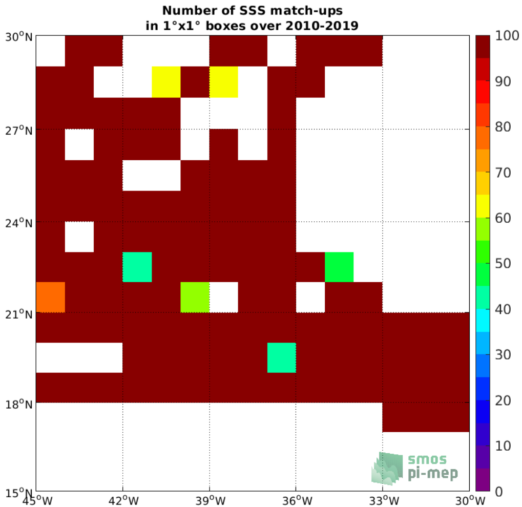
Figure 4: Number of SSS match-ups between TSG (SAMOS) SSS and the CCI SSS L4 Merged-OI v3.2 - 7-day running (ESA) SSS product for the SPURS 1 Pi-MEP region over 1°x1° boxes and for the full satellite product period.
