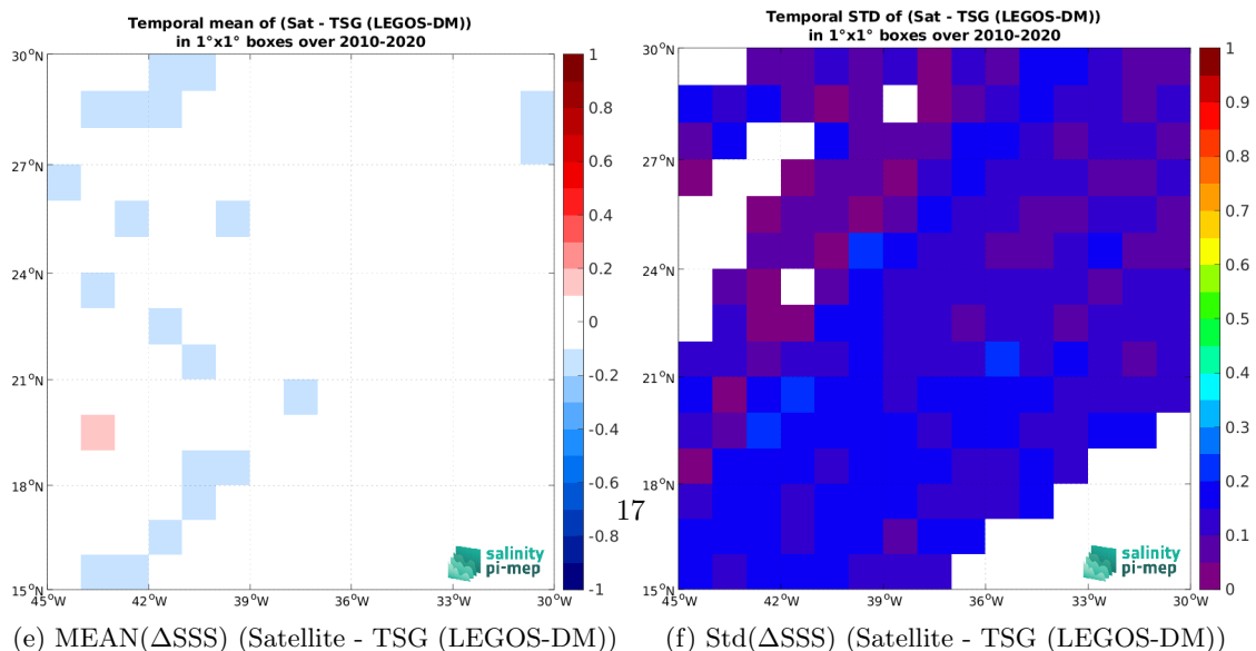
Figure 6: Temporal mean (left) and Std (right) of SSS from CCI SSS L4 Merged-OI v3.2 - 7-day running (ESA) (top), TSG (LEGOS-DM) (middle), and of \Delta SSS (Satellite - TSG (LEGOS-DM)). Only match-up pairs are used to generate these maps.
