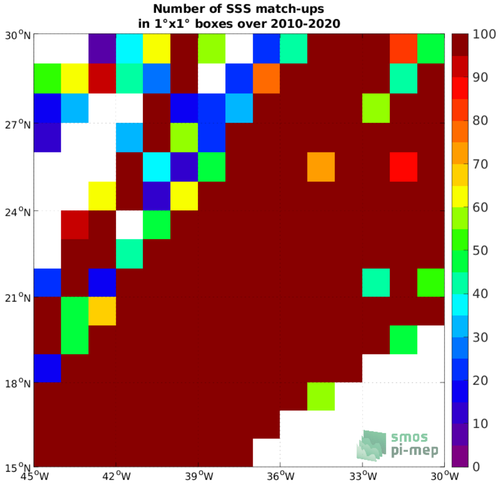
Figure 4: Number of SSS match-ups between TSG (LEGOS-DM) SSS and the CCI SSS L4 Merged-OI v3.2 - 7-day running (ESA) SSS product for the SPURS 1 Pi-MEP region over 1°x1° boxes and for the full satellite product period.
