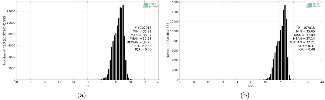
Figure 2: Histograms of SSS from TSG (LEGOS-DM) (a) and CCI SSS L4 Merged-OI v3.2 - 7-day running (ESA) (b) considering all match-up pairs per bins of 0.1 over the SPURS 1 Pi-MEP region and for the full satellite product period.
