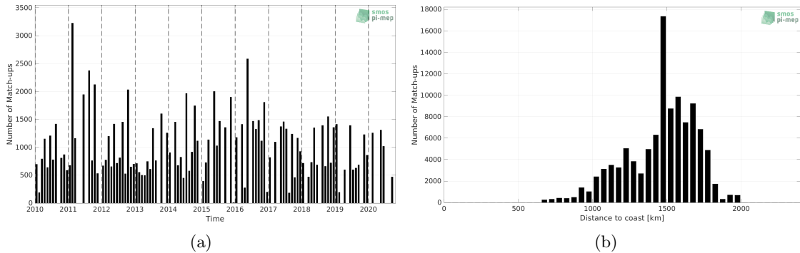
Figure 1: Number of match-ups between TSG (LEGOS-DM) and CCI SSS L4 Merged-OI v3.2 - 7-day running (ESA) SSS as a function of time (a) and as function of the distance to coast (b) over the SPURS 1 Pi-MEP region and for the full satellite product period.
