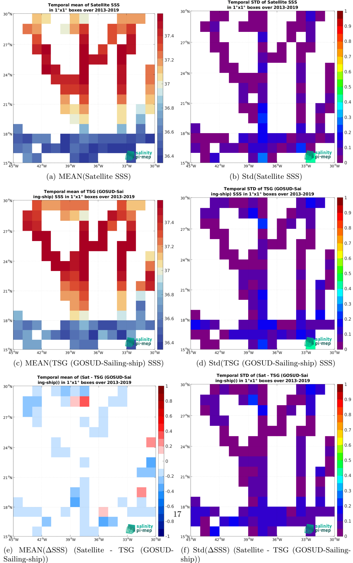
Figure 6: Temporal mean (left) and Std (right) of SSS from CCI SSS L4 Merged-OI v3.2 - 7-day running (ESA) (top), TSG (GOSUD-Sailing-ship) (middle), and of \Delta SSS (Satellite - TSG (GOSUD-Sailing-ship)). Only match-up pairs are used to generate these maps.
